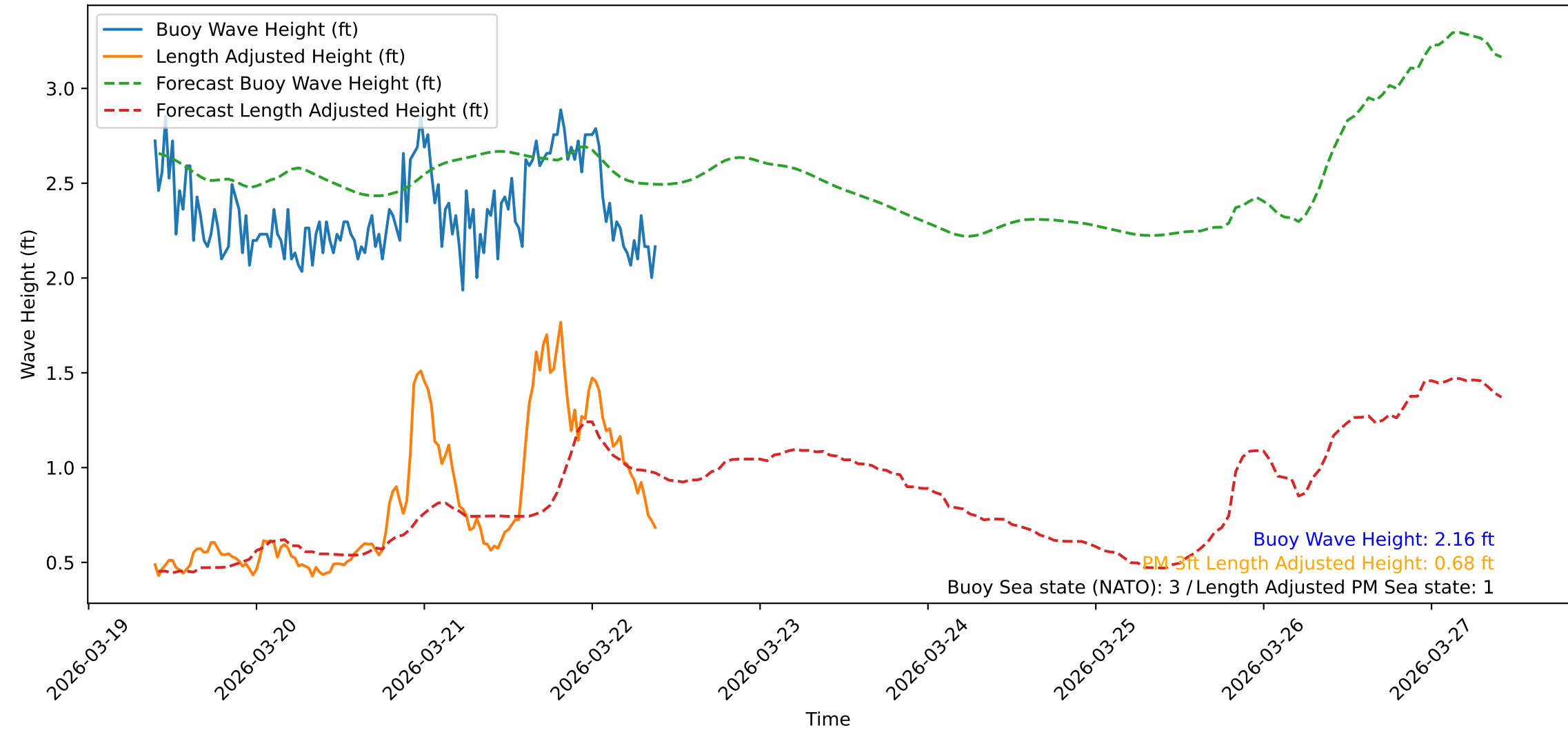
Wave Heights over Time for Green Beach at 2026-03-22 09:41:12
