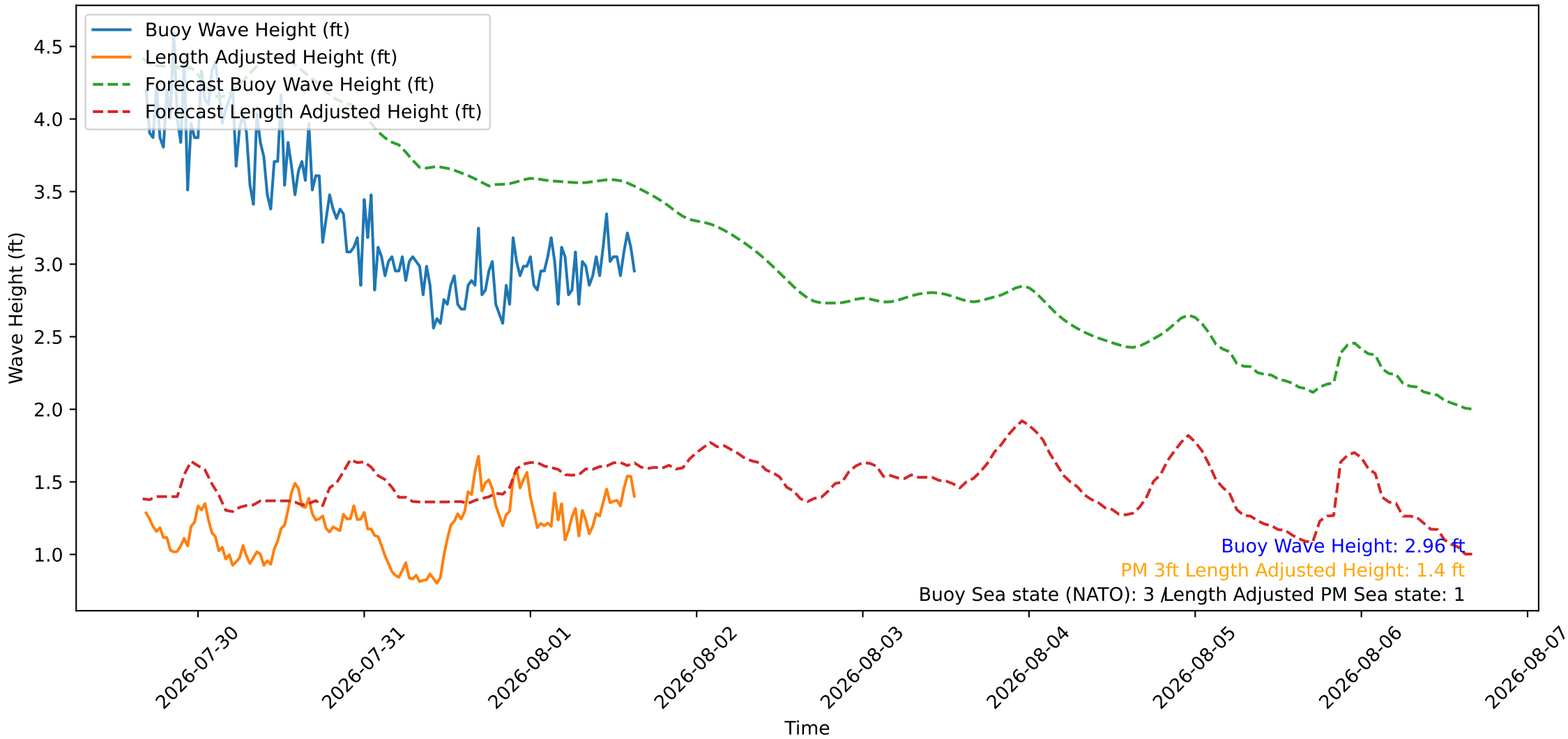
Wave Heights over Time for Red Beach at 2026-08-01 16:00:46
