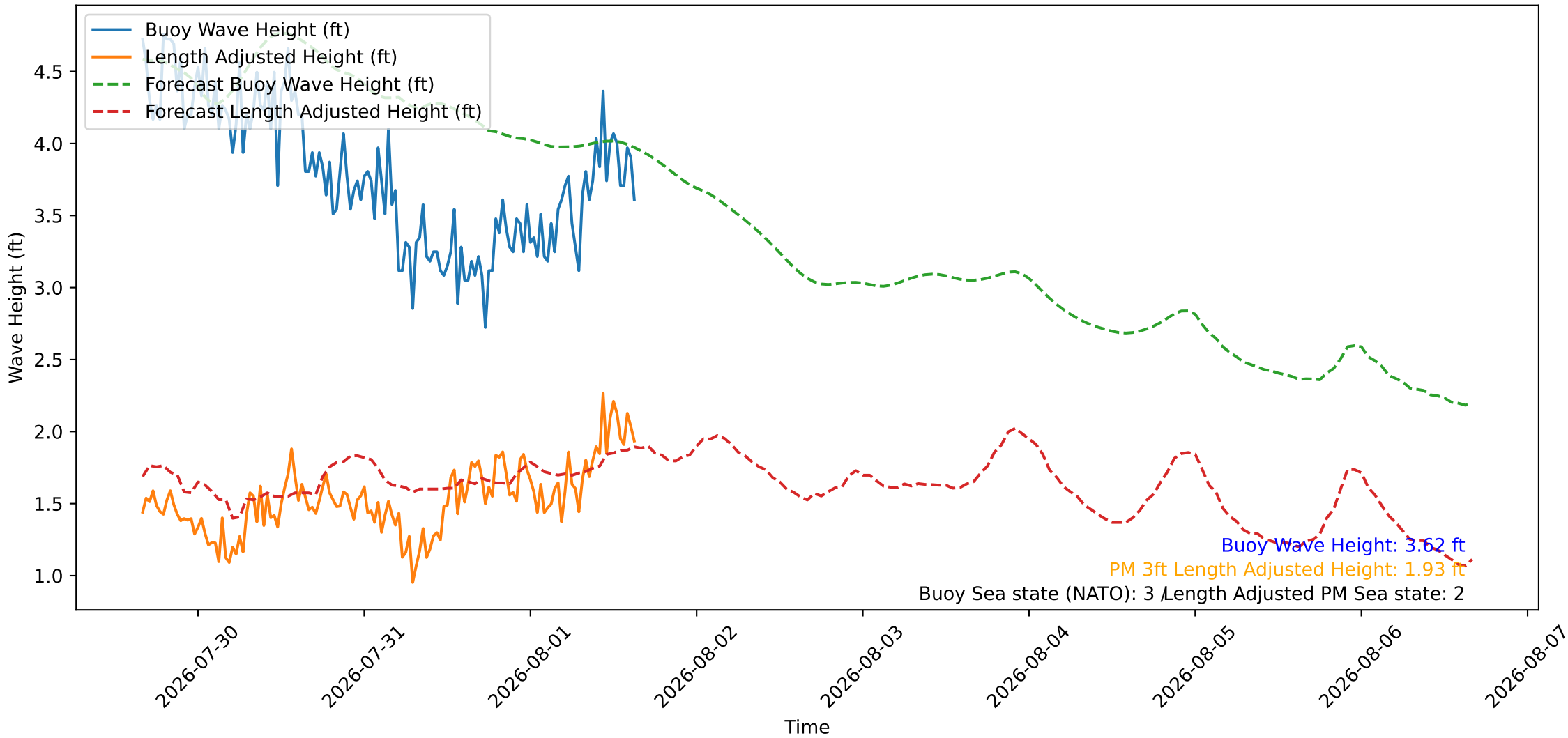
Wave Heights over Time for Oceanside Harbor at 2026-08-01 16:00:26
