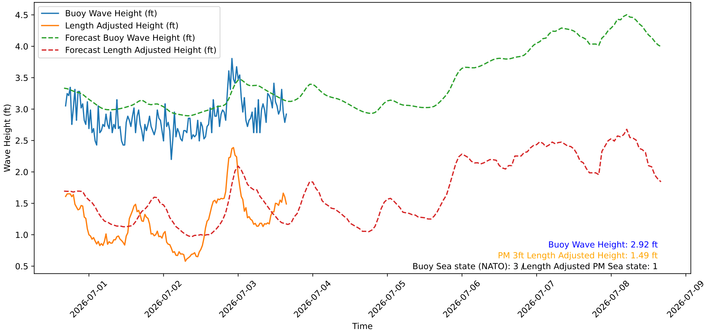
Wave Heights over Time for Red Beach at 2026-07-03 16:10:46
