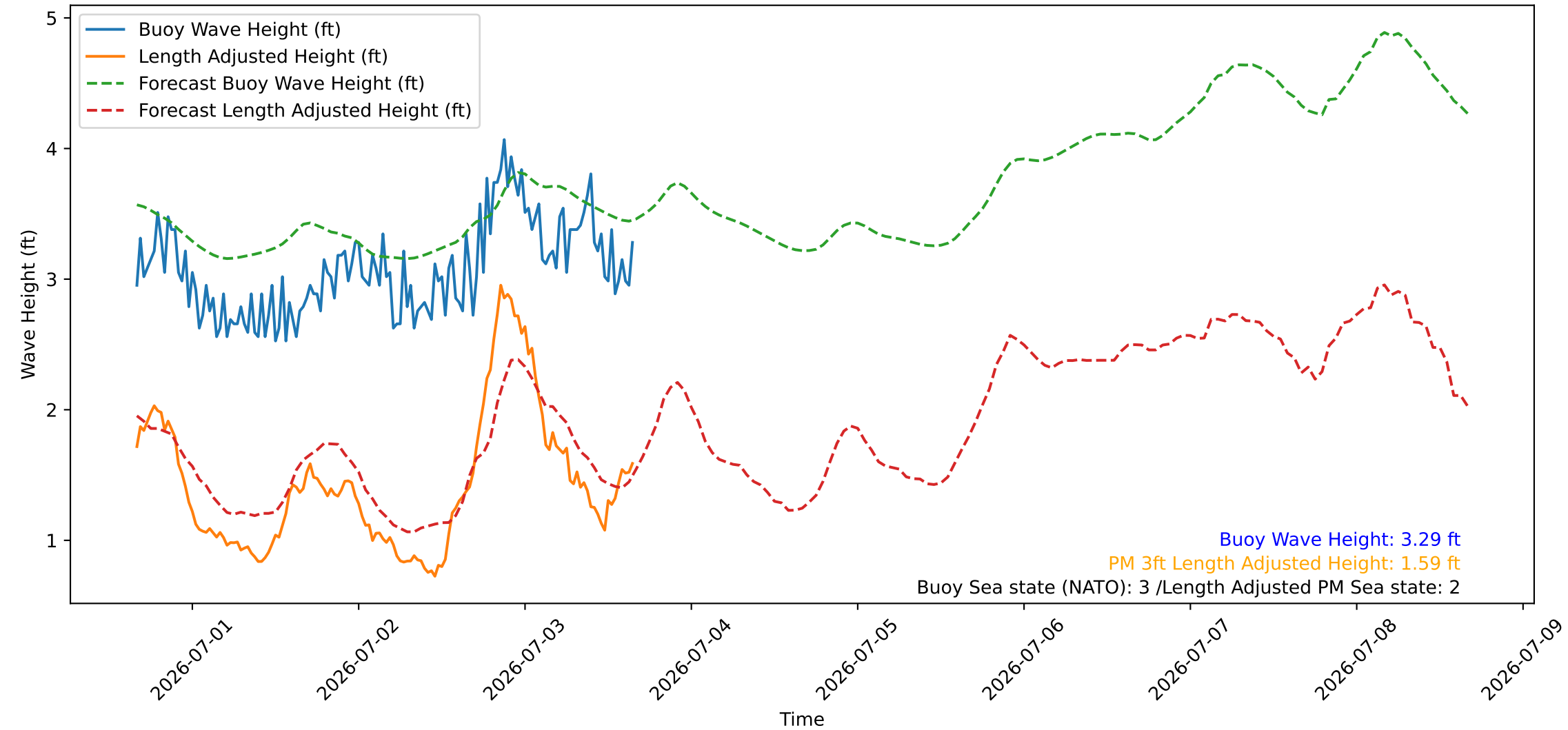
Wave Heights over Time for Green Beach at 2026-07-03 16:11:09
