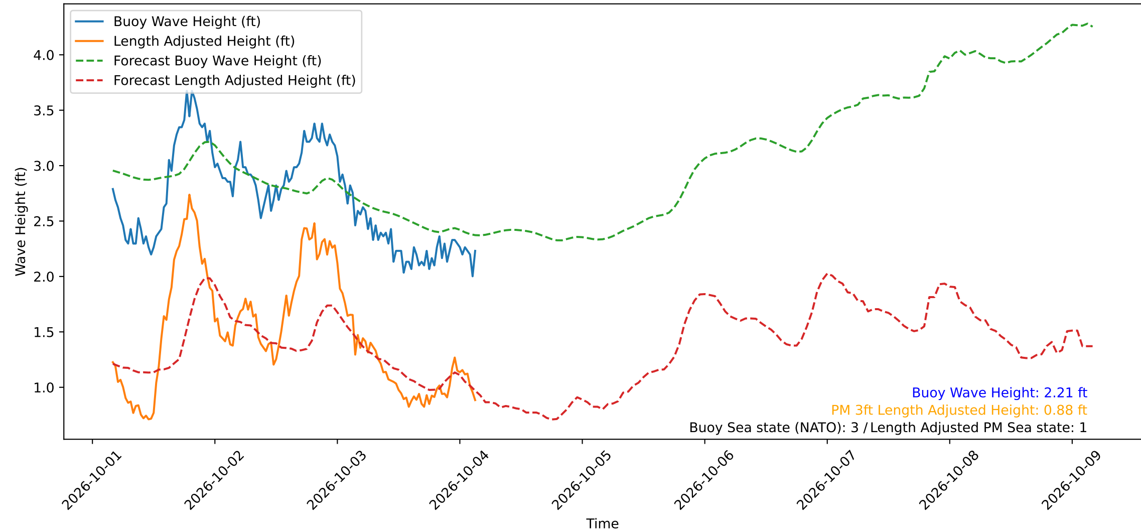
Wave Heights over Time for Green Beach at 2026-10-04 03:51:14
