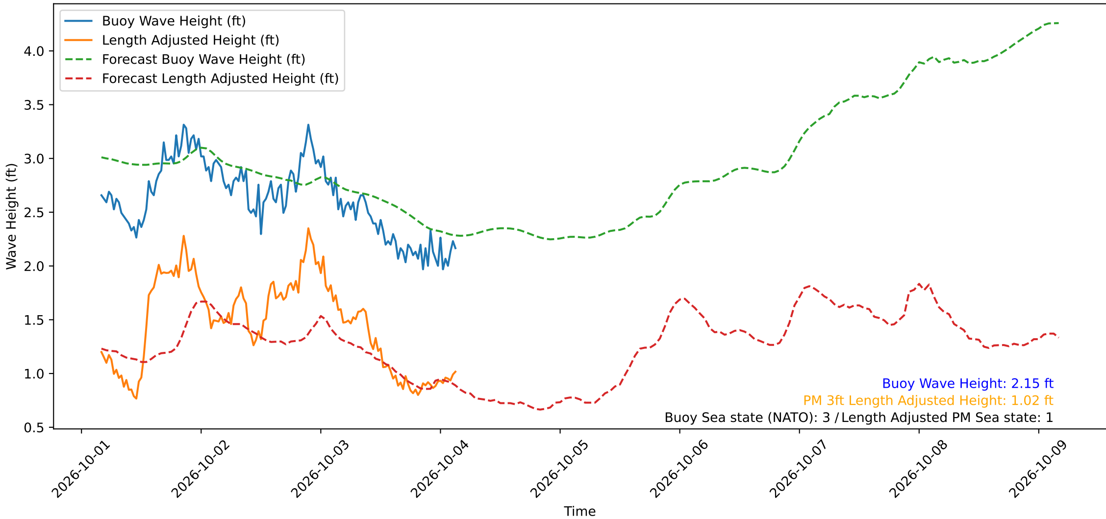
Wave Heights over Time for Oceanside Harbor at 2026-10-04 03:50:29
