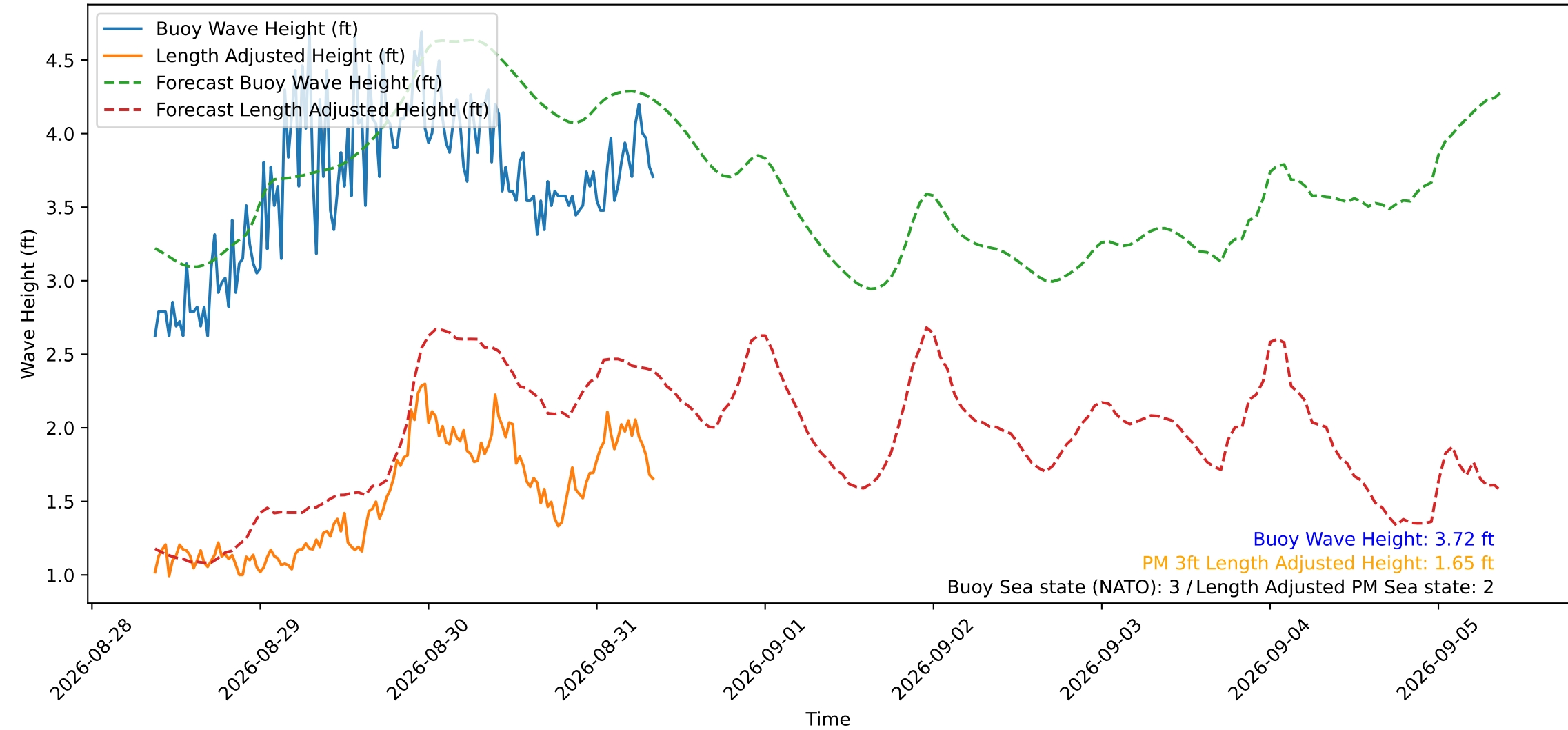
Wave Heights over Time for Red Beach at 2026-08-31 08:50:50
