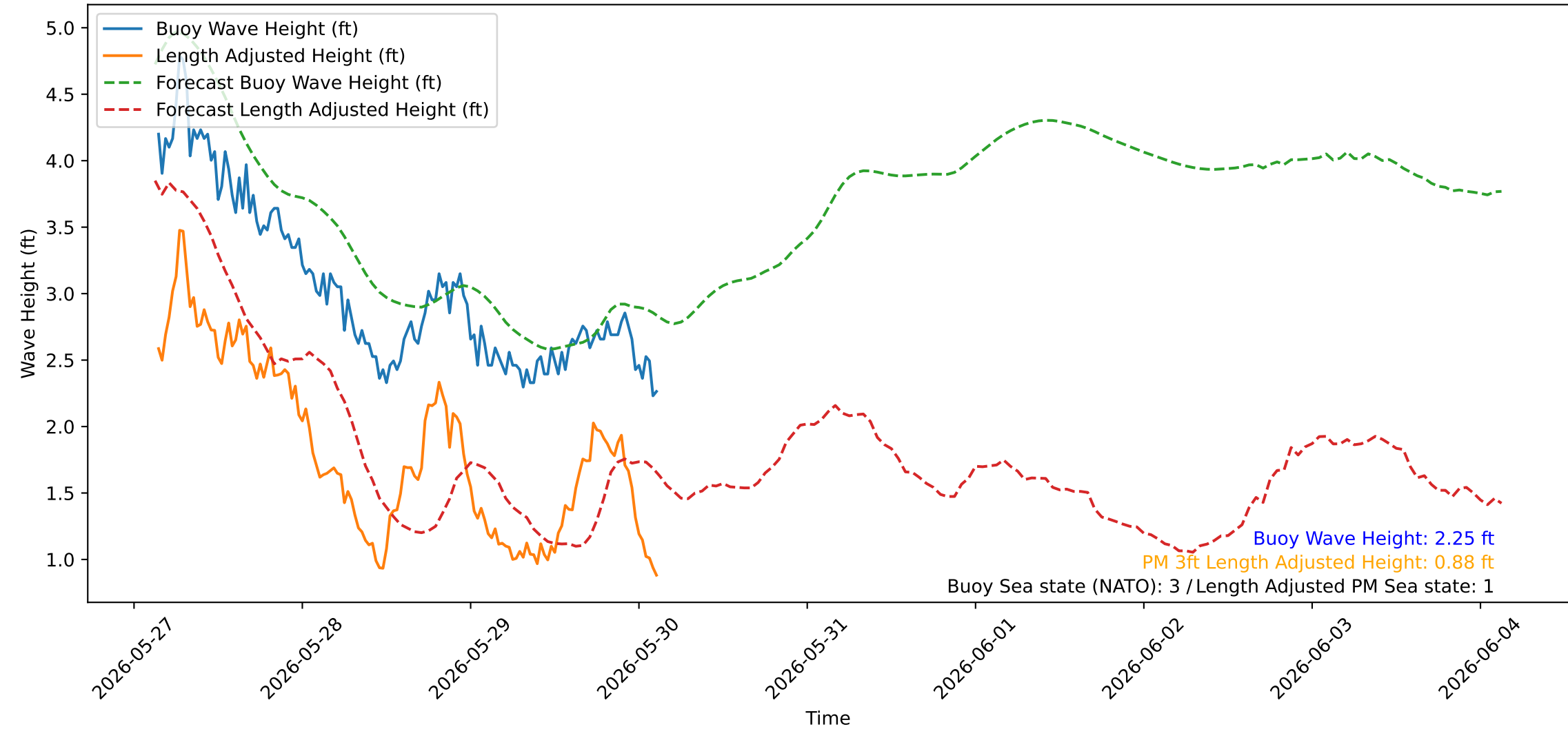
Wave Heights over Time for Red Beach at 2026-05-30 03:10:42
