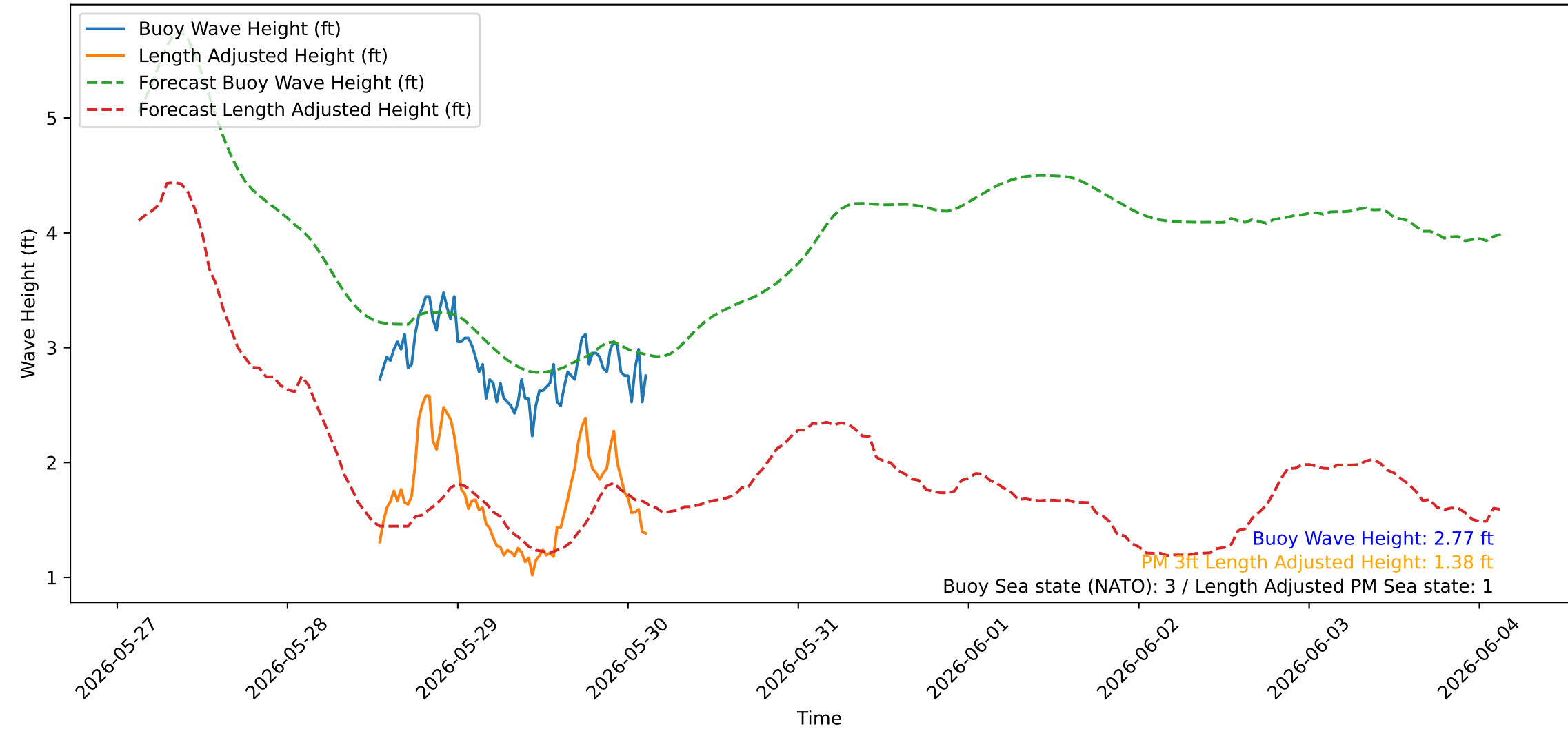
Wave Heights over Time for Oceanside Harbor at 2026-05-30 03:10:23
