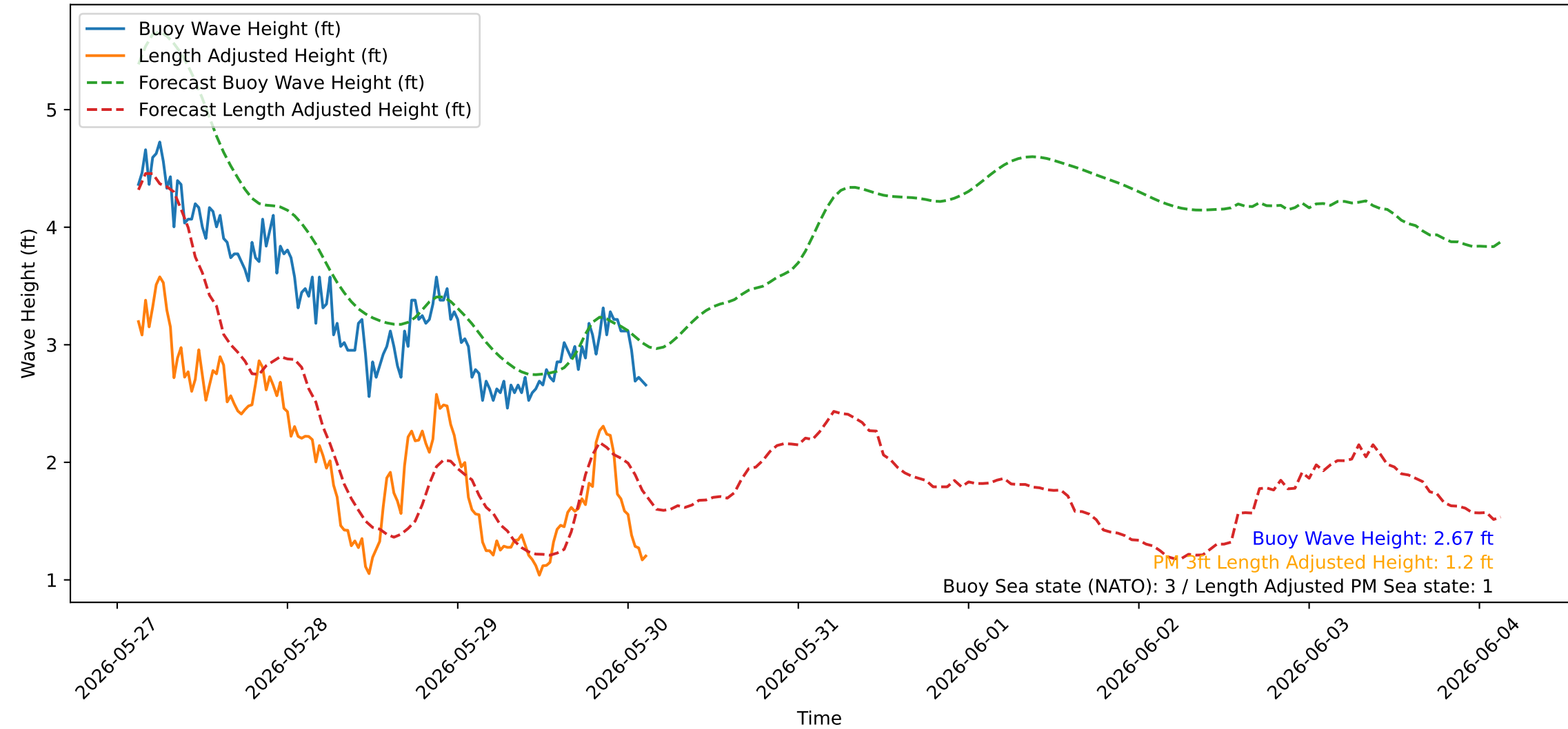
Wave Heights over Time for Green Beach at 2026-05-30 03:11:05
