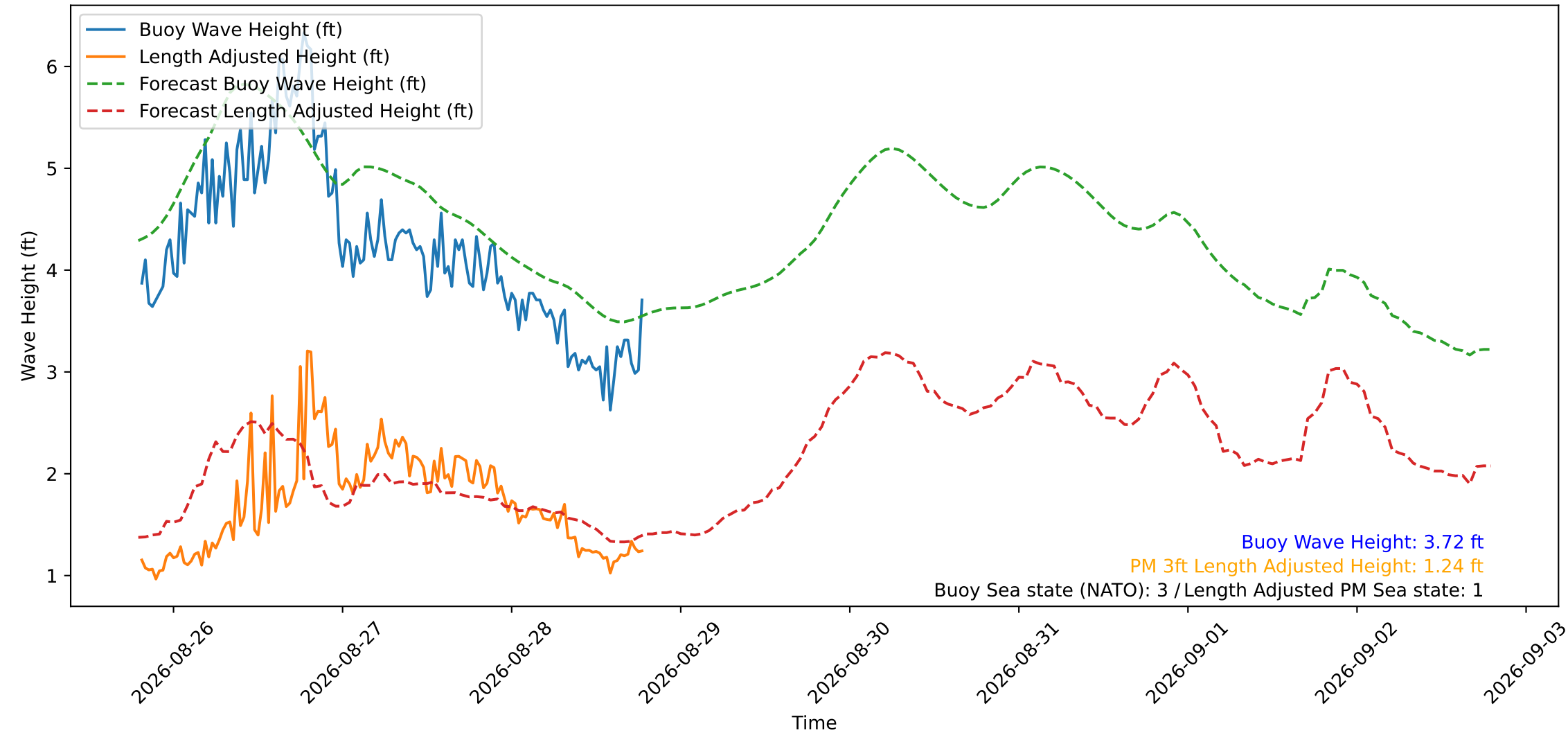
Wave Heights over Time for Green Beach at 2026-08-28 19:11:11
