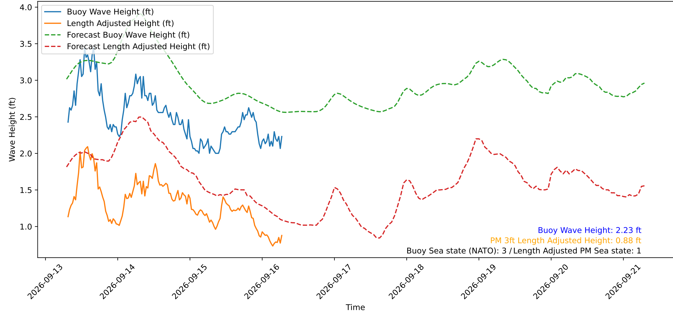
Wave Heights over Time for Red Beach at 2026-09-16 07:20:50
