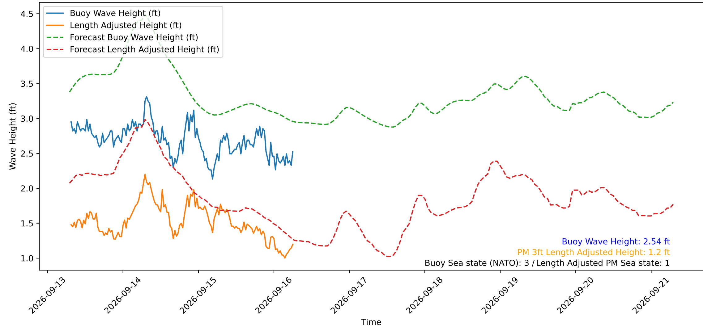
Wave Heights over Time for Green Beach at 2026-09-16 07:21:13
