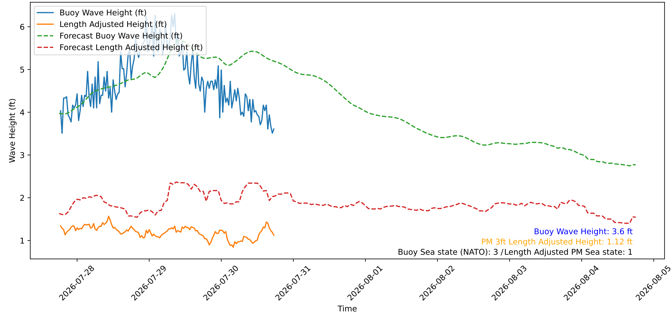
Wave Heights over Time for Green Beach at 2026-07-30 18:21:24
