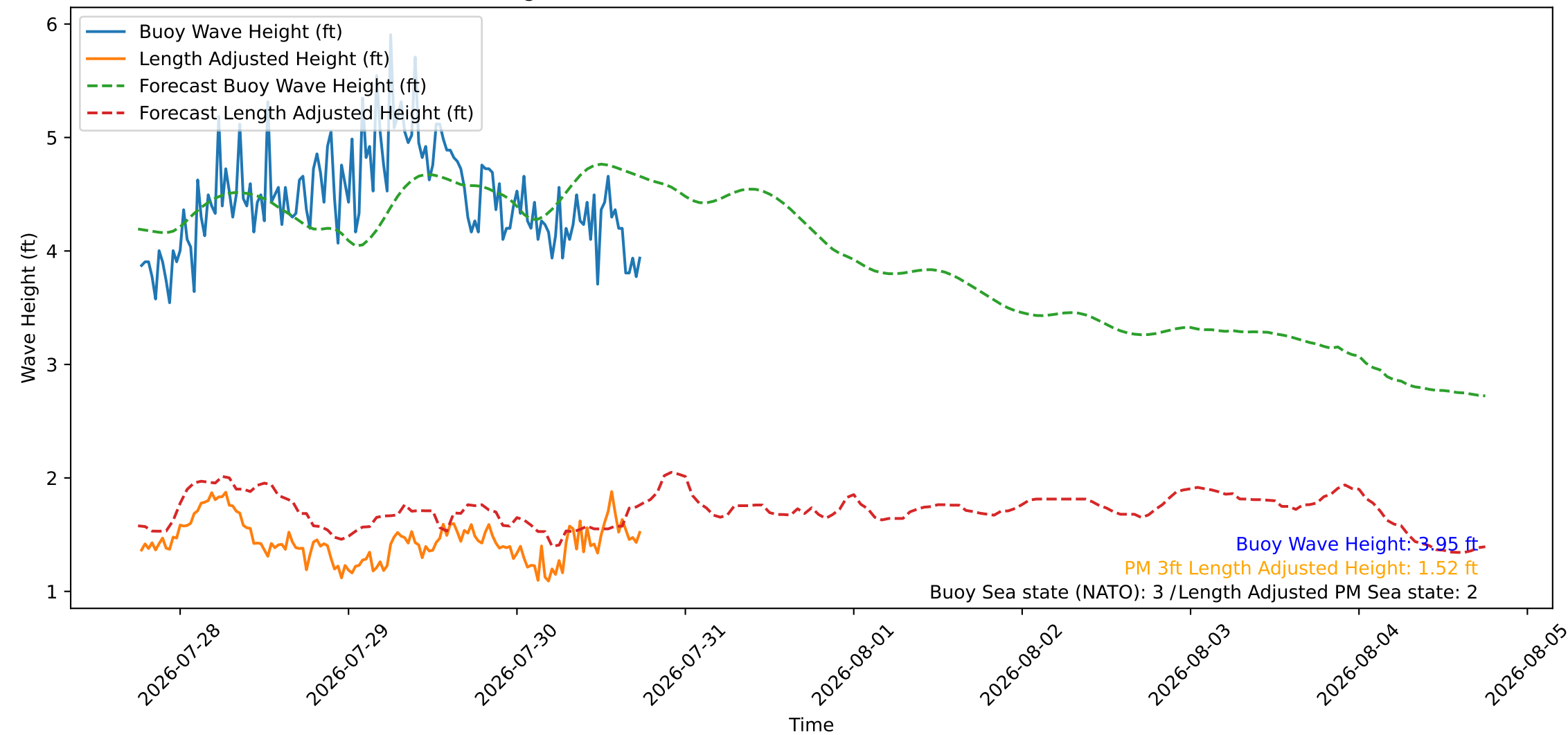
Wave Heights over Time for Oceanside Harbor at 2026-07-30 18:20:31
