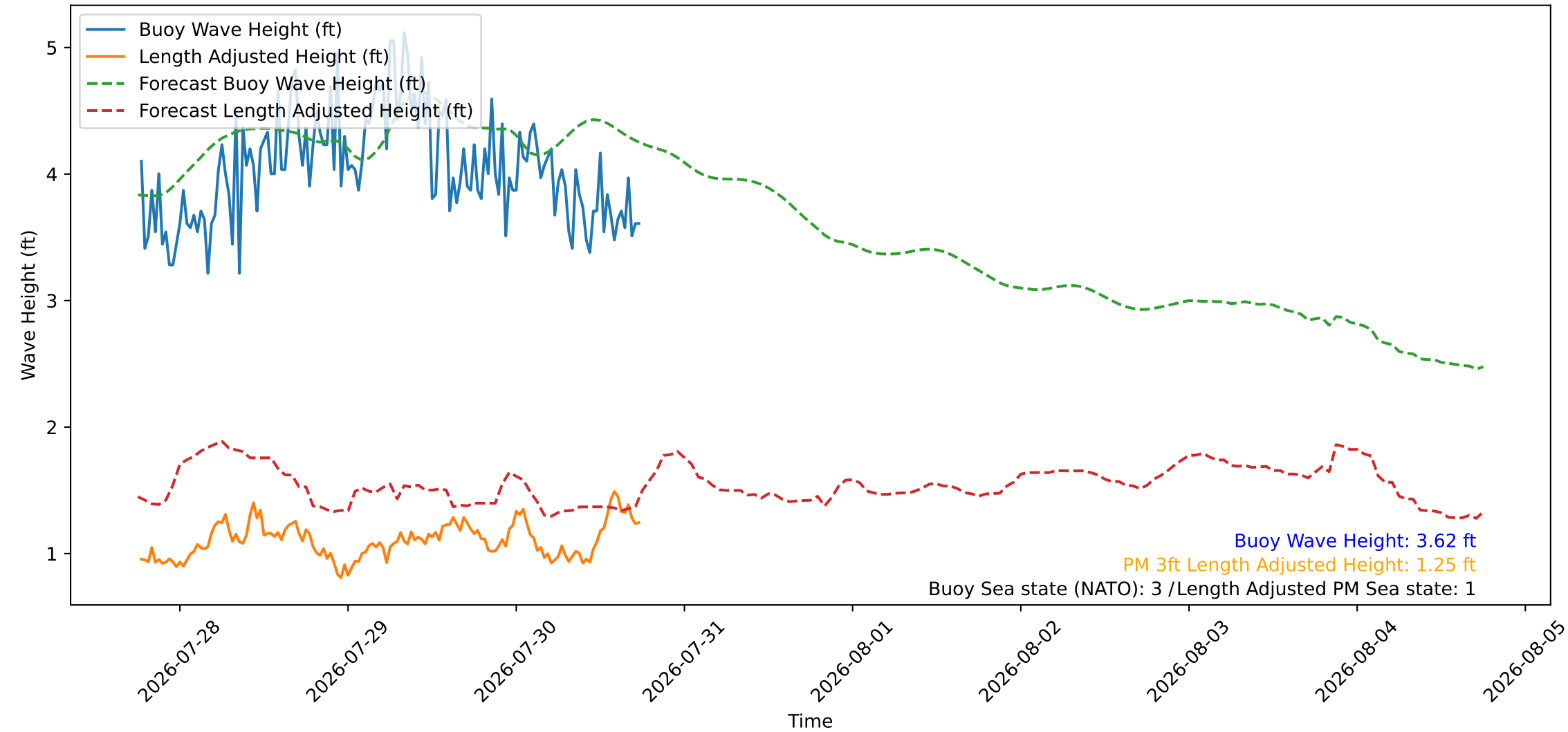
Wave Heights over Time for Red Beach at 2026-07-30 18:20:55
