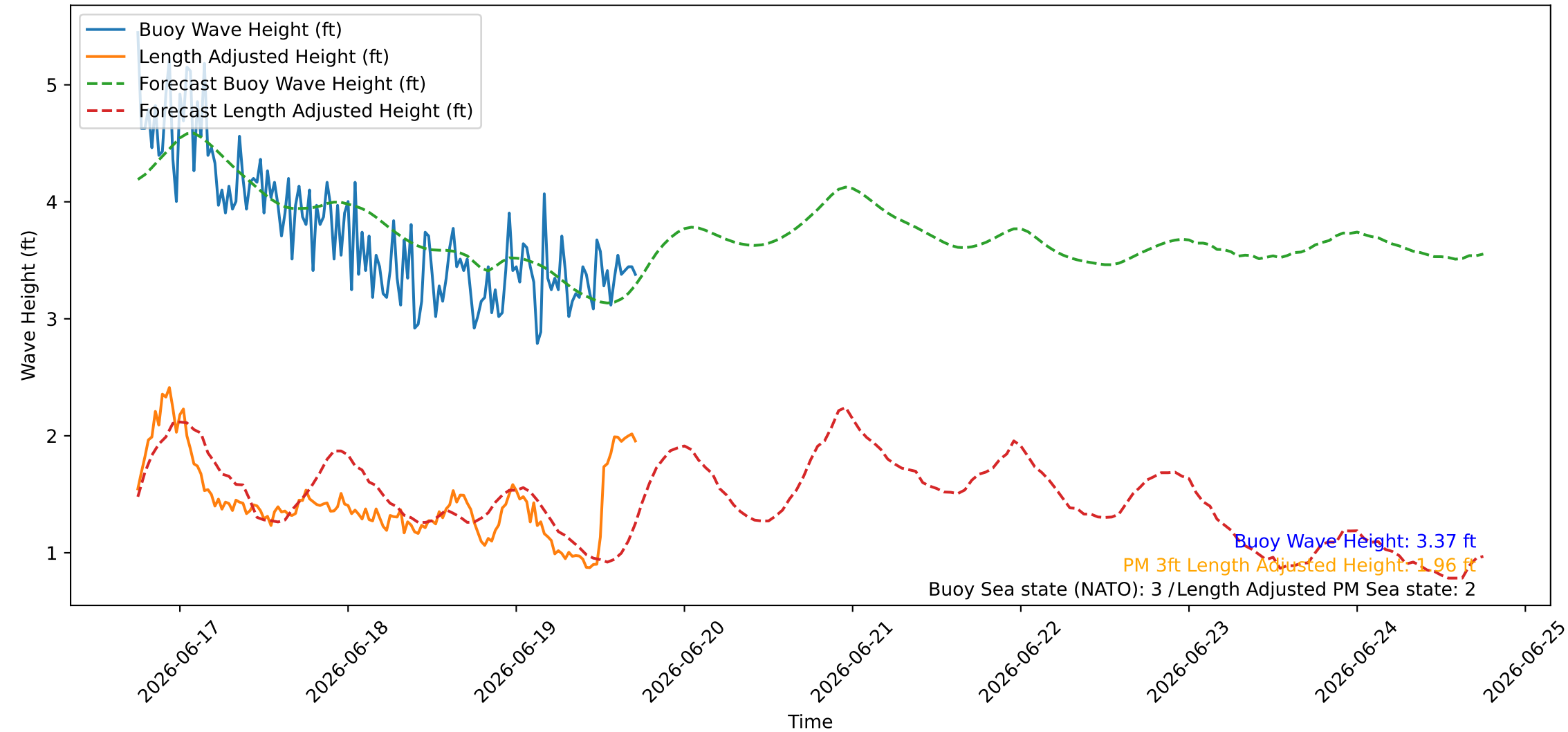
Wave Heights over Time for Oceanside Harbor at 2026-06-19 18:00:26
