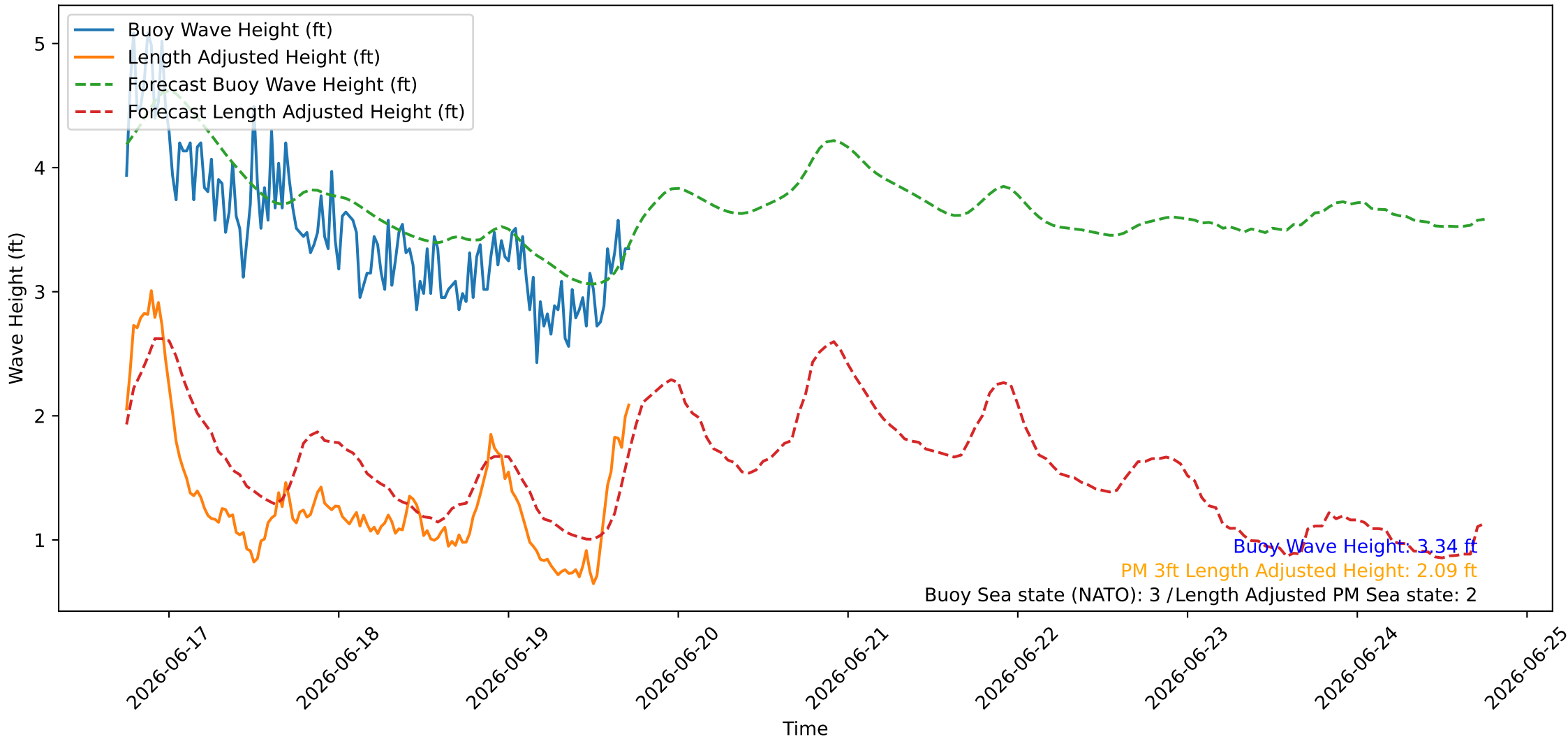
Wave Heights over Time for Green Beach at 2026-06-19 18:01:08
