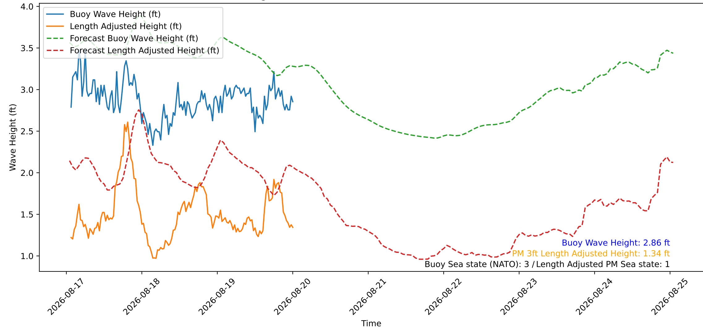
Wave Heights over Time for Red Beach at 2026-08-20 01:00:46
