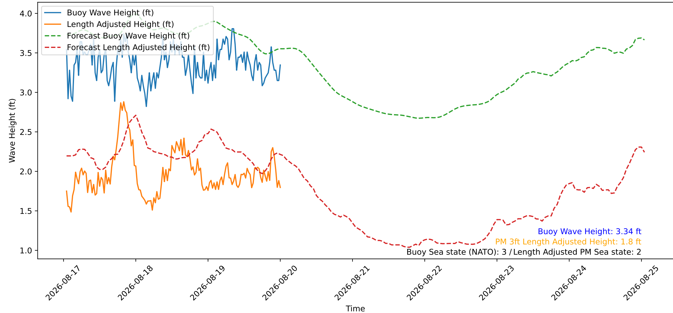
Wave Heights over Time for Oceanside Harbor at 2026-08-20 01:00:26
