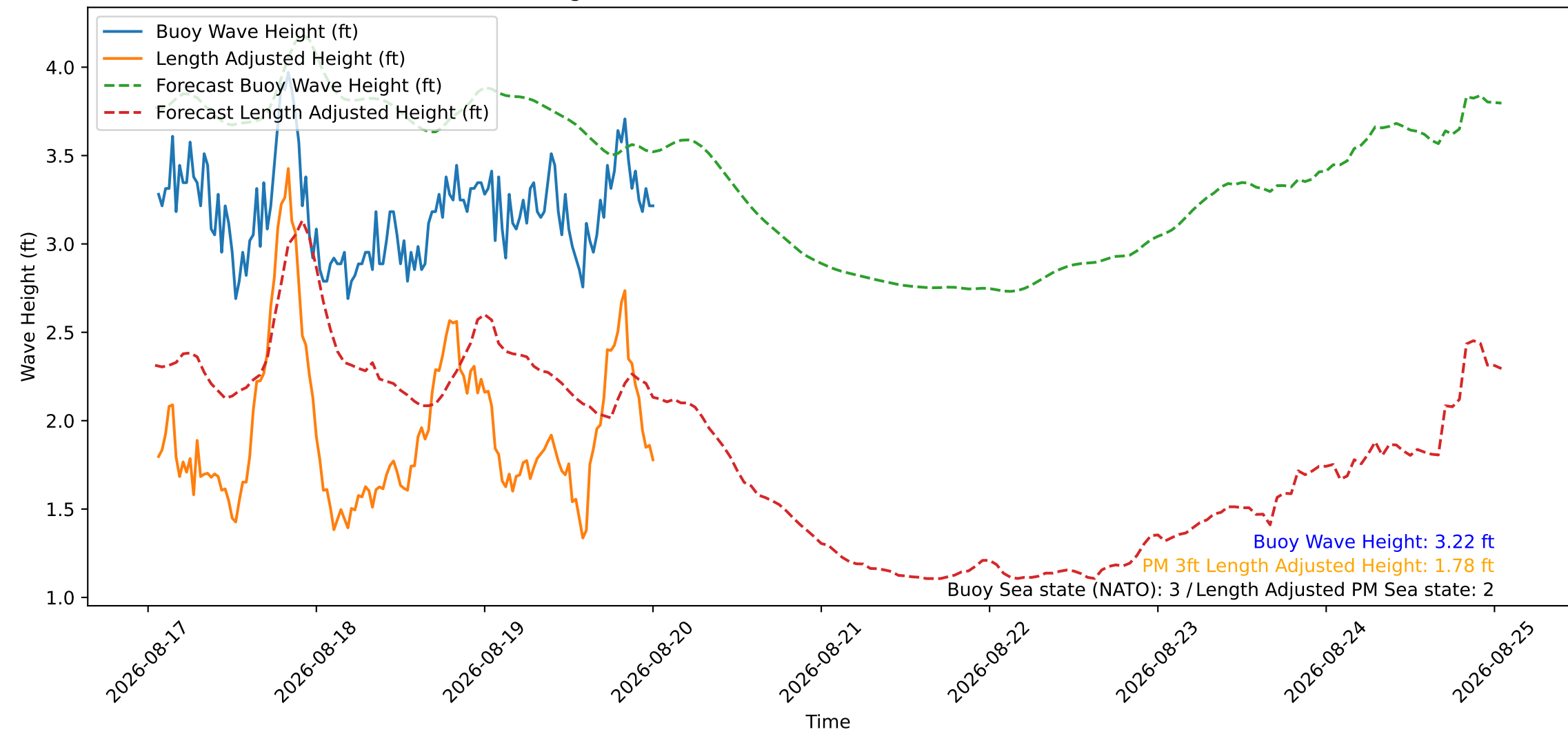
Wave Heights over Time for Green Beach at 2026-08-20 01:01:09
