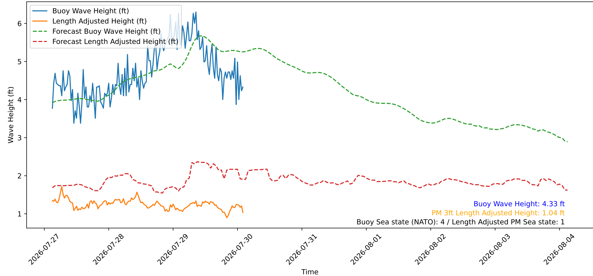
Wave Heights over Time for Green Beach at 2026-07-30 02:51:09
