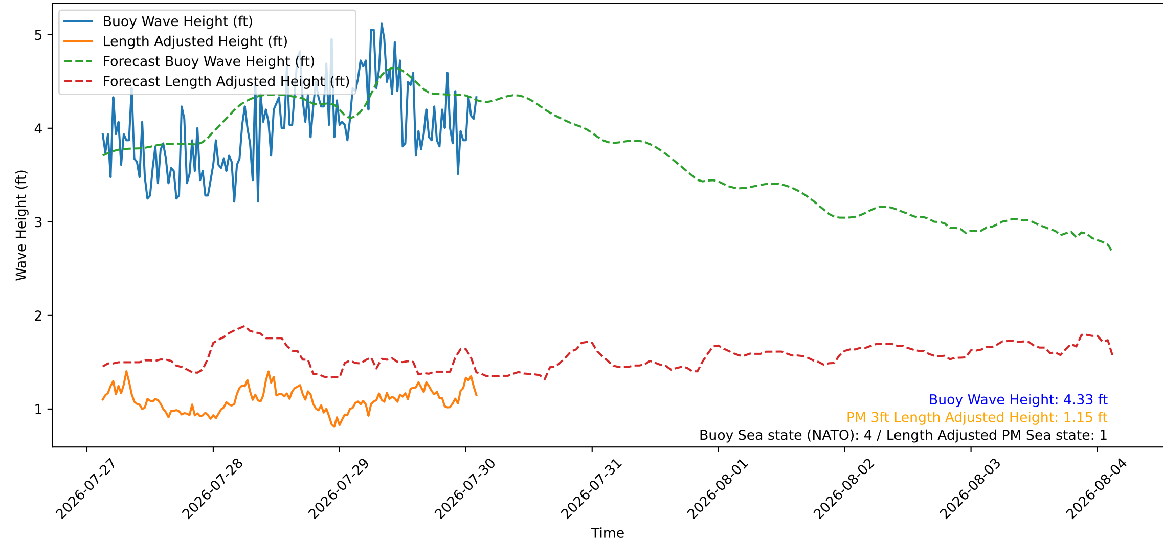
Wave Heights over Time for Red Beach at 2026-07-30 02:50:47
