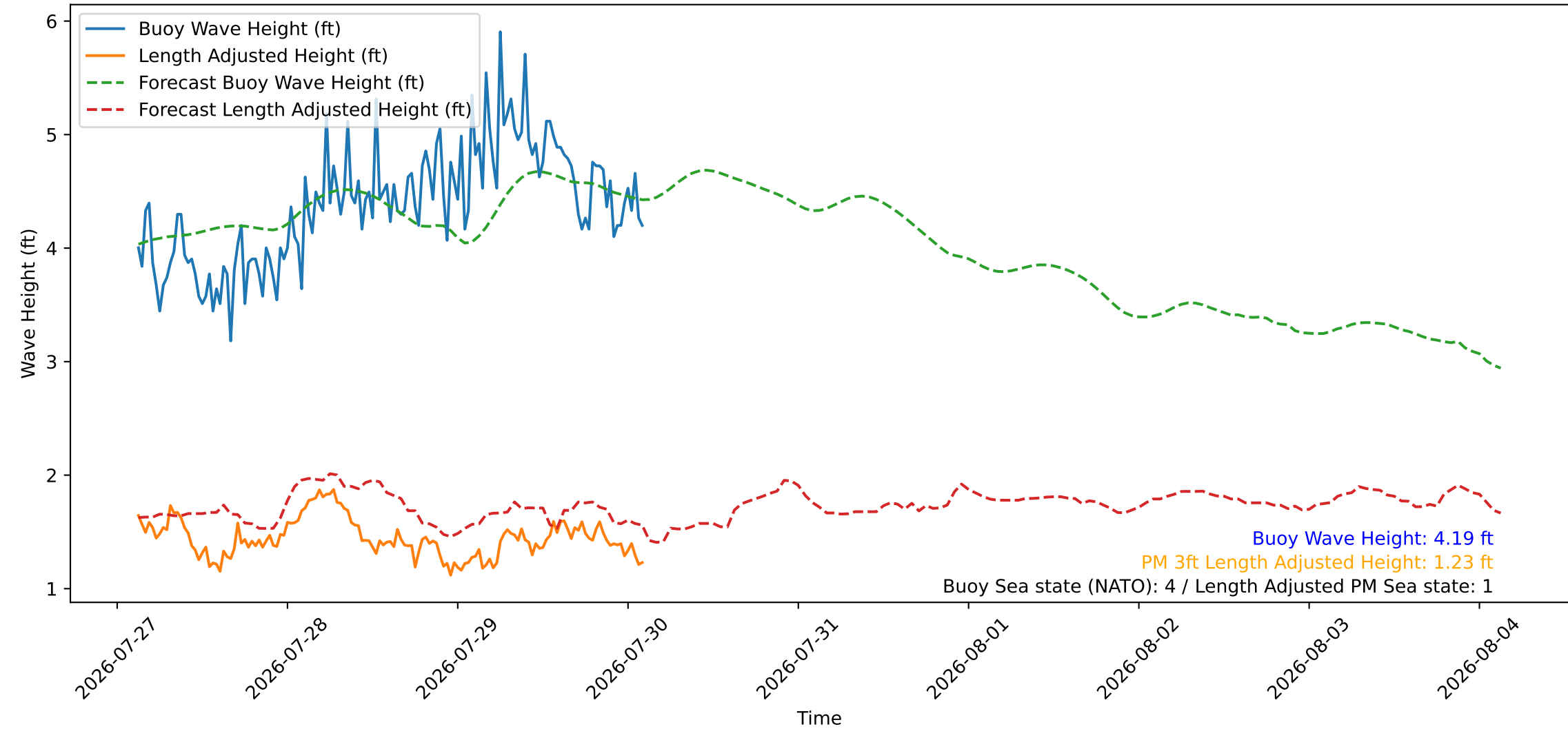
Wave Heights over Time for Oceanside Harbor at 2026-07-30 02:50:26
