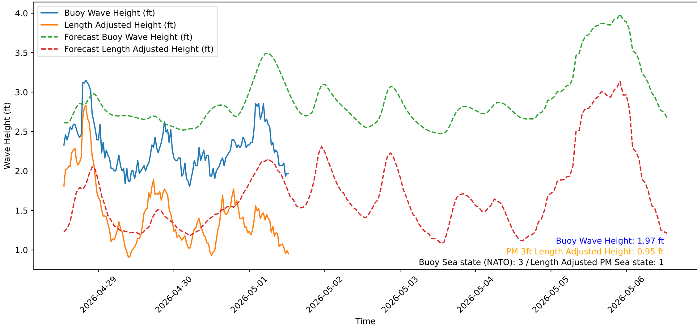
Wave Heights over Time for Green Beach at 2026-05-01 13:11:12
