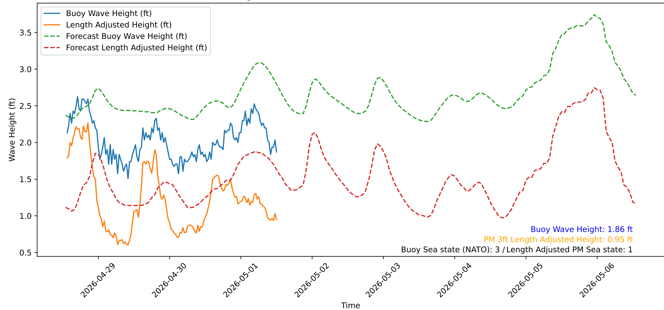
Wave Heights over Time for Red Beach at 2026-05-01 13:10:50
