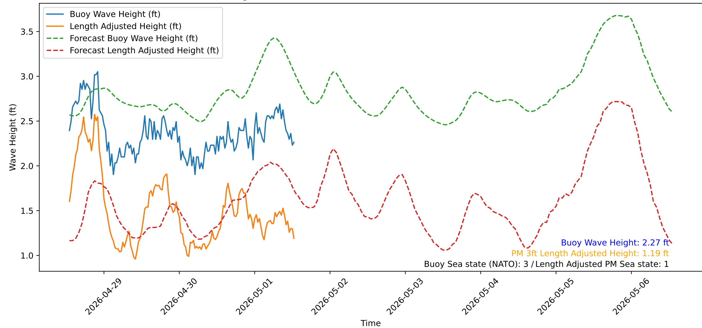
Wave Heights over Time for Oceanside Harbor at 2026-05-01 13:10:31
