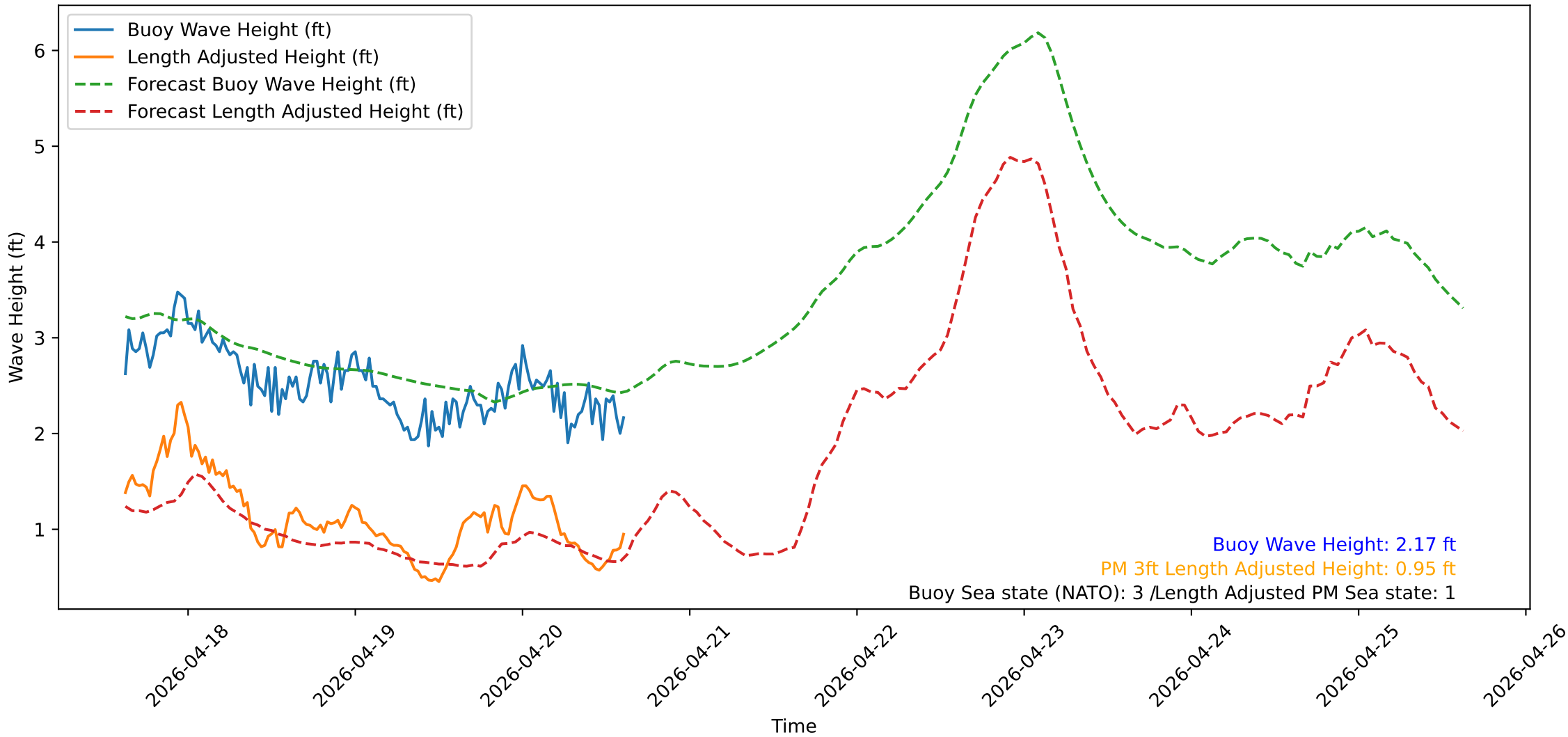
Wave Heights over Time for Green Beach at 2026-04-20 15:11:13
