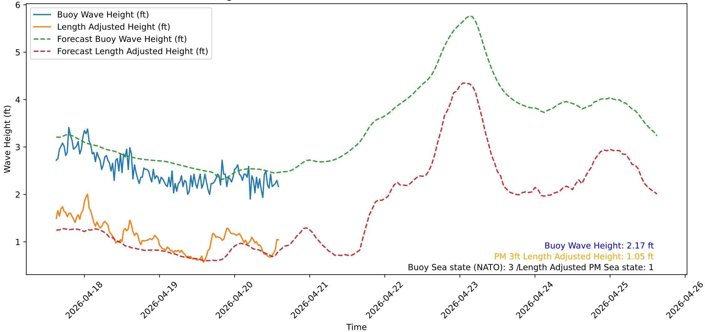
Wave Heights over Time for Oceanside Harbor at 2026-04-20 15:10:32
