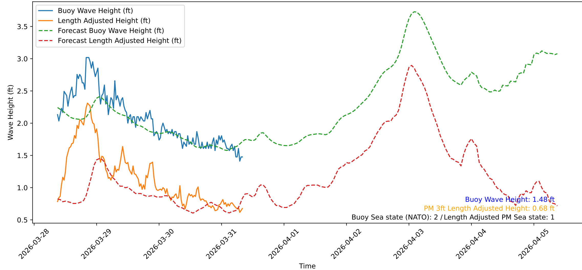
Wave Heights over Time for Red Beach at 2026-03-31 08:50:47
