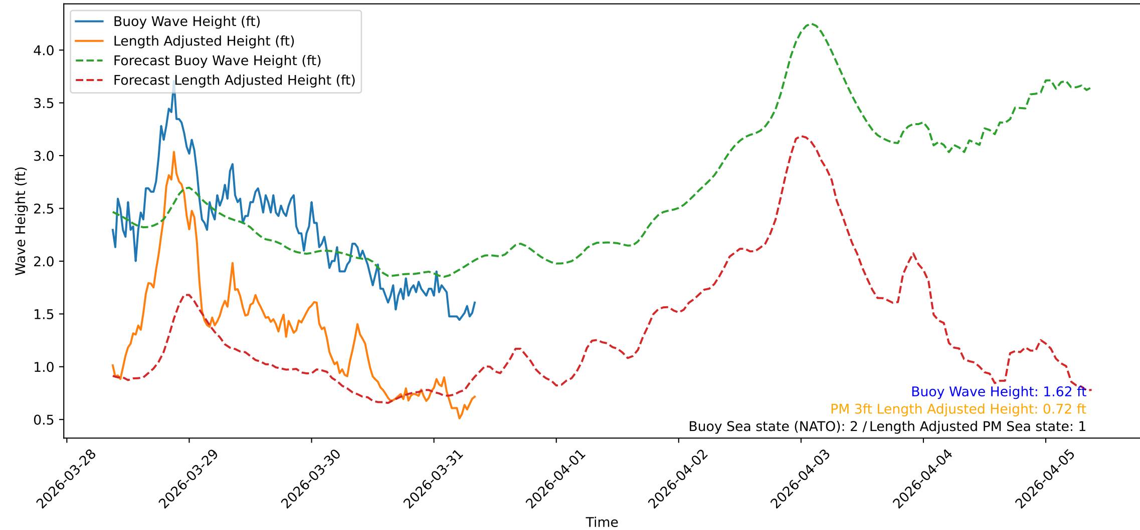
Wave Heights over Time for Green Beach at 2026-03-31 08:51:09
