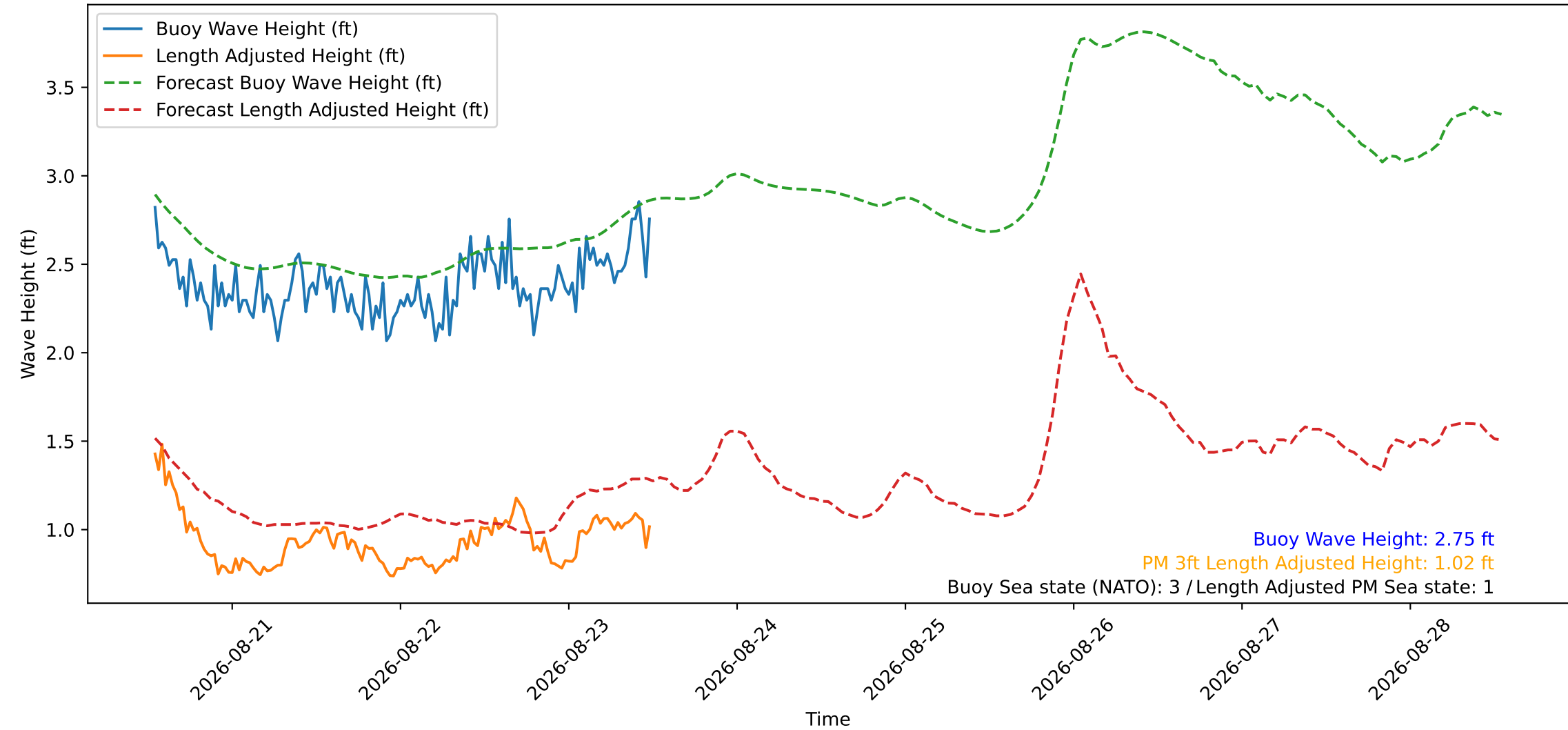
Wave Heights over Time for Red Beach at 2026-08-23 12:30:50
