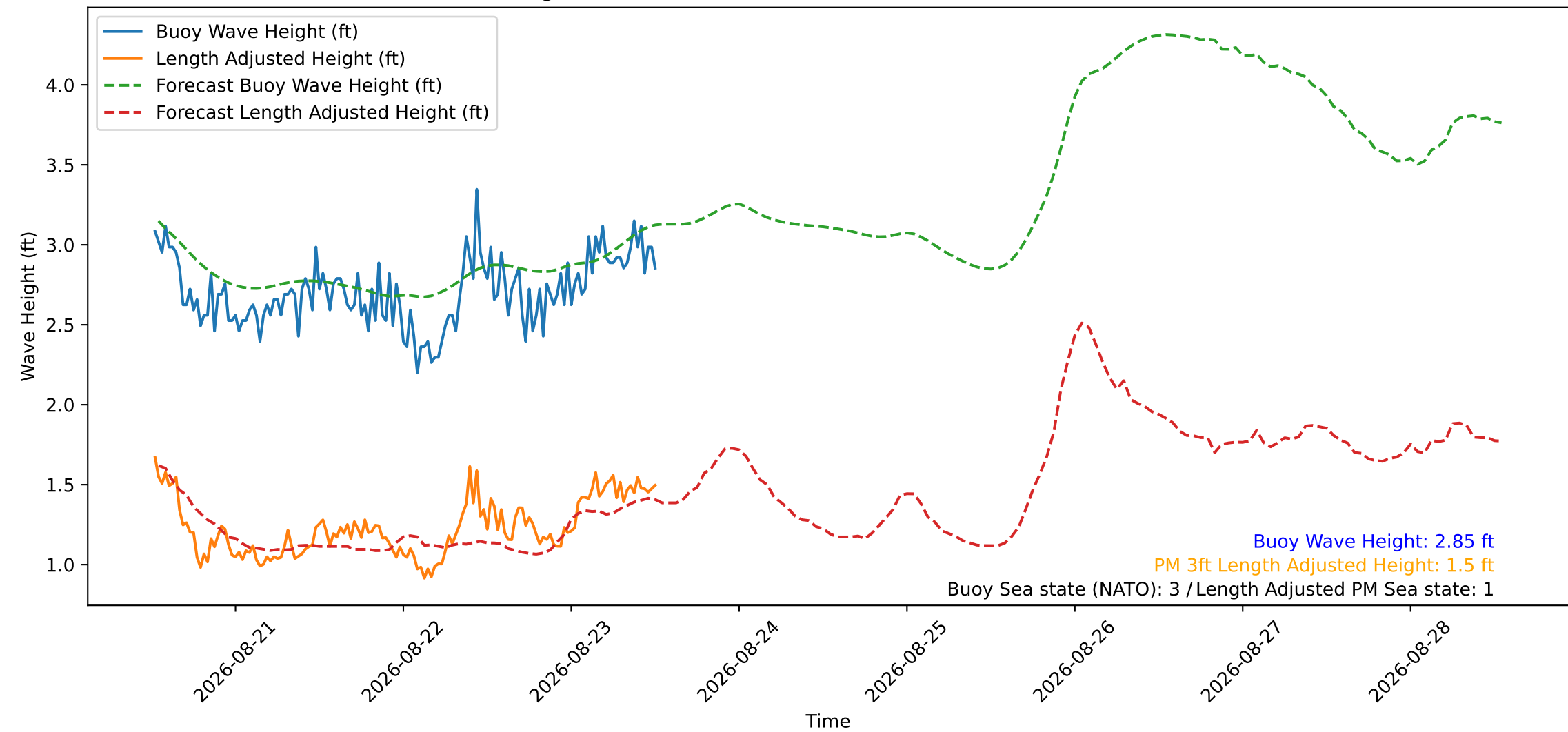
Wave Heights over Time for Oceanside Harbor at 2026-08-23 12:30:30
