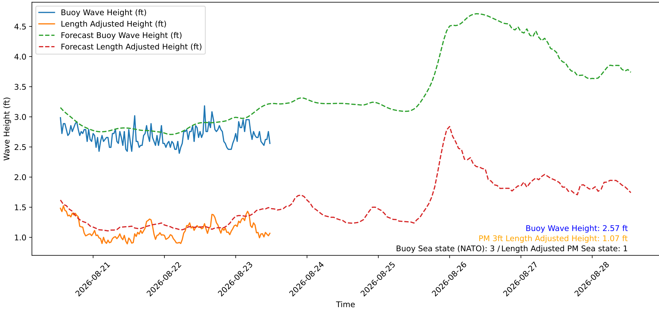
Wave Heights over Time for Green Beach at 2026-08-23 12:31:13
