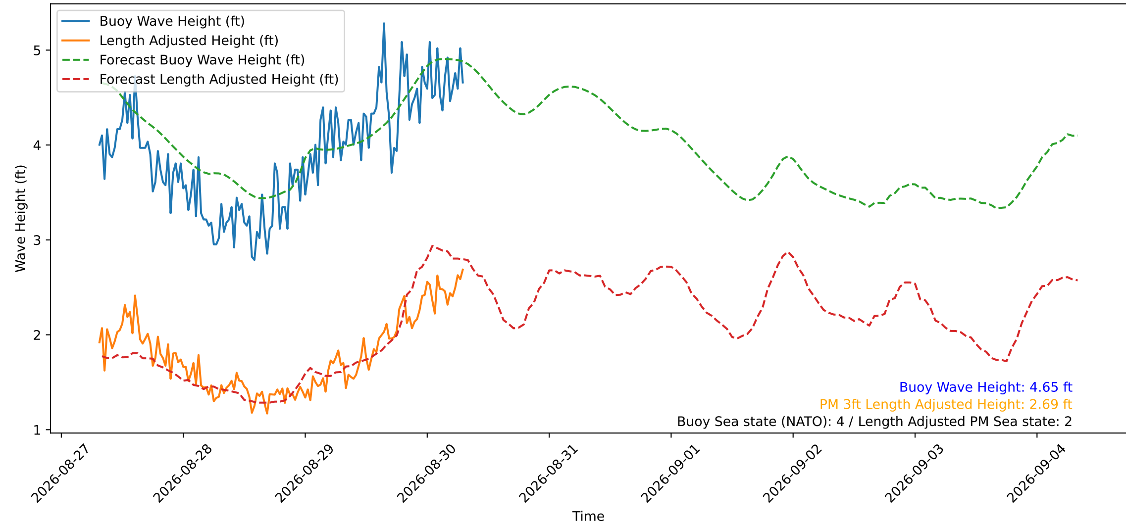
Wave Heights over Time for Oceanside Harbor at 2026-08-30 07:40:30
