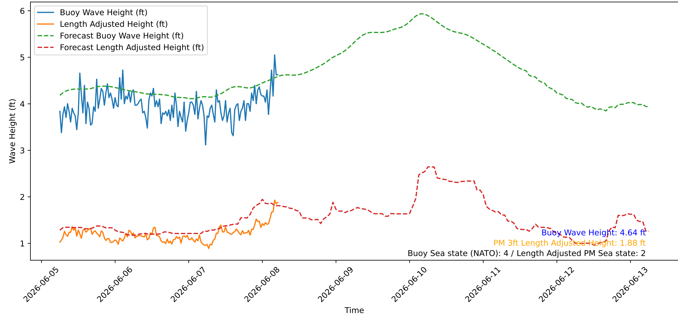
Wave Heights over Time for Green Beach at 2026-06-08 06:01:07
