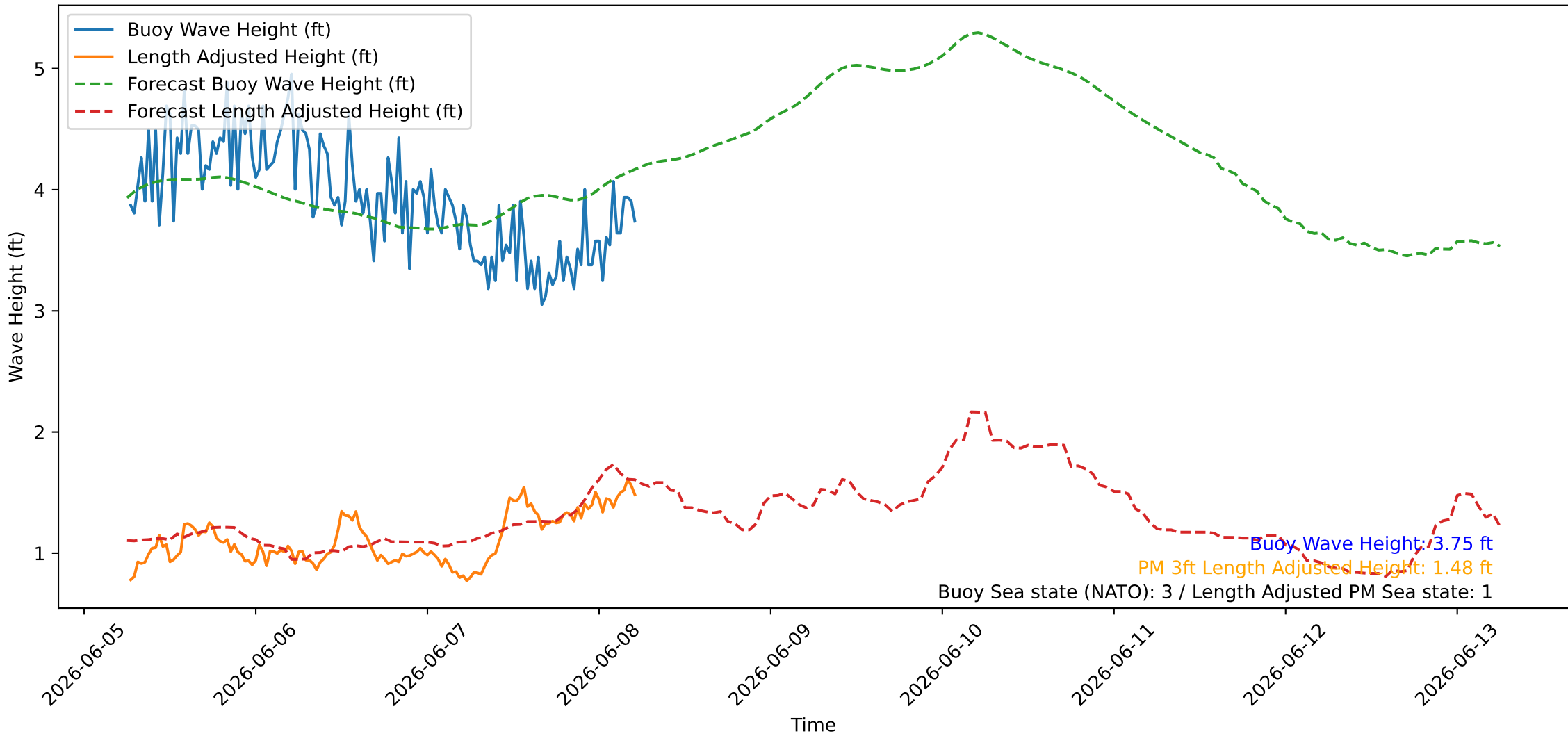
Wave Heights over Time for Red Beach at 2026-06-08 06:00:45
