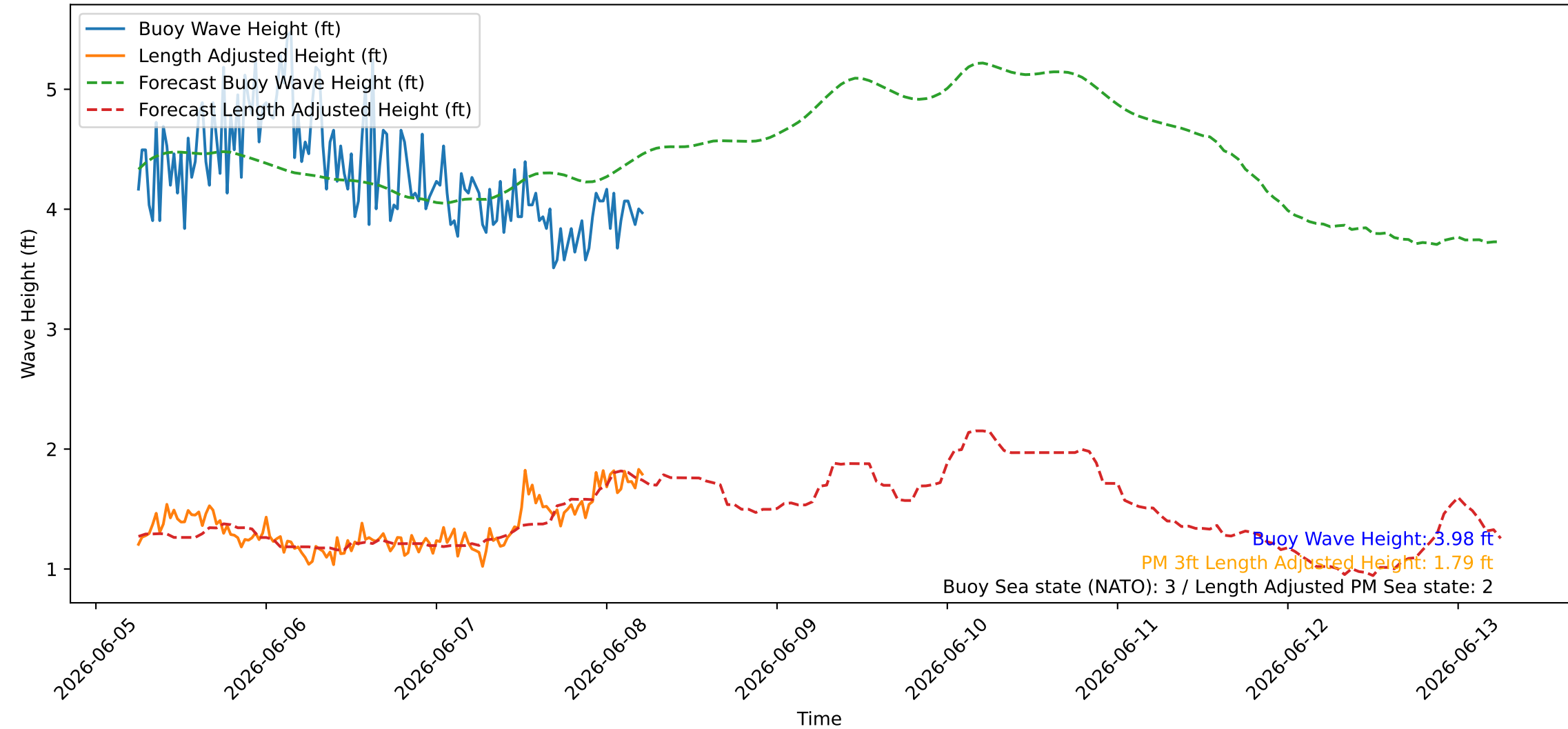
Wave Heights over Time for Oceanside Harbor at 2026-06-08 06:00:26
