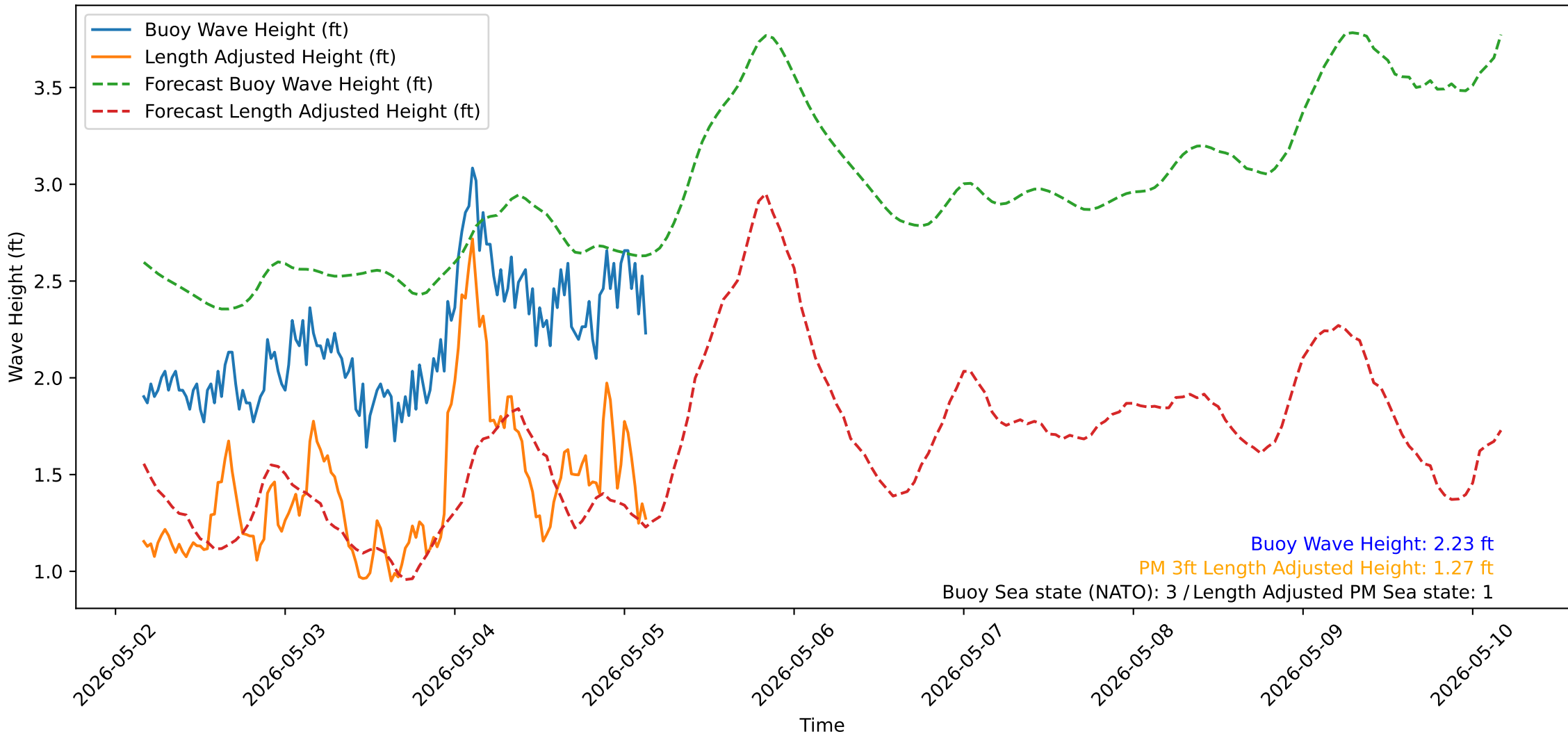
Wave Heights over Time for Oceanside Harbor at 2026-05-05 04:00:31
