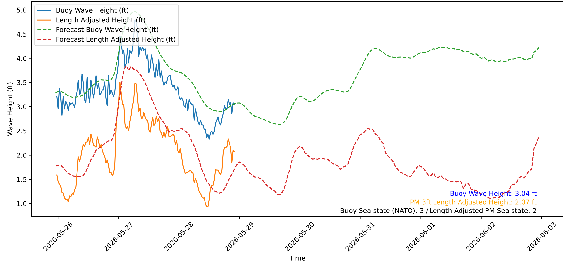
Wave Heights over Time for Red Beach at 2026-05-28 23:00:39
