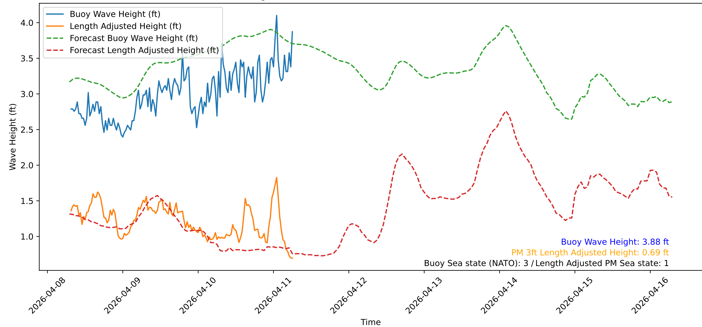
Wave Heights over Time for Red Beach at 2026-04-11 07:00:50
