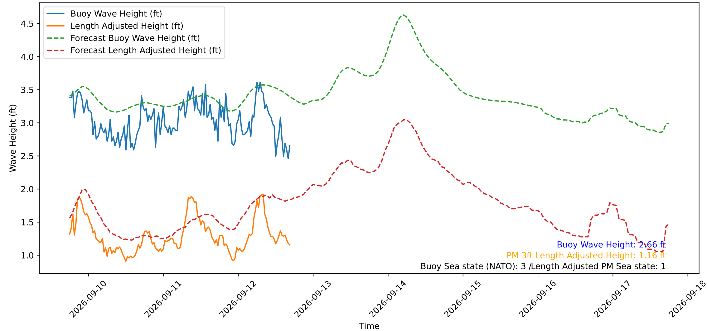
Wave Heights over Time for Green Beach at 2026-09-12 17:31:12
