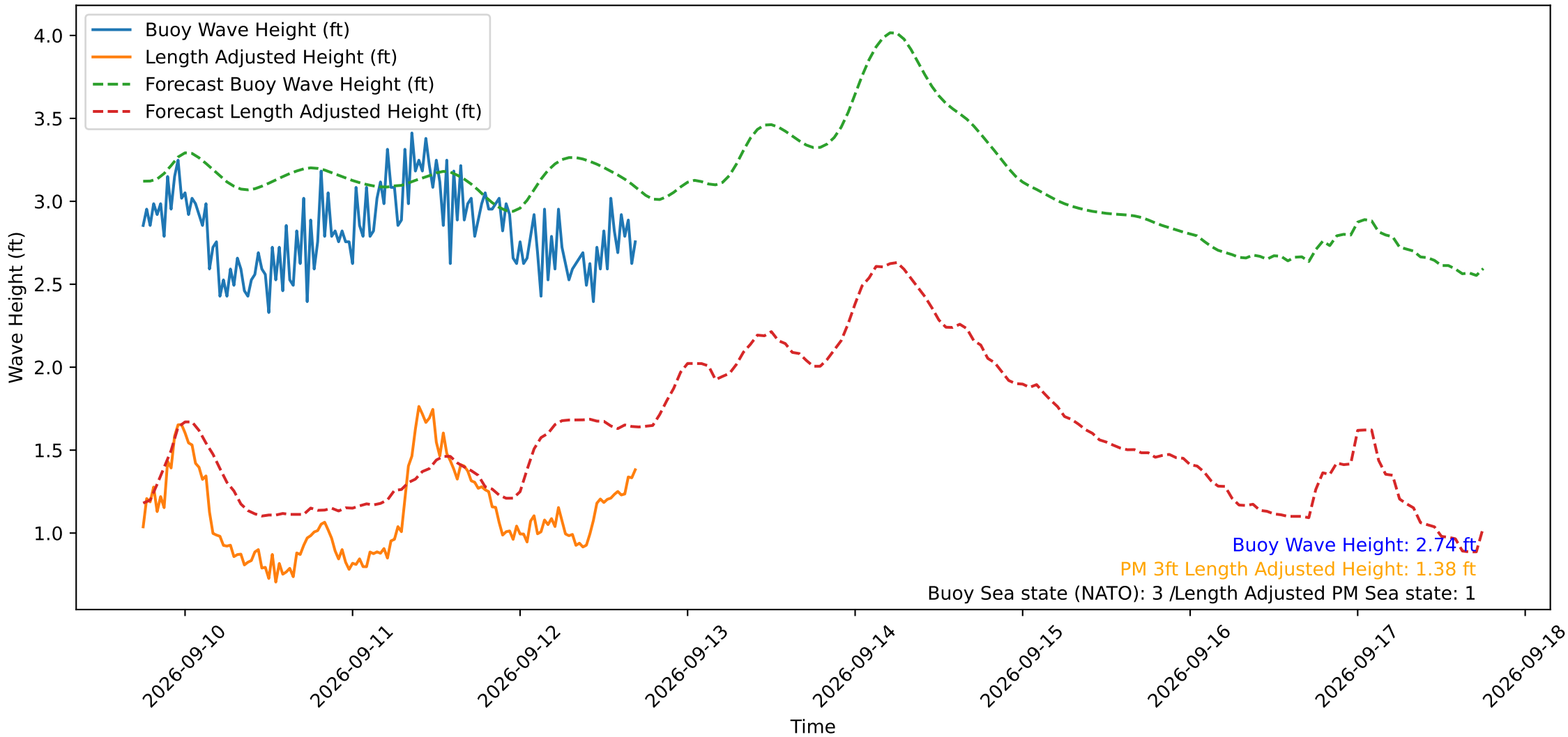
Wave Heights over Time for Red Beach at 2026-09-12 17:30:50
