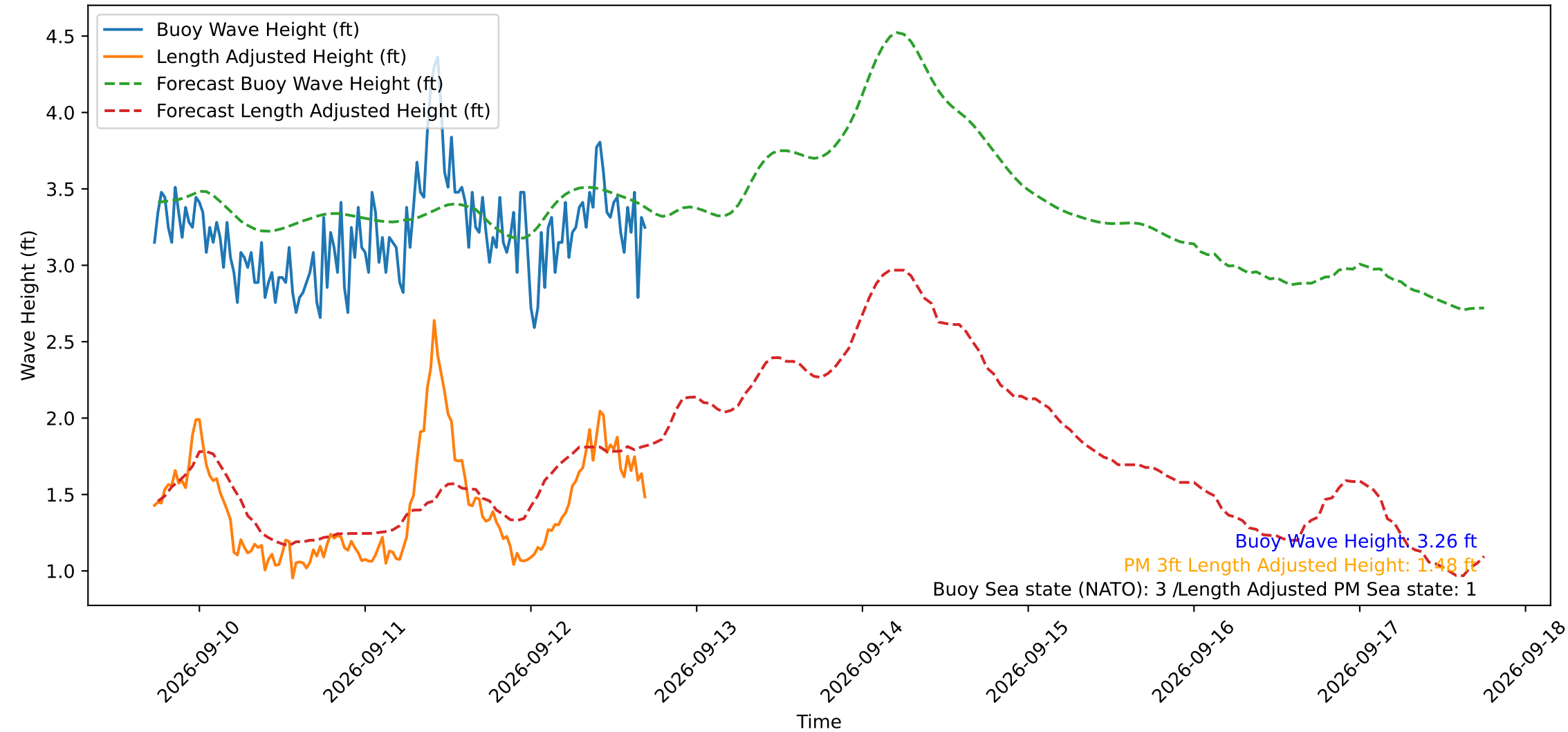
Wave Heights over Time for Oceanside Harbor at 2026-09-12 17:30:30
