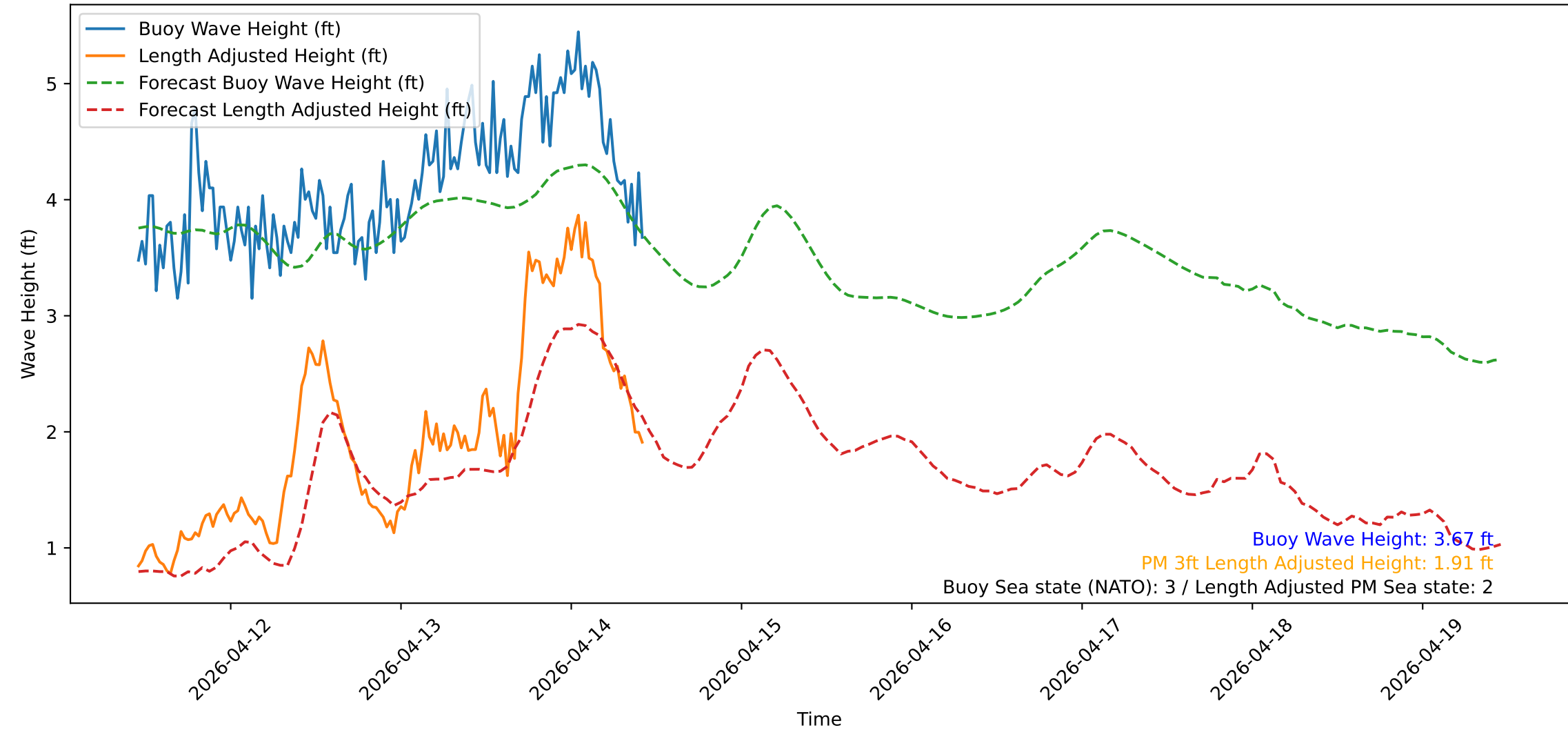
Wave Heights over Time for Oceanside Harbor at 2026-04-14 10:50:31
