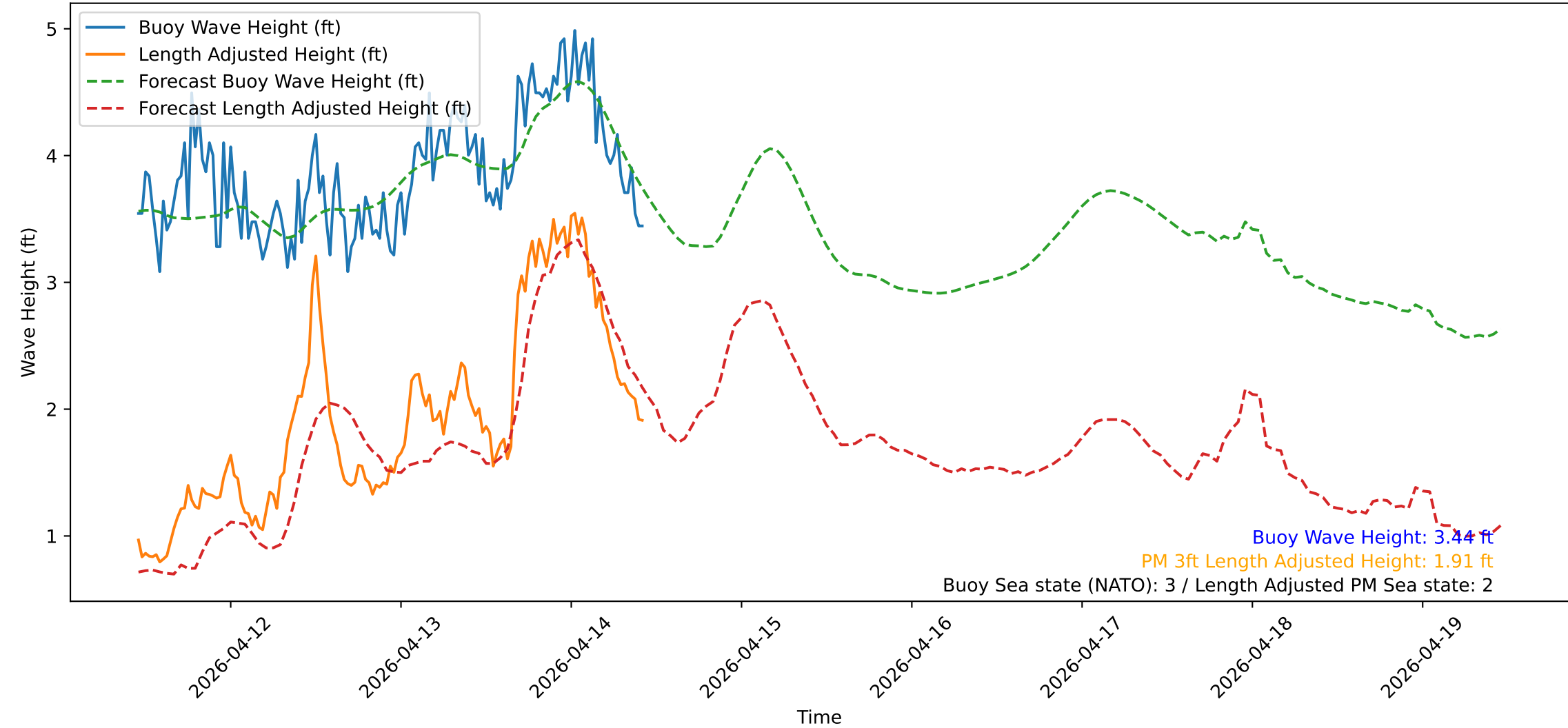
Wave Heights over Time for Green Beach at 2026-04-14 10:51:13
