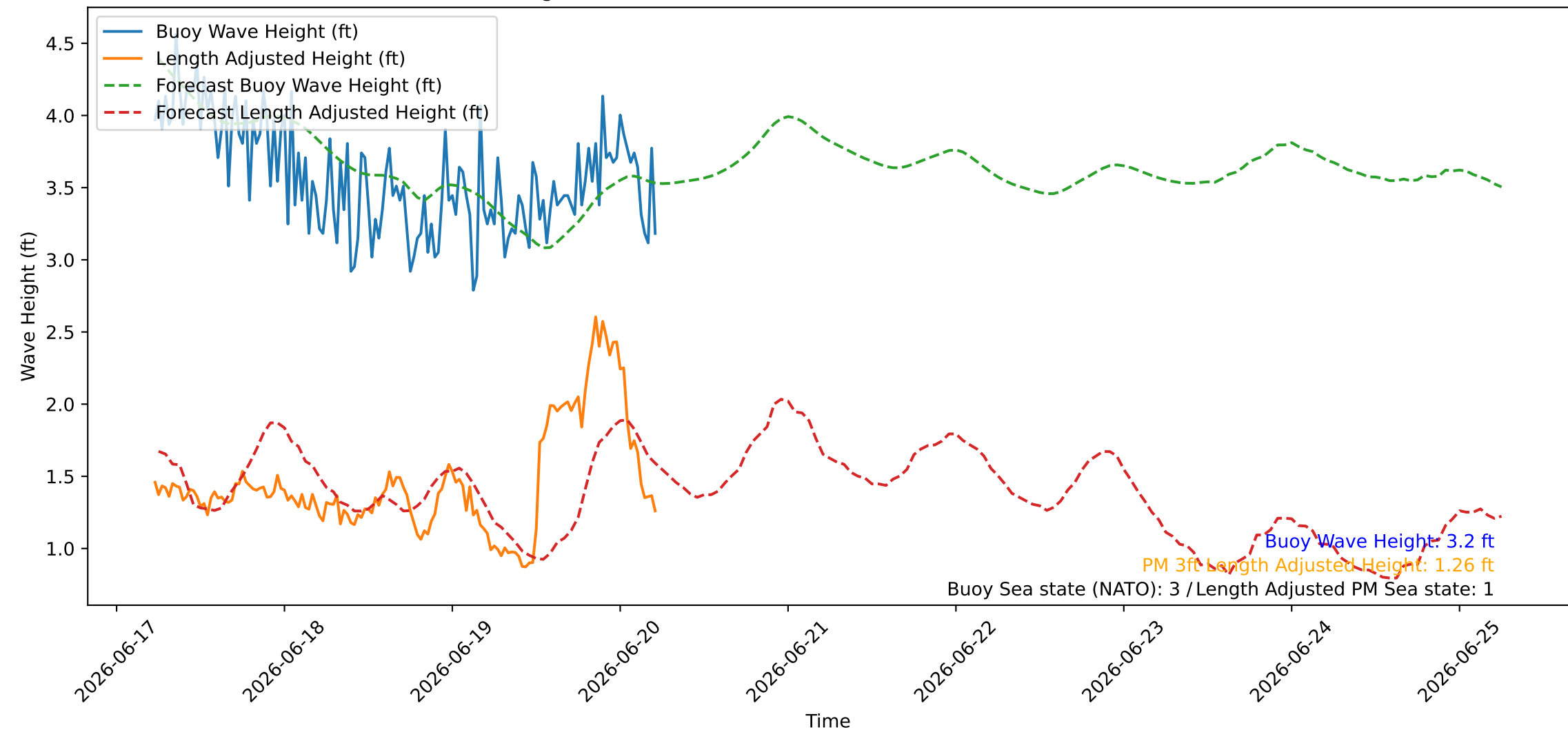
Wave Heights over Time for Oceanside Harbor at 2026-06-20 05:40:26
