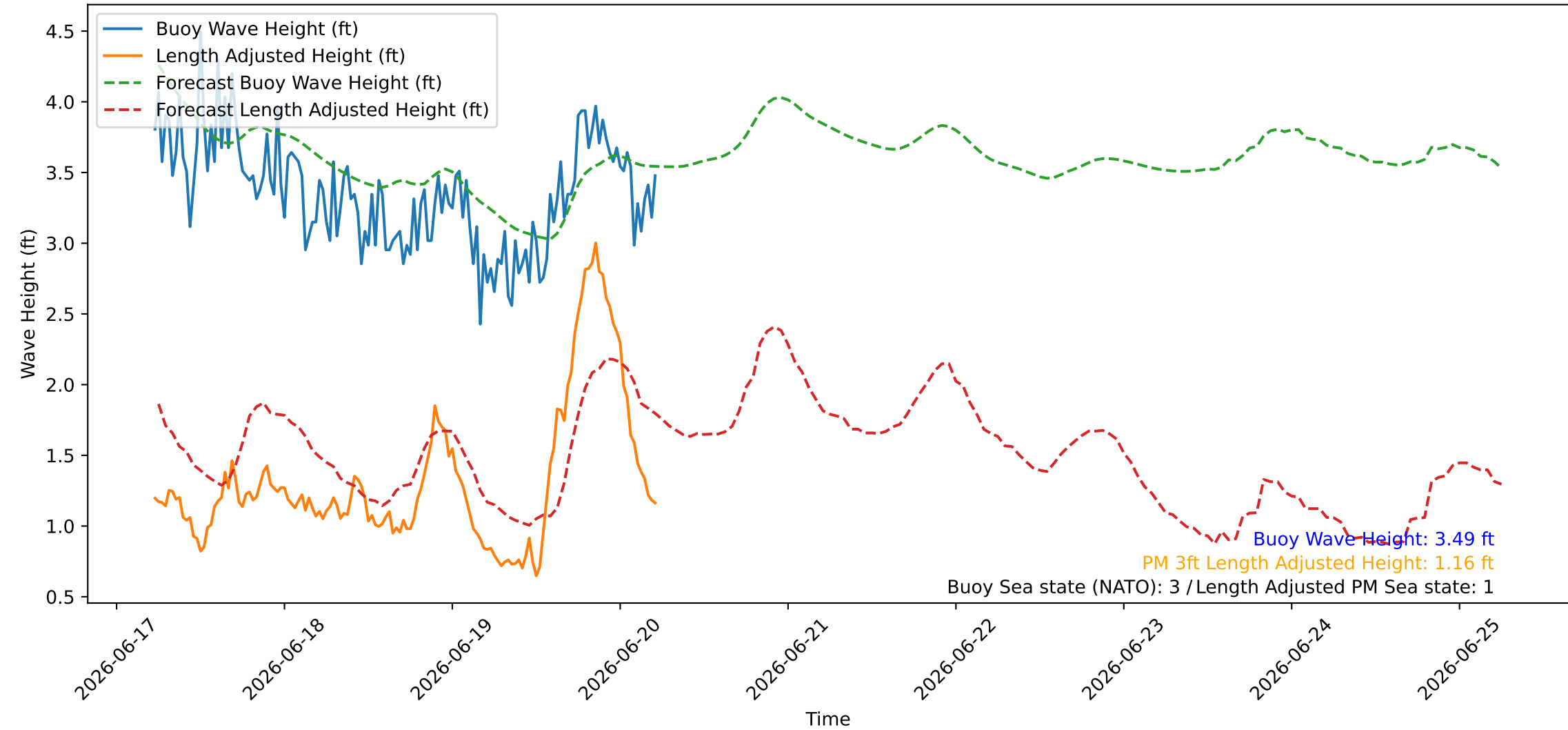
Wave Heights over Time for Green Beach at 2026-06-20 05:41:07
