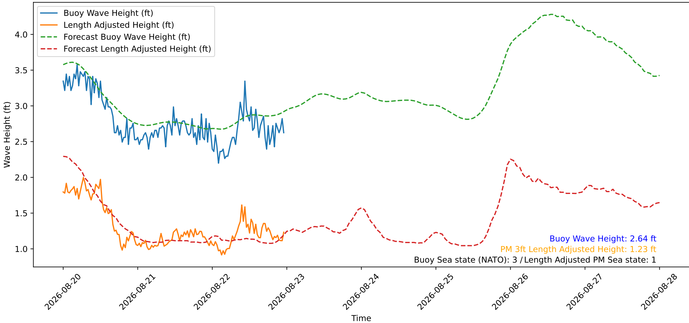
Wave Heights over Time for Oceanside Harbor at 2026-08-22 23:50:29
