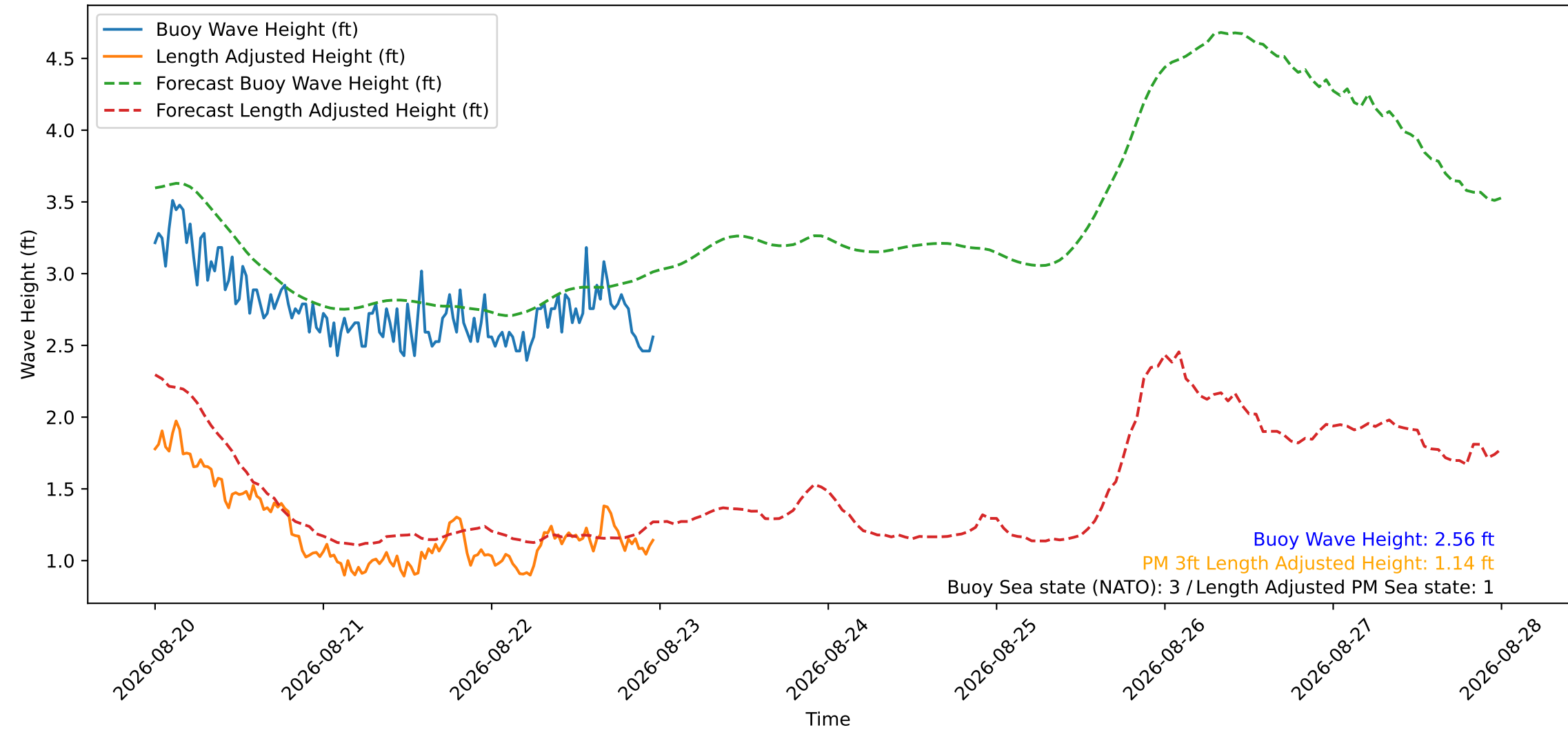
Wave Heights over Time for Green Beach at 2026-08-22 23:51:14
