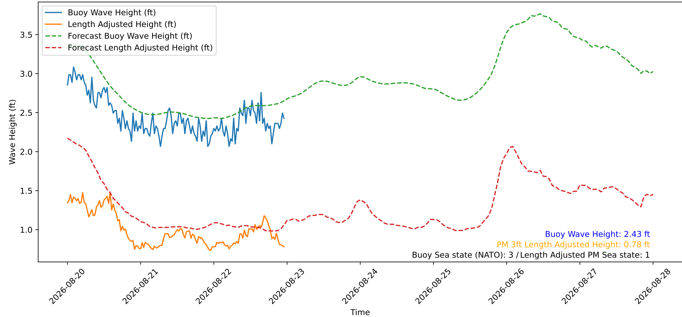
Wave Heights over Time for Red Beach at 2026-08-22 23:50:51
