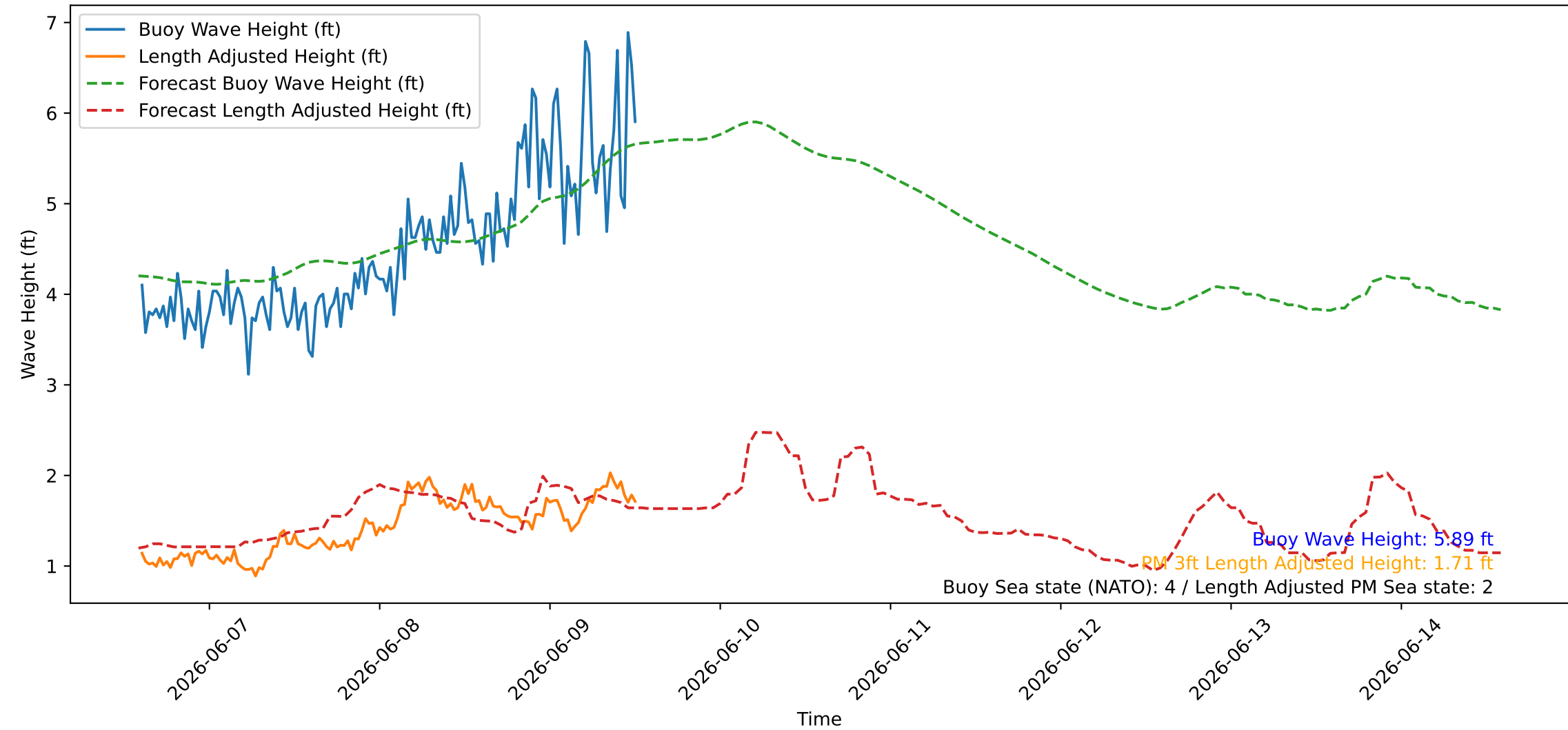
Wave Heights over Time for Green Beach at 2026-06-09 14:21:08
