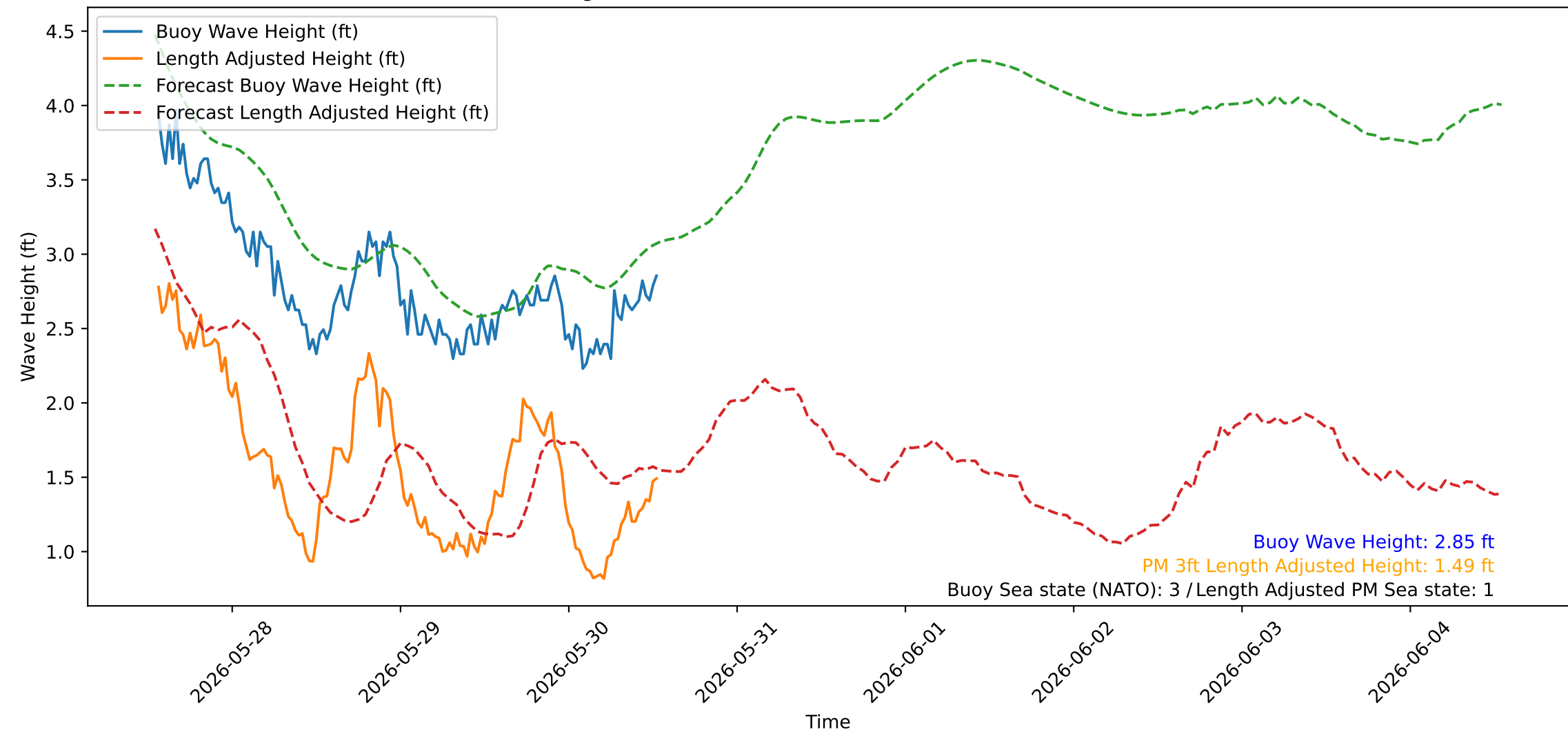
Wave Heights over Time for Red Beach at 2026-05-30 13:20:44
