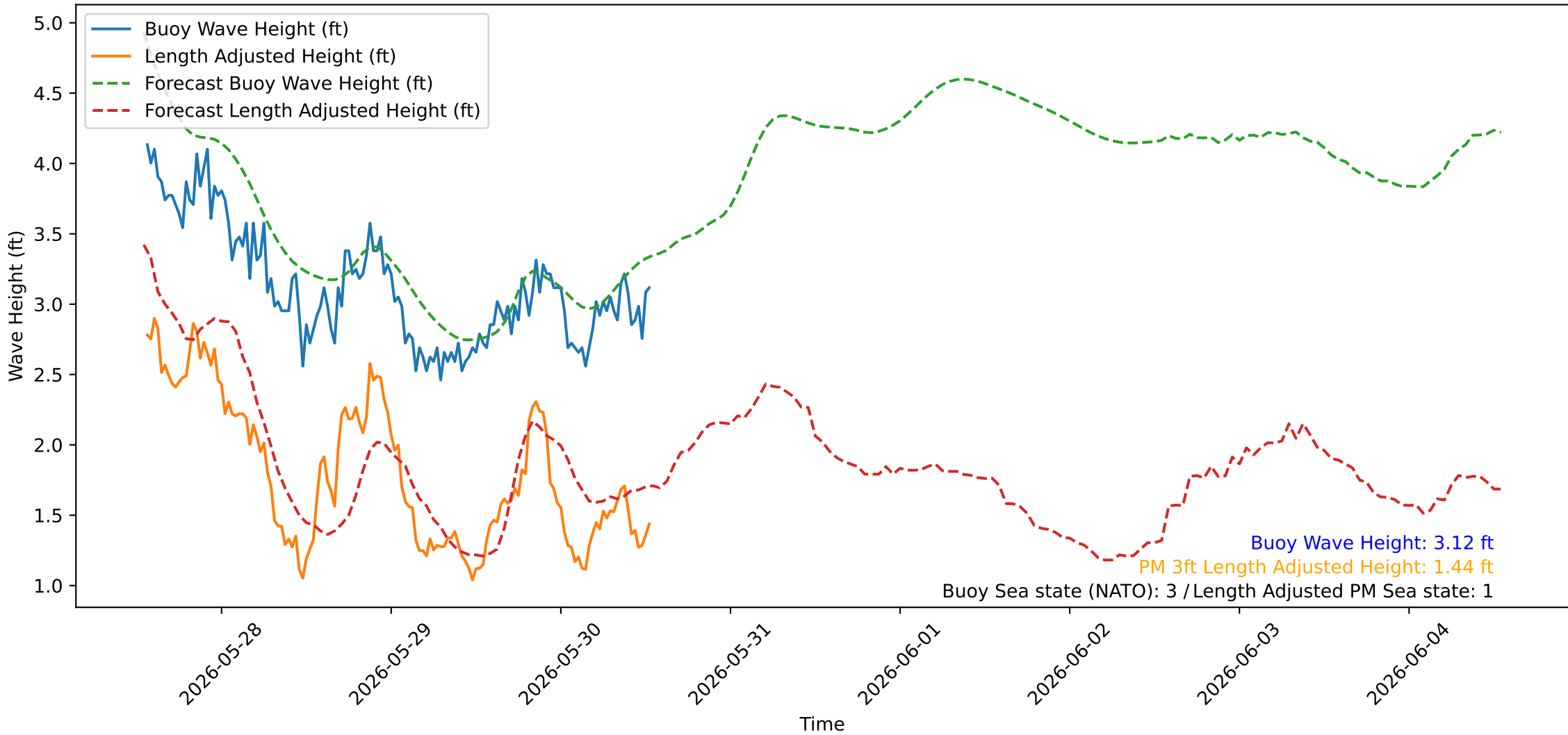
Wave Heights over Time for Green Beach at 2026-05-30 13:21:07
