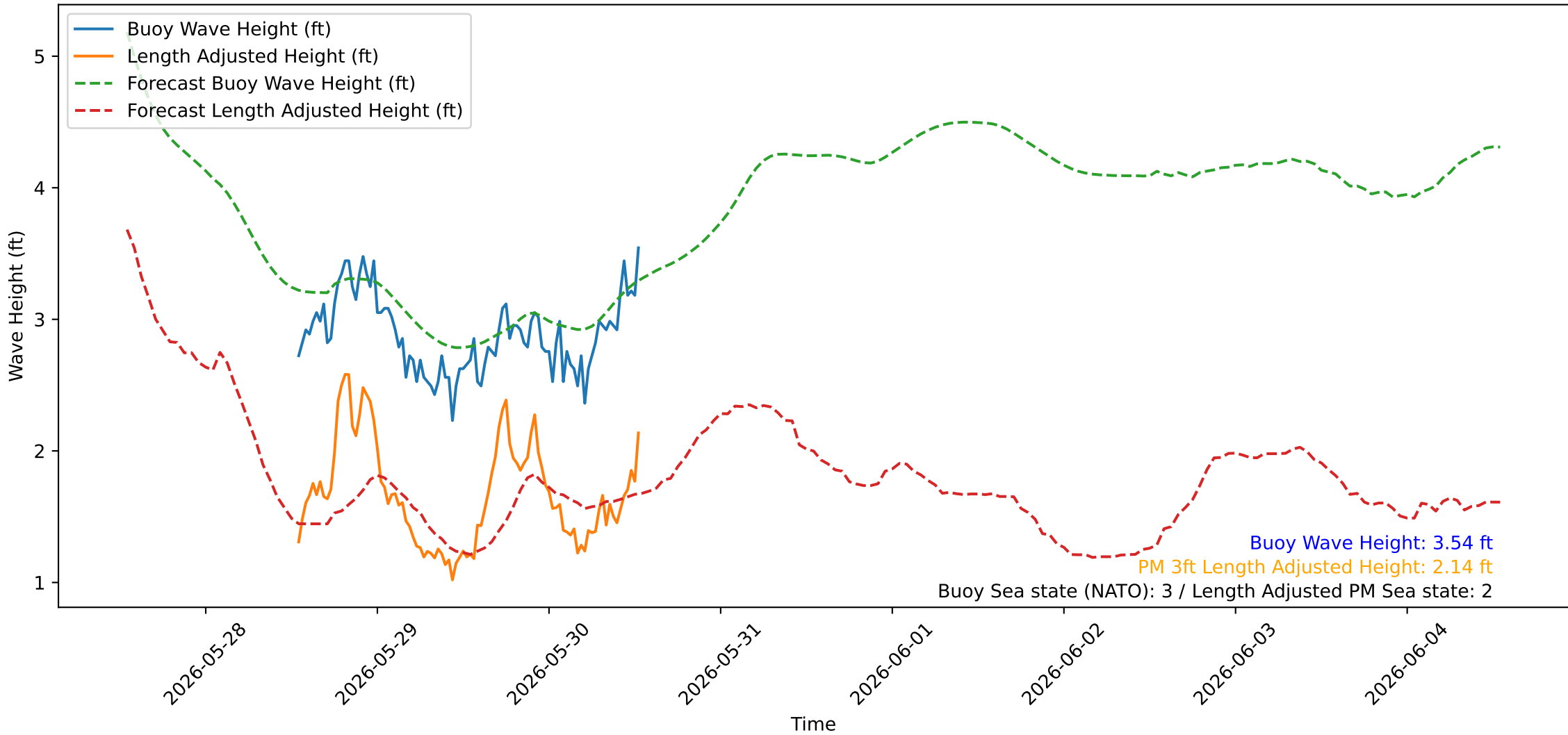
Wave Heights over Time for Oceanside Harbor at 2026-05-30 13:20:24
