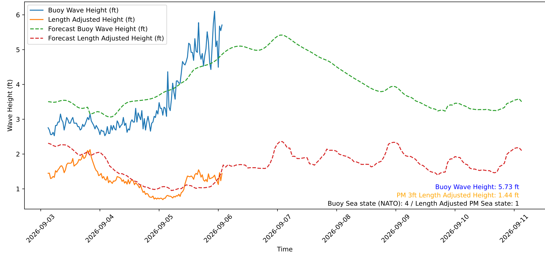
Wave Heights over Time for Red Beach at 2026-09-06 02:30:50
