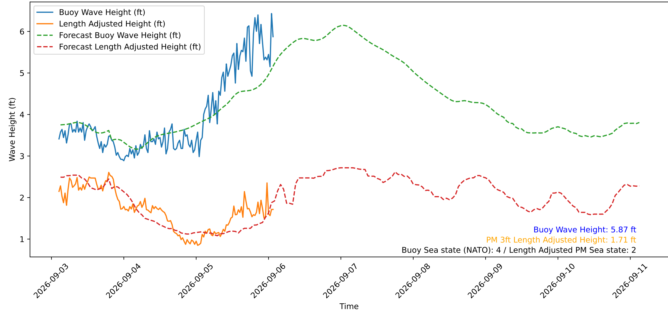
Wave Heights over Time for Oceanside Harbor at 2026-09-06 02:30:30
