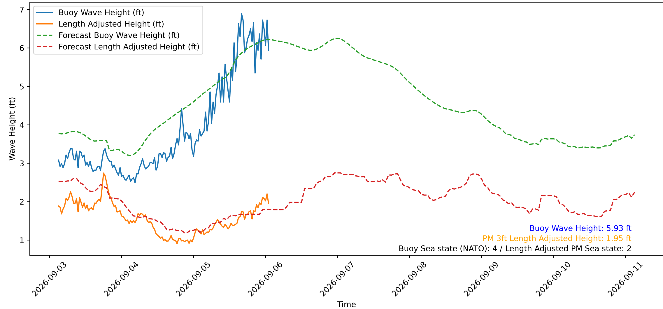
Wave Heights over Time for Green Beach at 2026-09-06 02:31:13
