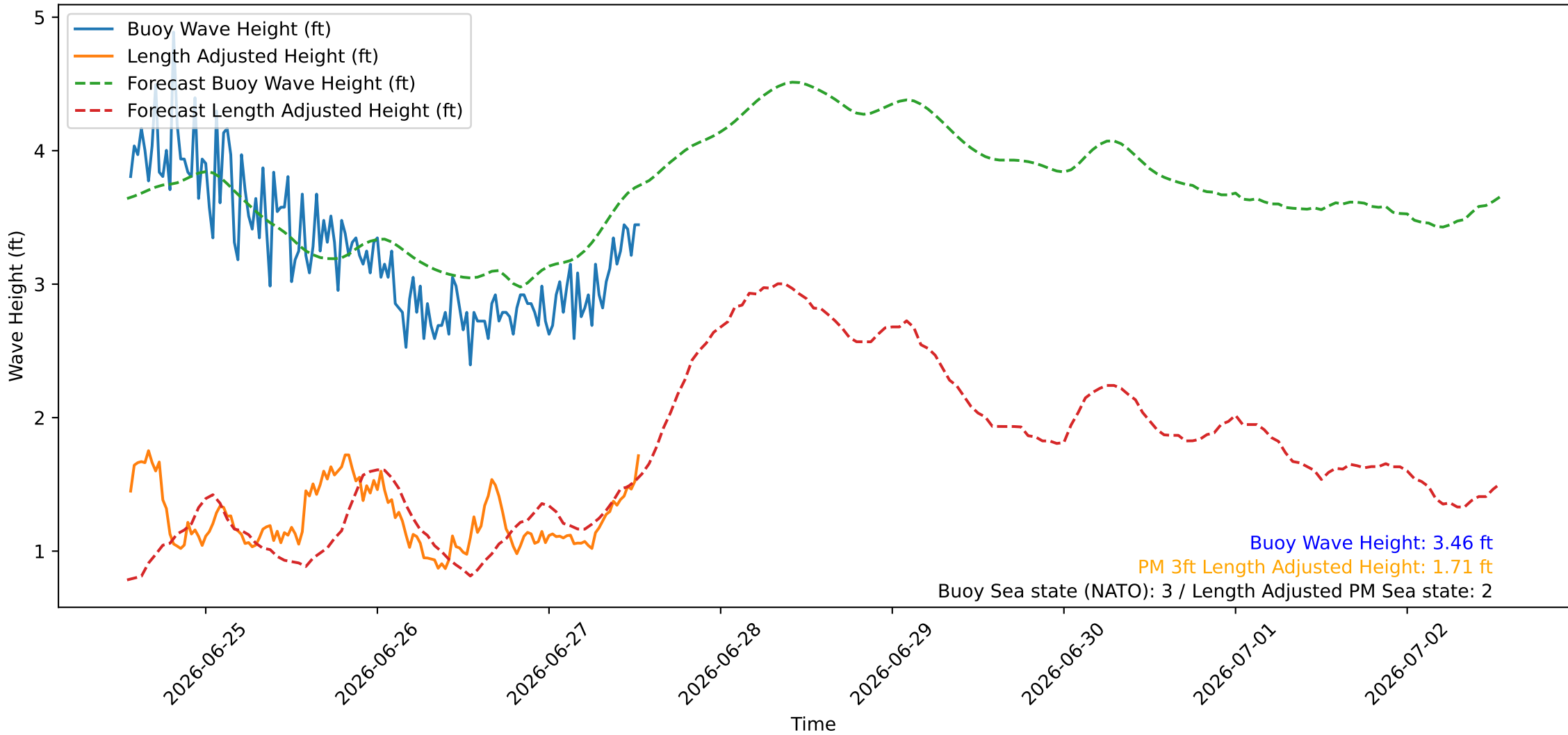
Wave Heights over Time for Oceanside Harbor at 2026-06-27 13:20:26
