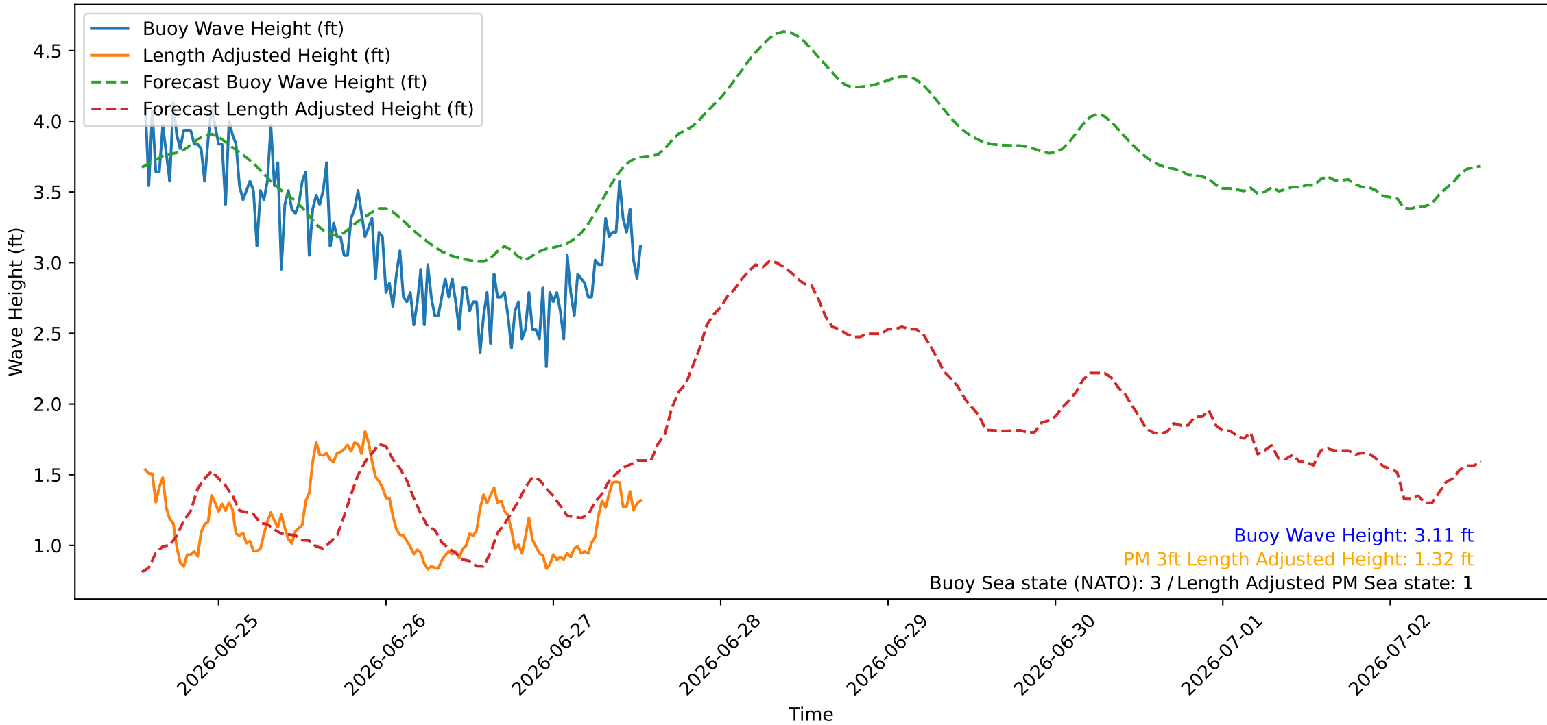
Wave Heights over Time for Green Beach at 2026-06-27 13:21:09
