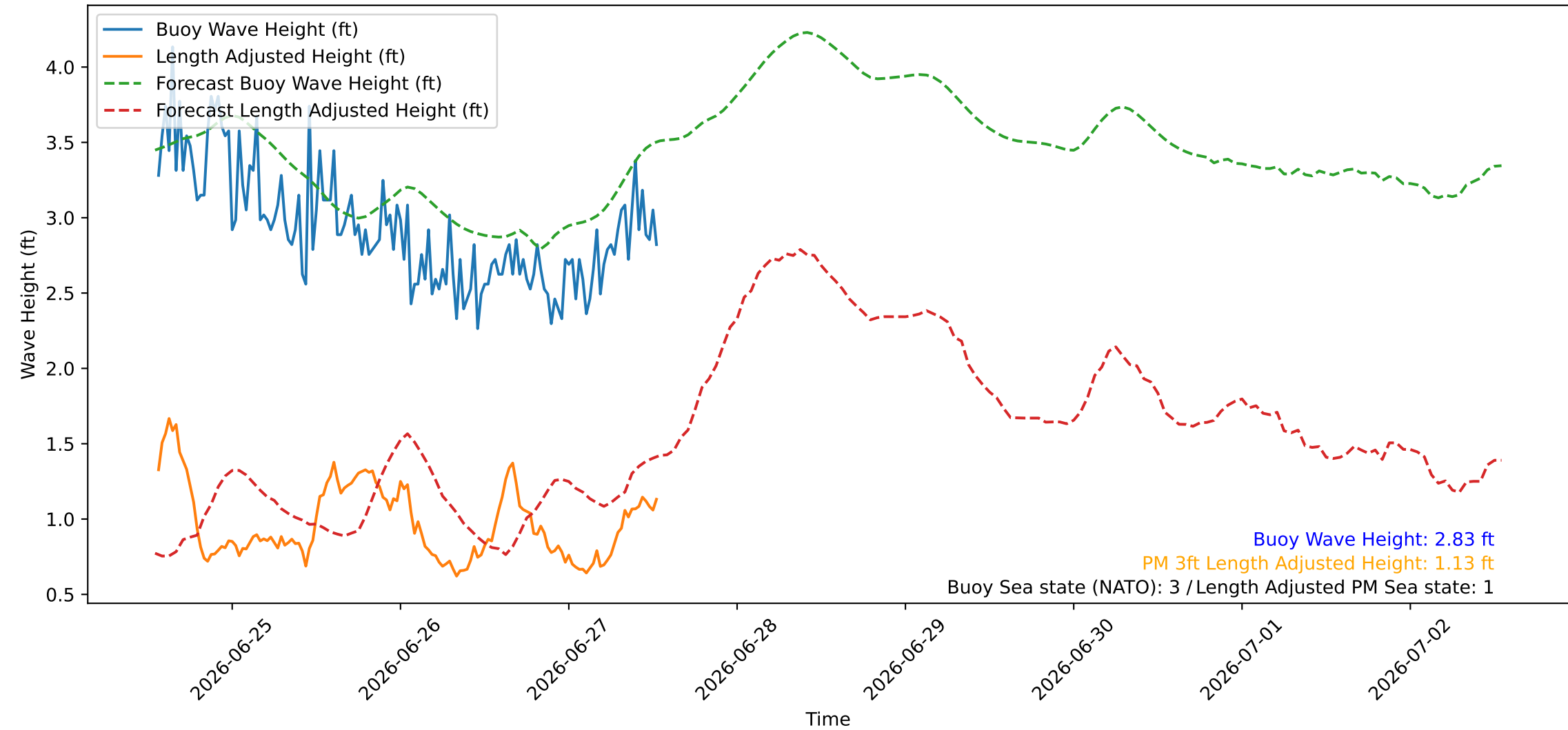
Wave Heights over Time for Red Beach at 2026-06-27 13:20:46
