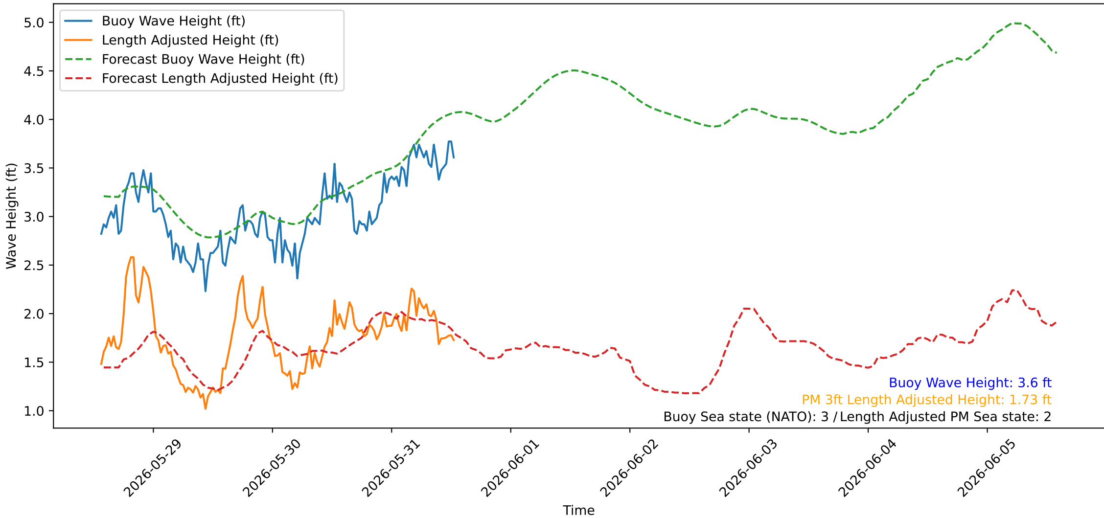
Wave Heights over Time for Oceanside Harbor at 2026-05-31 13:40:25
