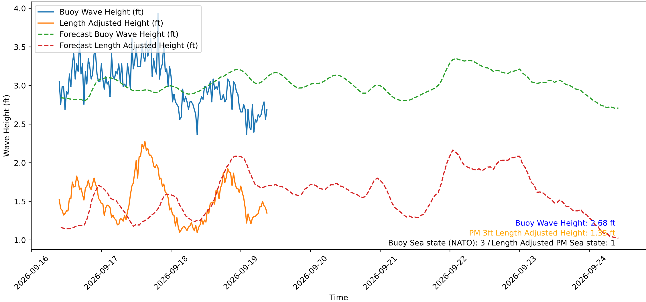
Wave Heights over Time for Oceanside Harbor at 2026-09-19 09:30:29
