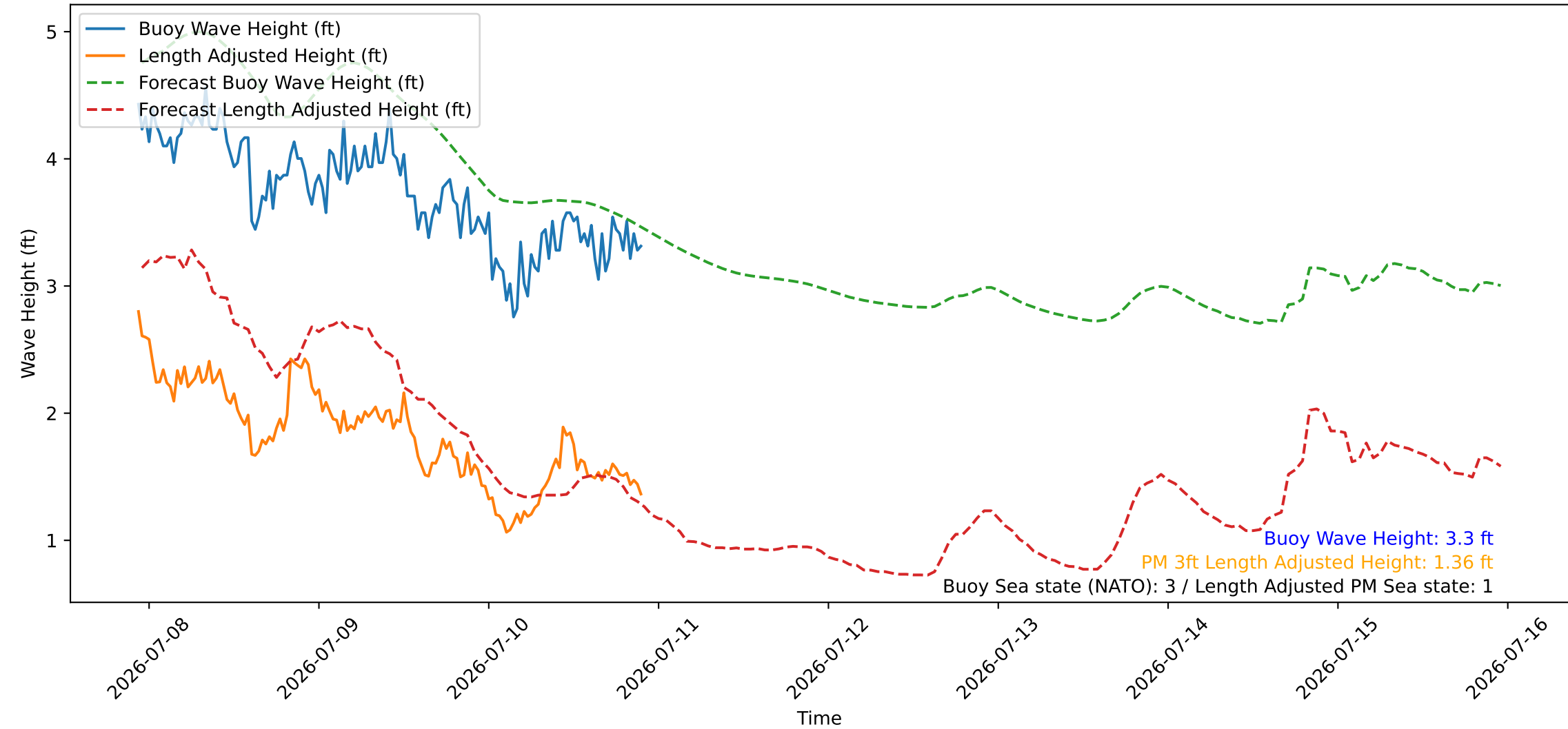
Wave Heights over Time for Green Beach at 2026-07-10 22:31:08
