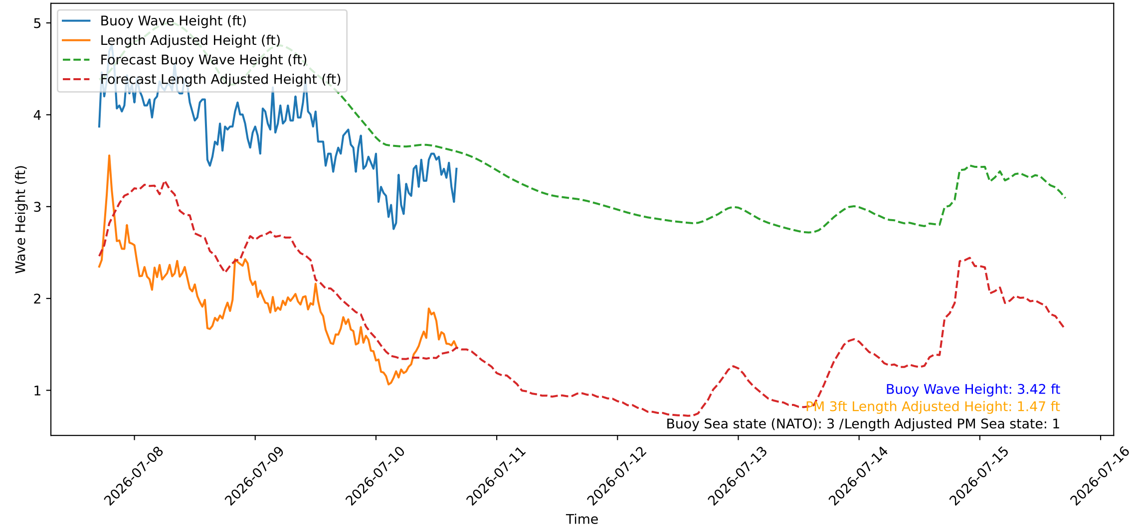
Wave Heights over Time for Green Beach at 2026-07-10 16:51:09
