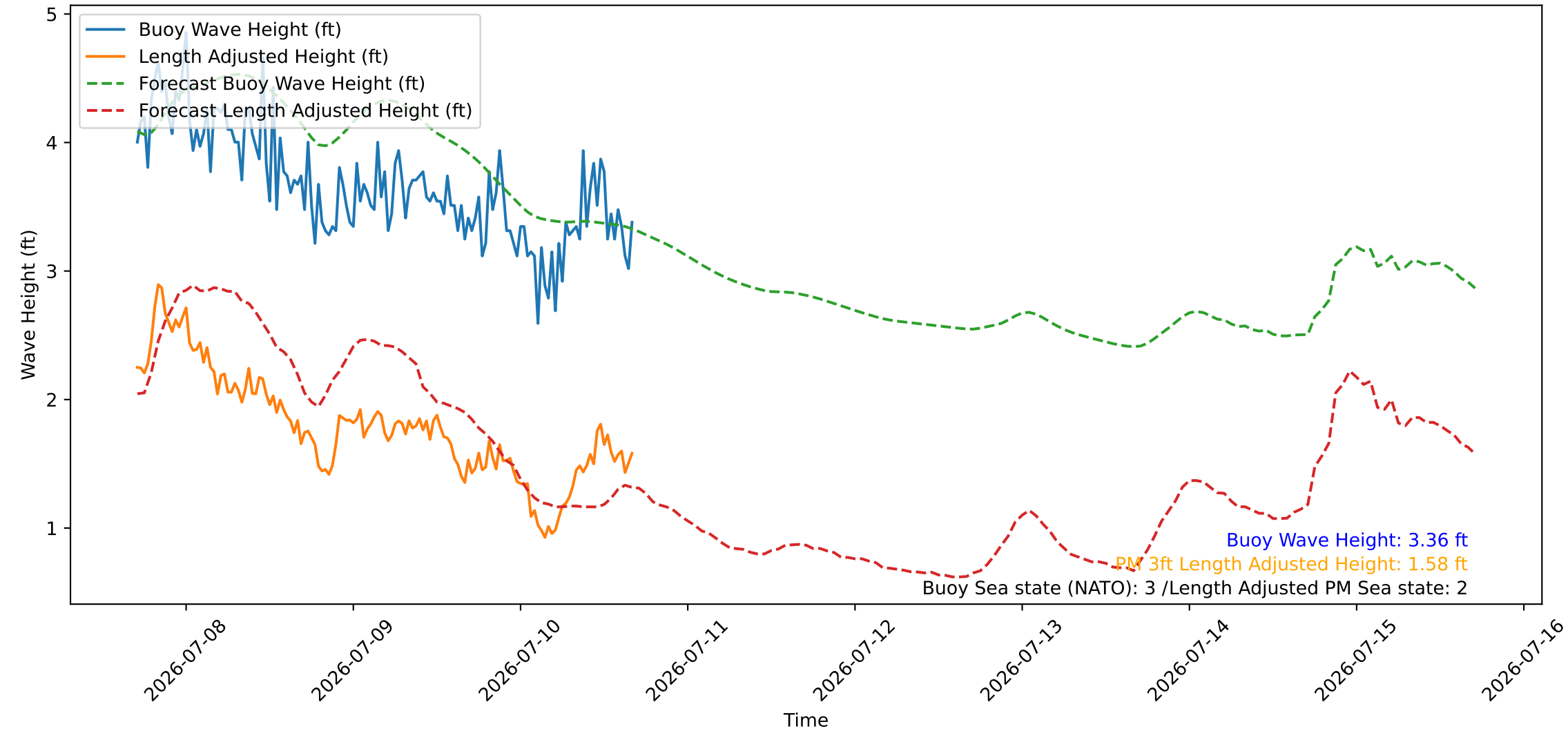
Wave Heights over Time for Red Beach at 2026-07-10 16:50:47
