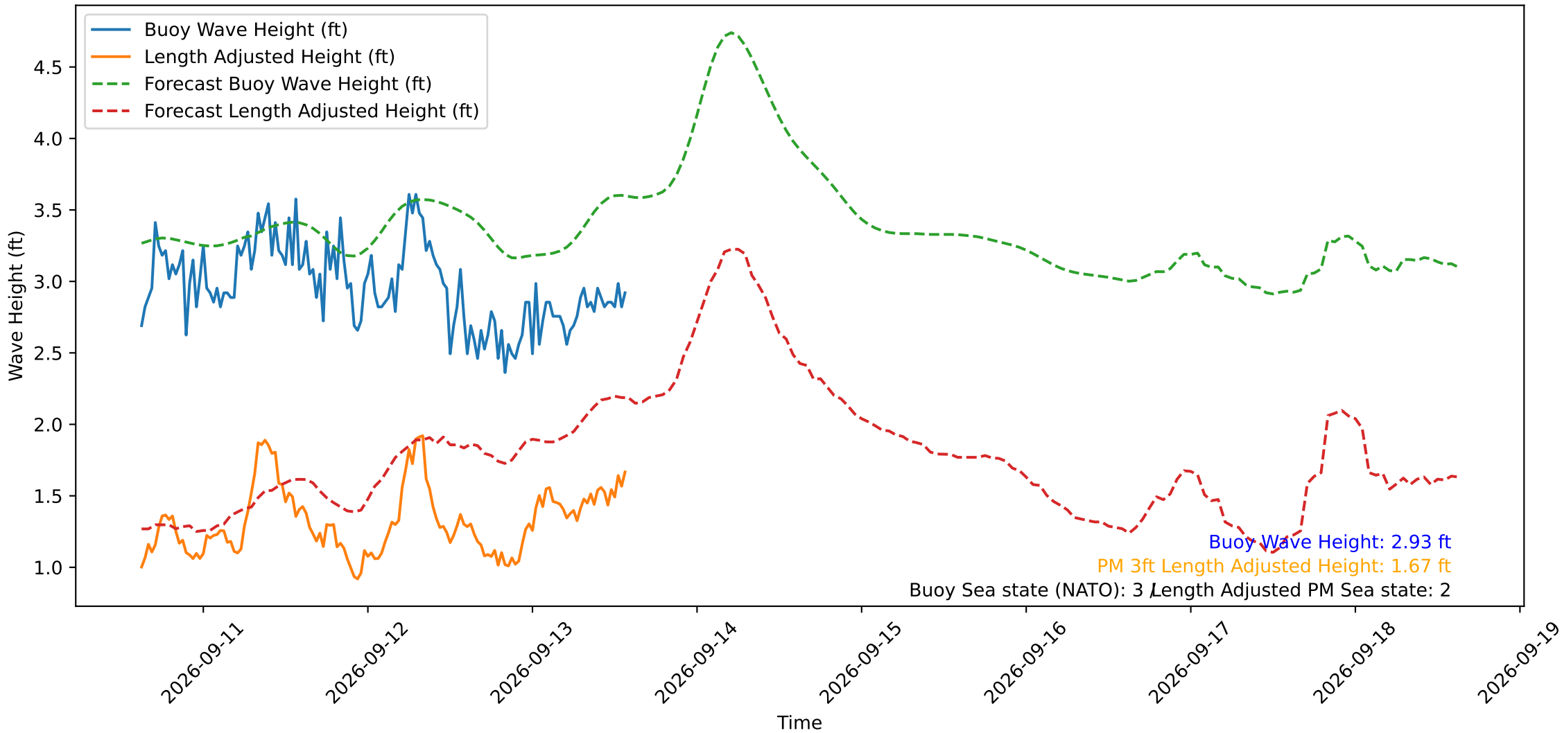
Wave Heights over Time for Green Beach at 2026-09-13 14:31:13
