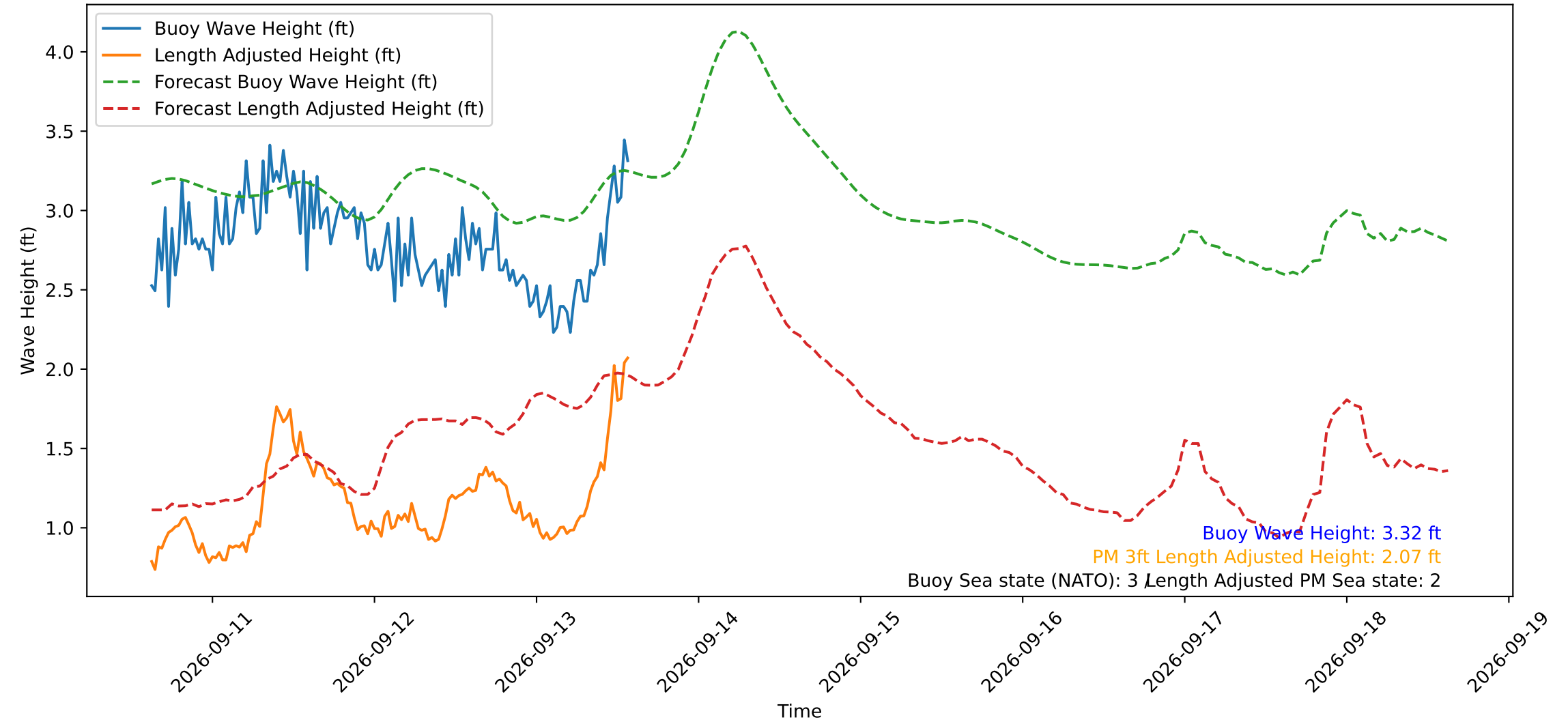
Wave Heights over Time for Red Beach at 2026-09-13 14:30:50
