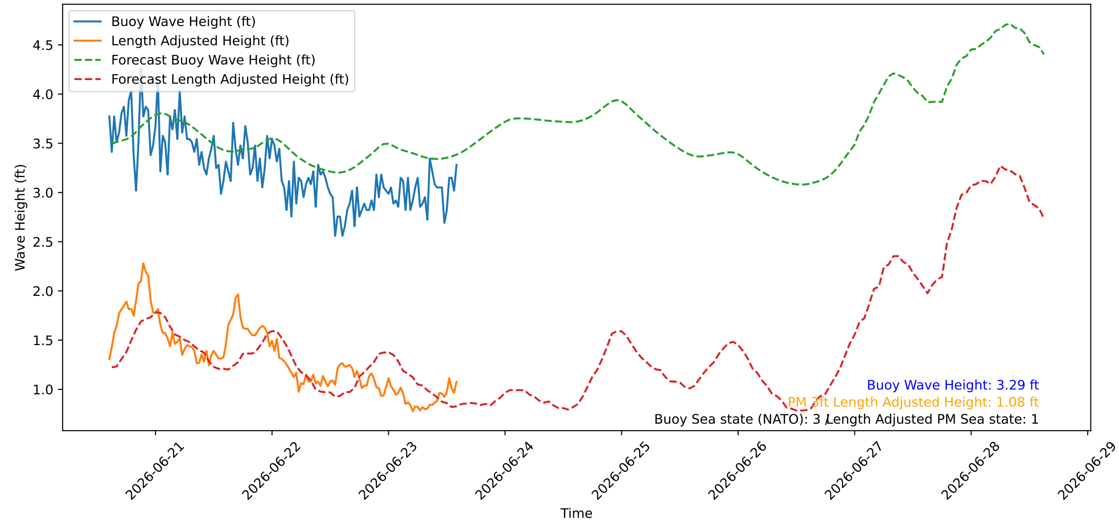
Wave Heights over Time for Oceanside Harbor at 2026-06-23 14:40:26
