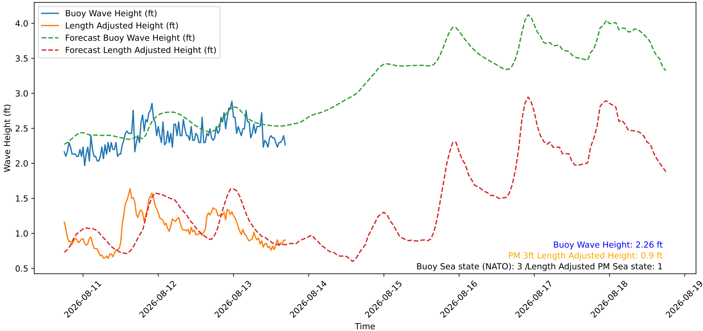
Wave Heights over Time for Red Beach at 2026-08-13 17:50:47
