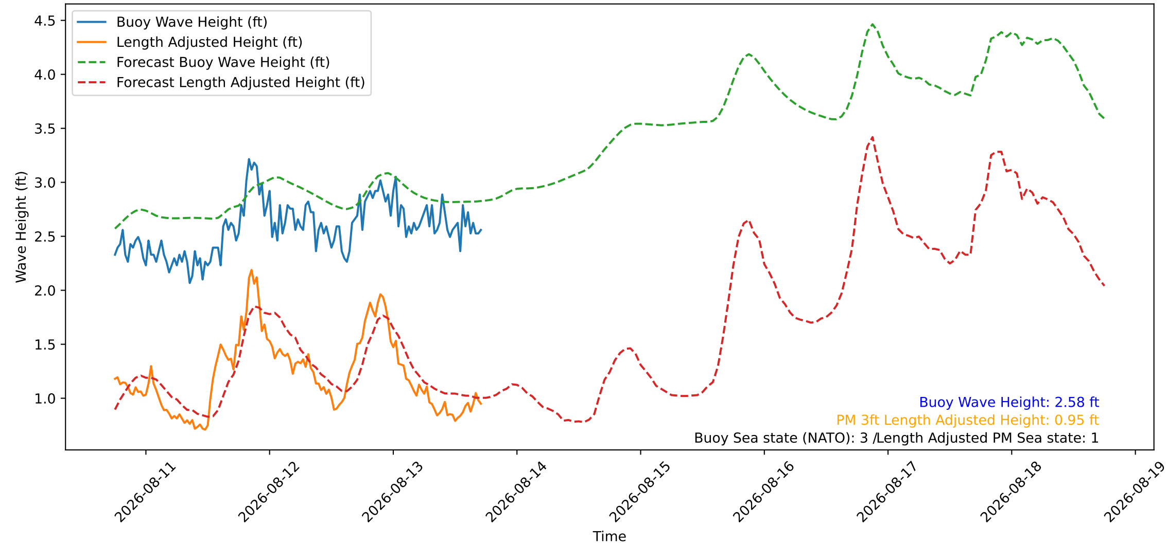
Wave Heights over Time for Green Beach at 2026-08-13 17:51:10
