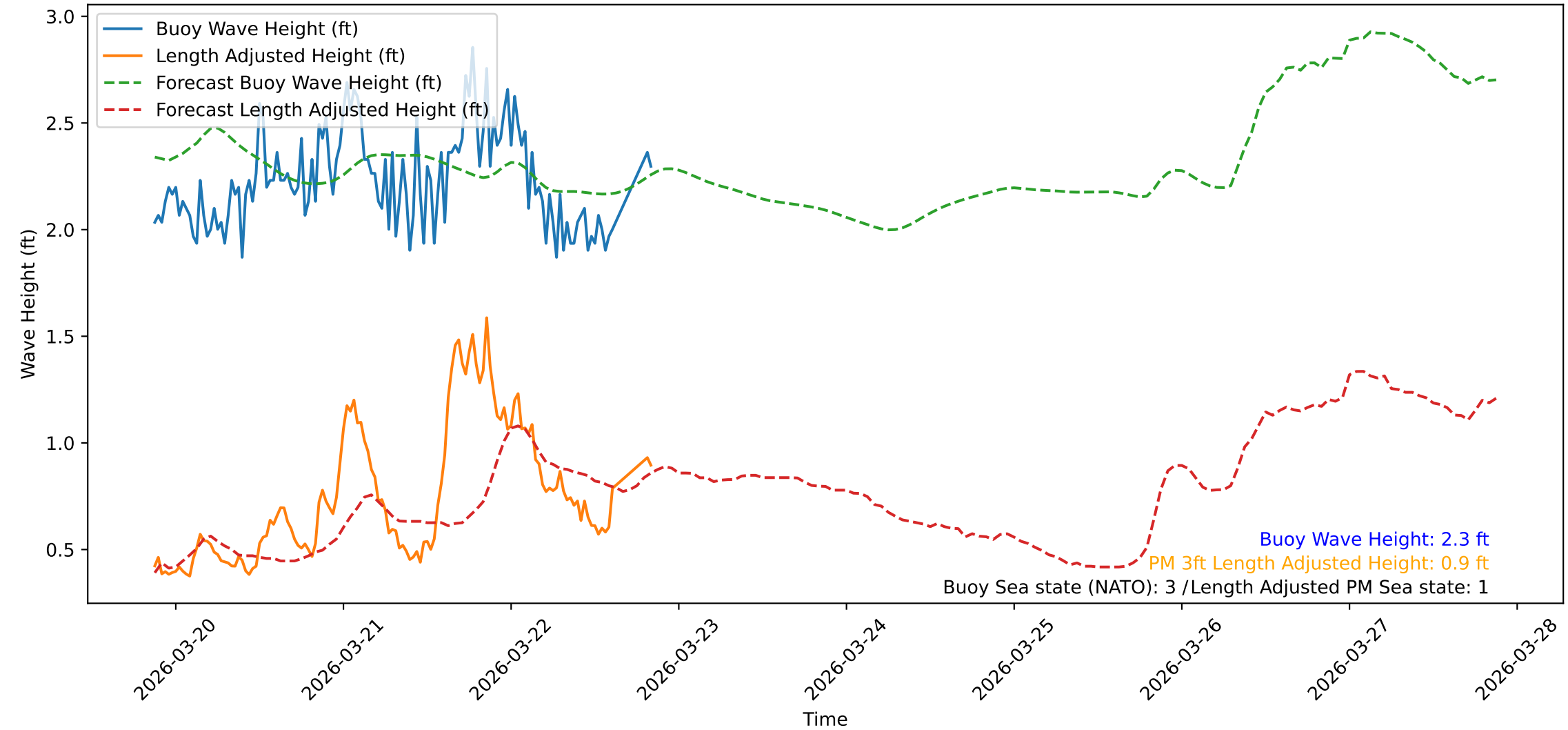
Wave Heights over Time for Red Beach at 2026-03-22 20:50:46
