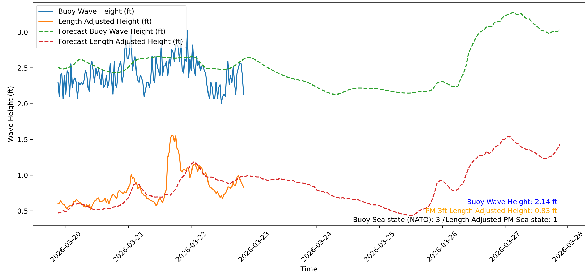
Wave Heights over Time for Oceanside Harbor at 2026-03-22 20:50:31
