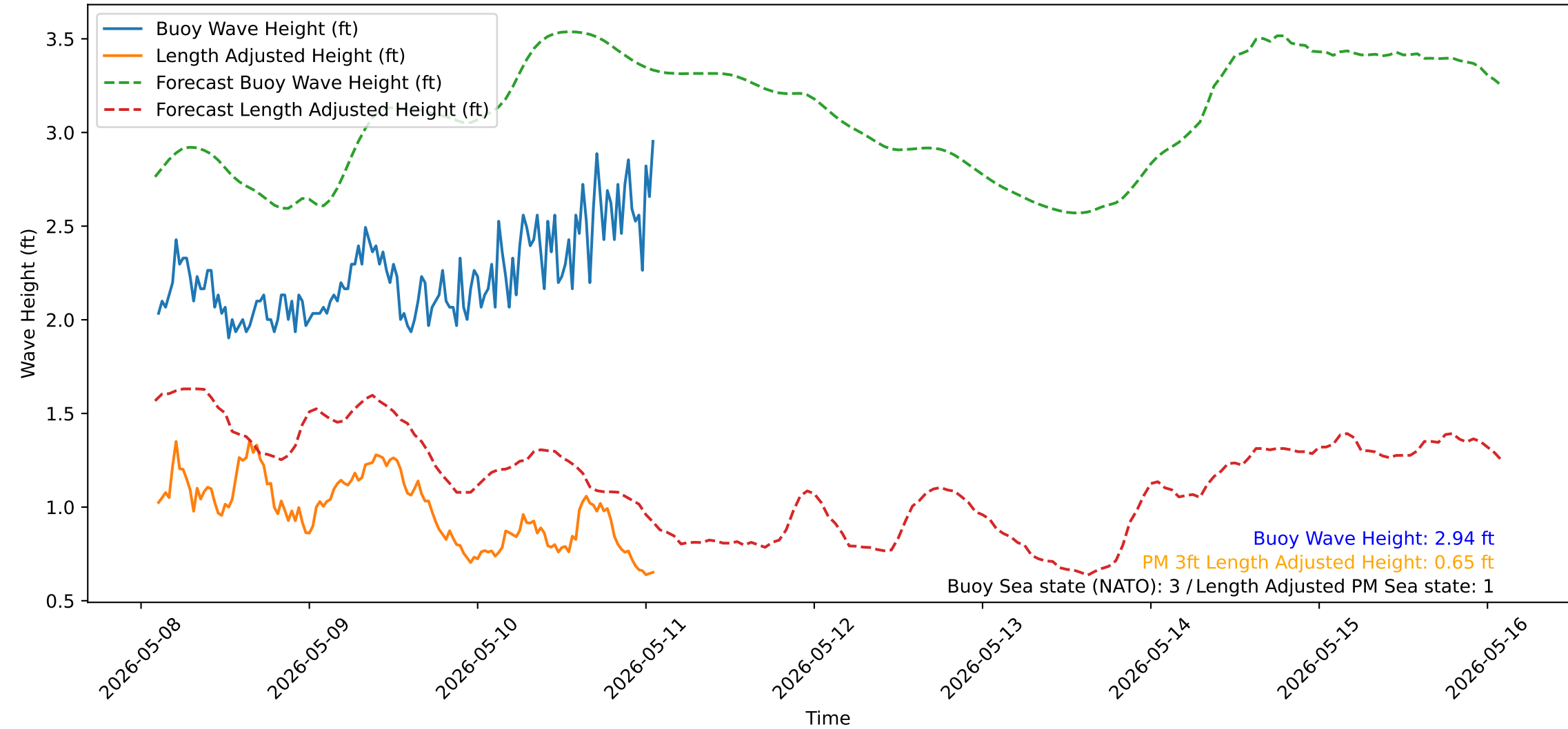
Wave Heights over Time for Red Beach at 2026-05-11 02:00:50
