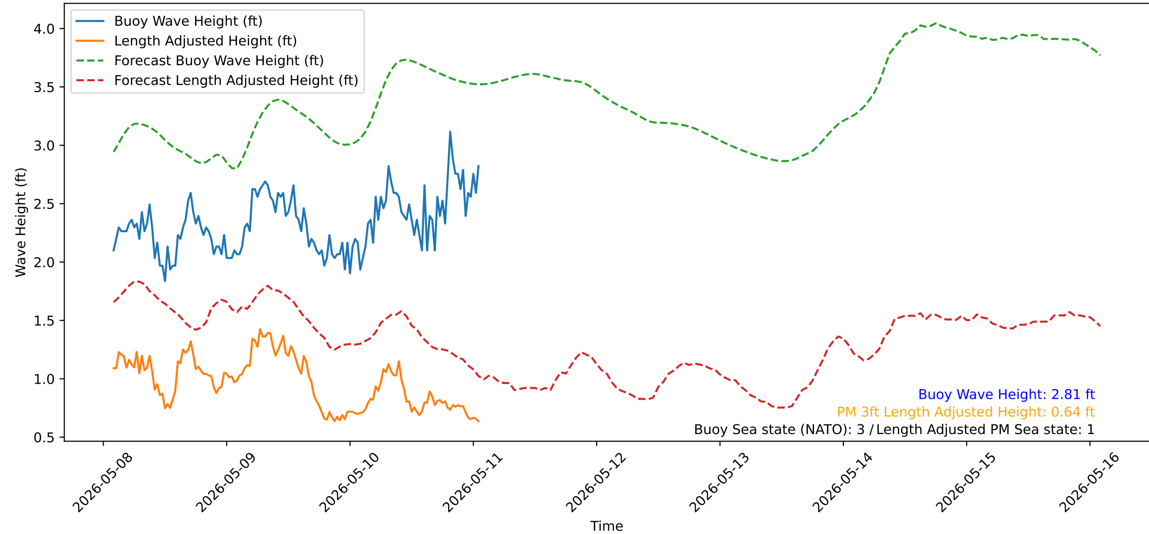
Wave Heights over Time for Green Beach at 2026-05-11 02:01:13
