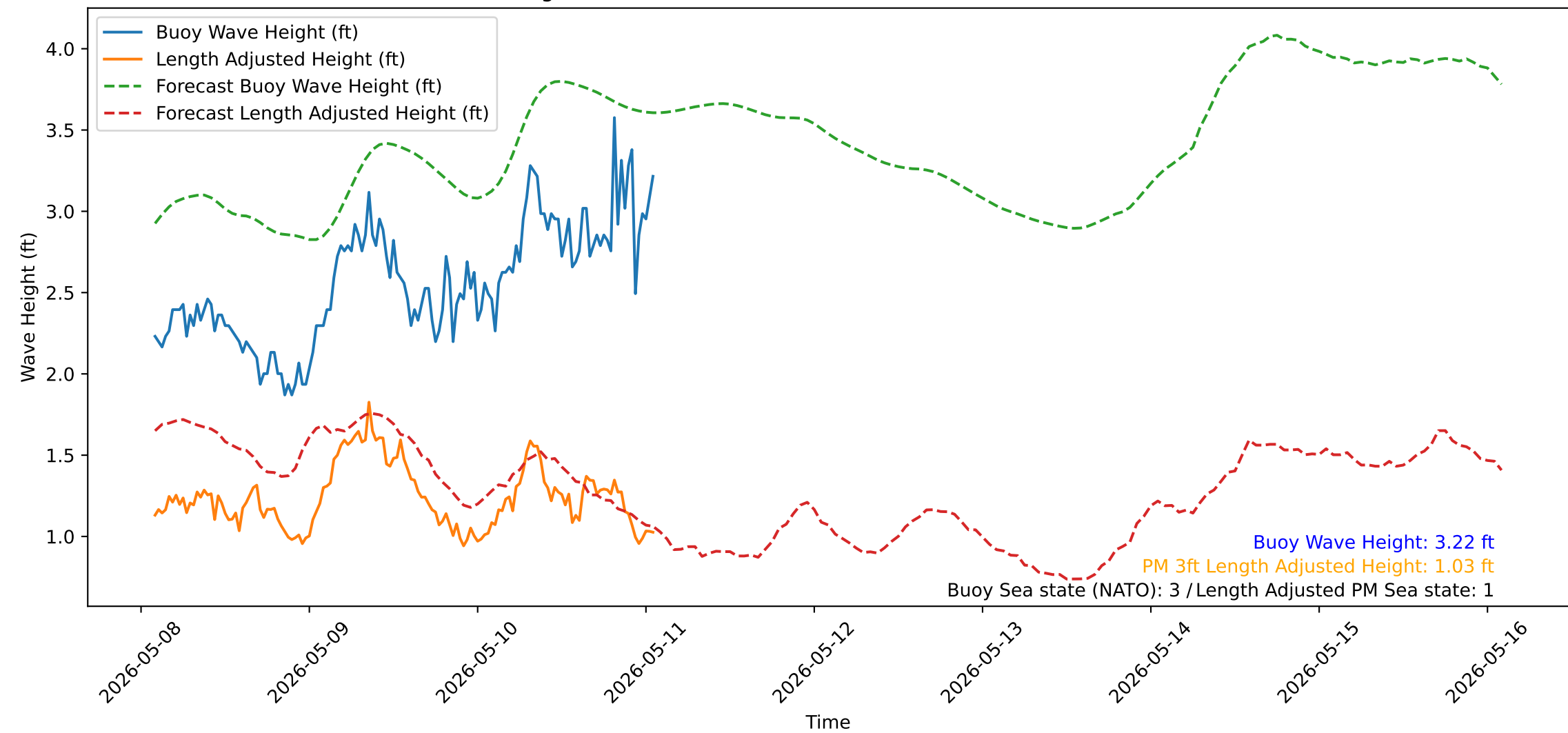
Wave Heights over Time for Oceanside Harbor at 2026-05-11 02:00:31
