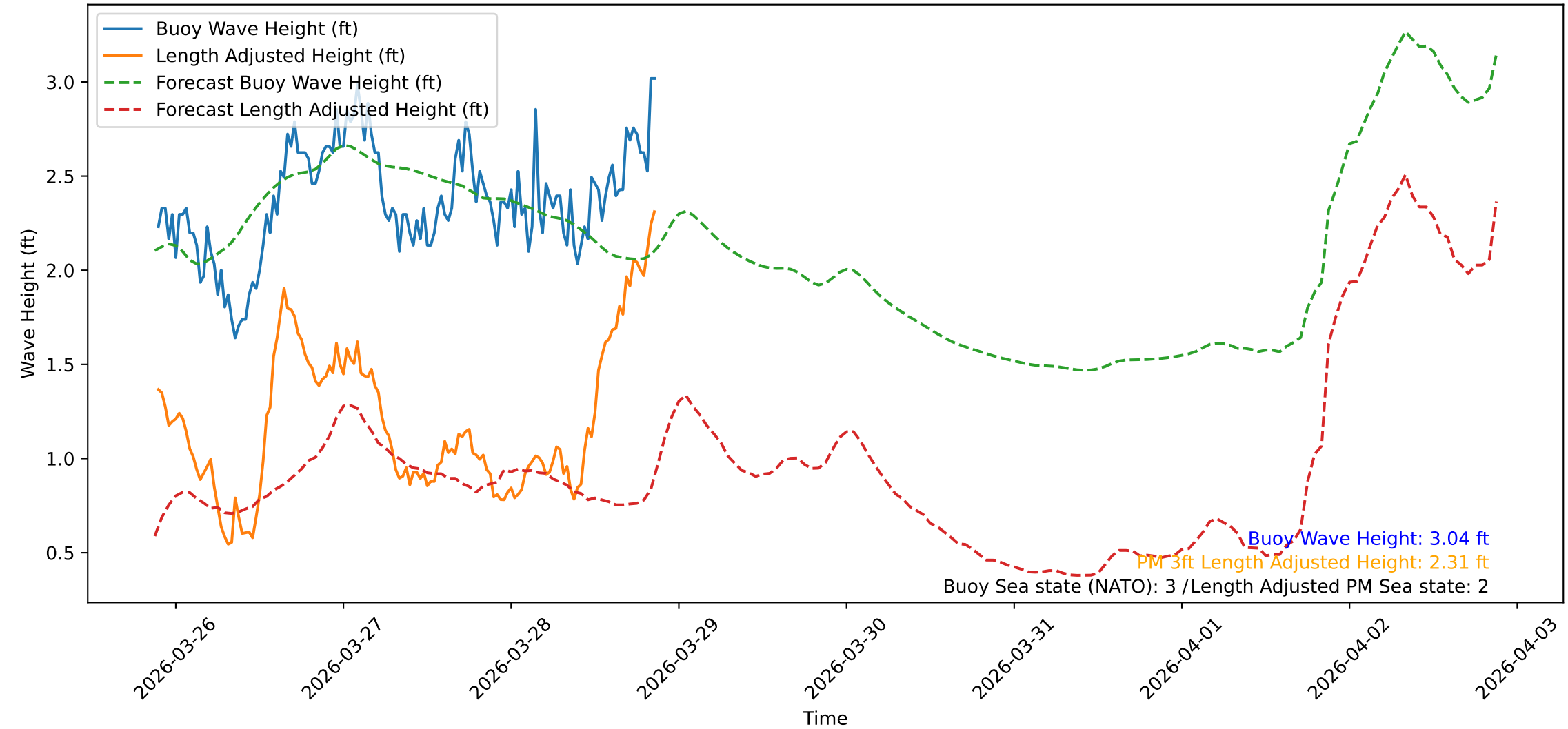
Wave Heights over Time for Red Beach at 2026-03-28 21:10:47
