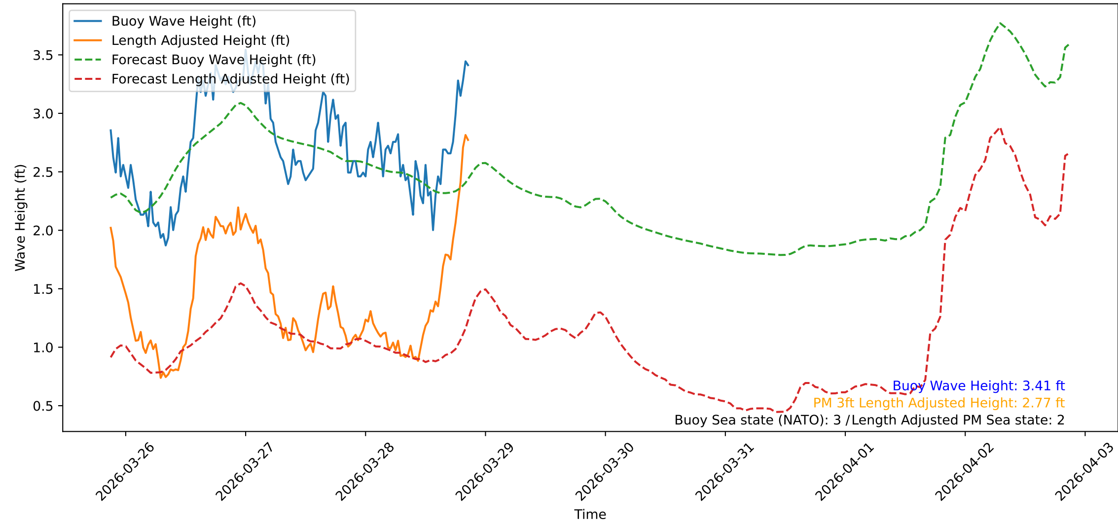
Wave Heights over Time for Green Beach at 2026-03-28 21:11:09
