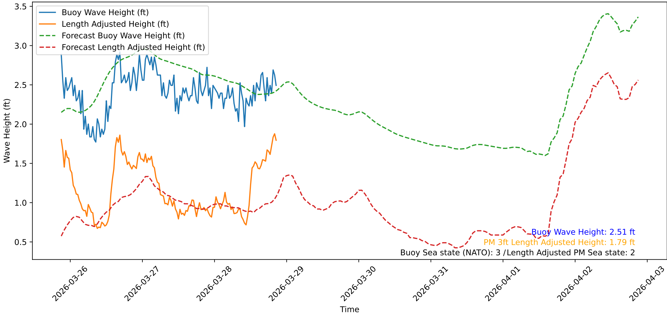
Wave Heights over Time for Oceanside Harbor at 2026-03-28 21:10:32
