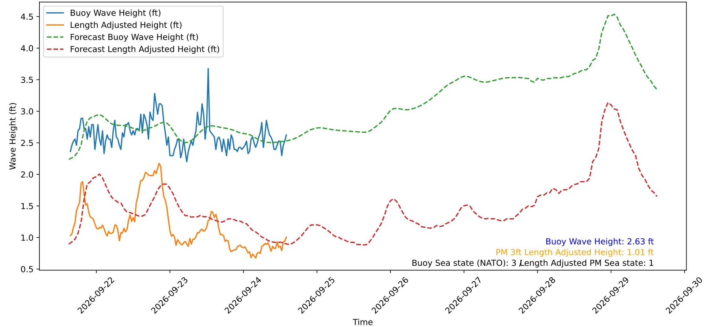
Wave Heights over Time for Red Beach at 2026-09-24 15:00:50
