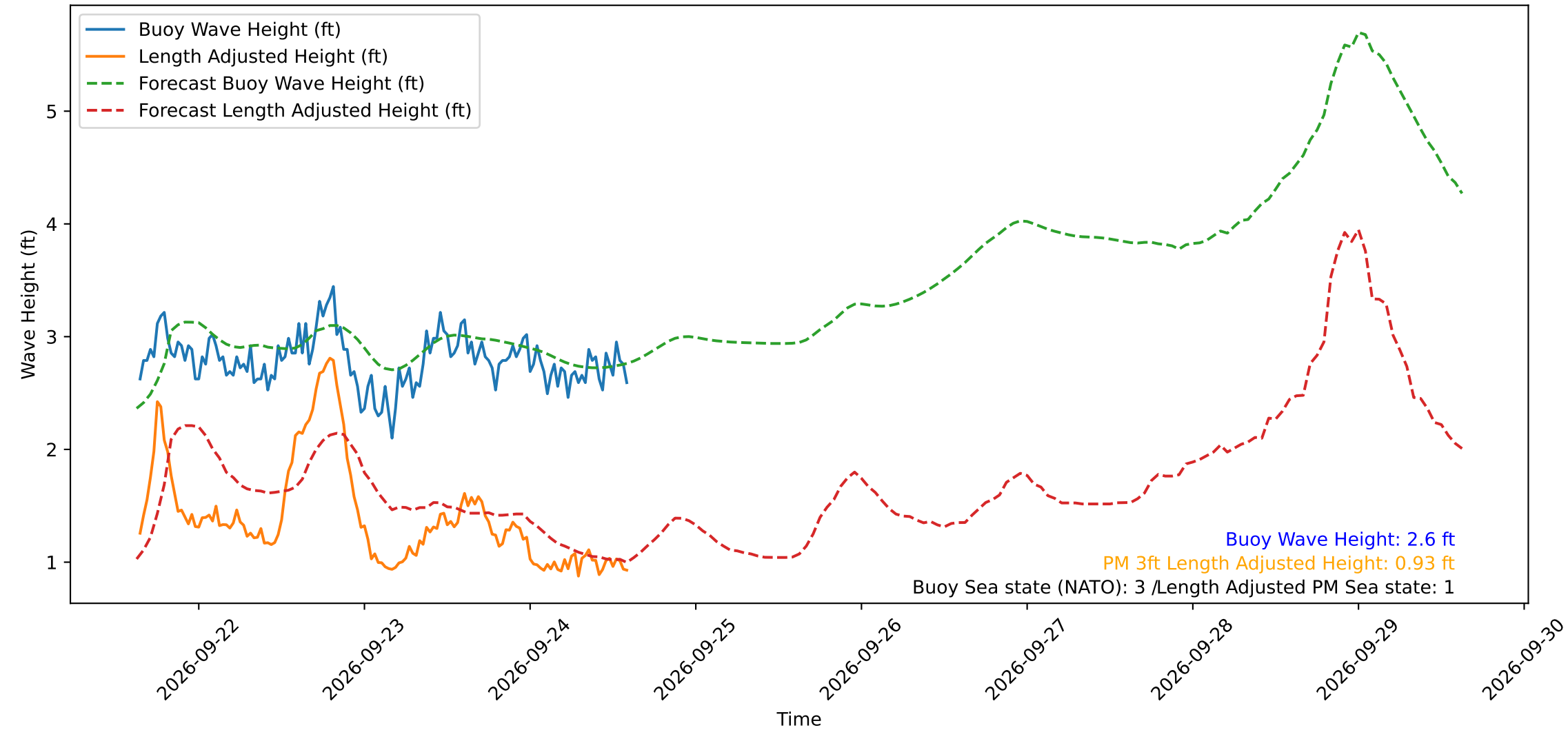
Wave Heights over Time for Green Beach at 2026-09-24 15:01:13
