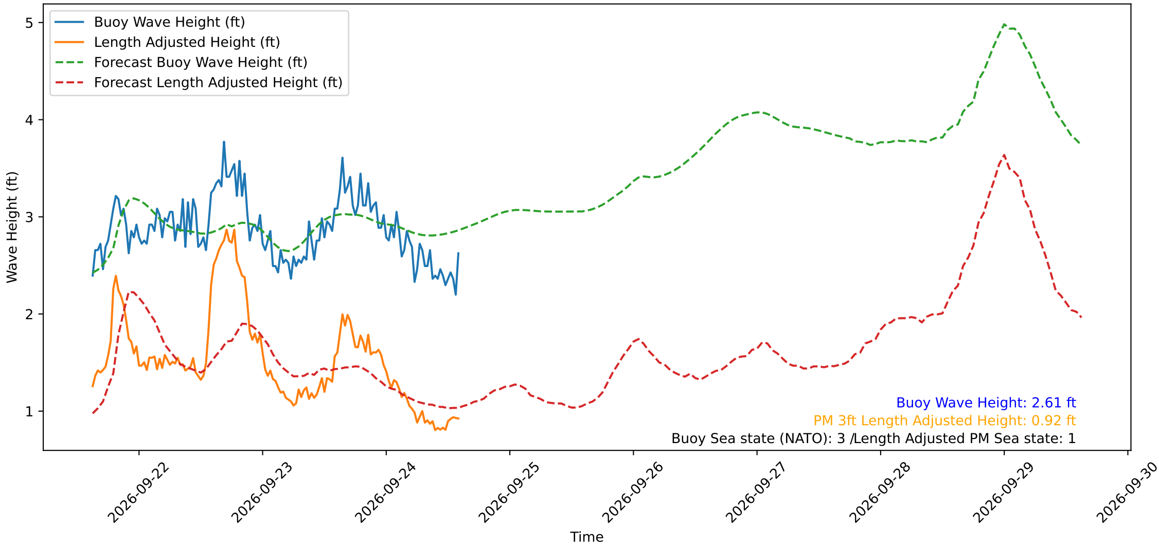
Wave Heights over Time for Oceanside Harbor at 2026-09-24 15:00:30
