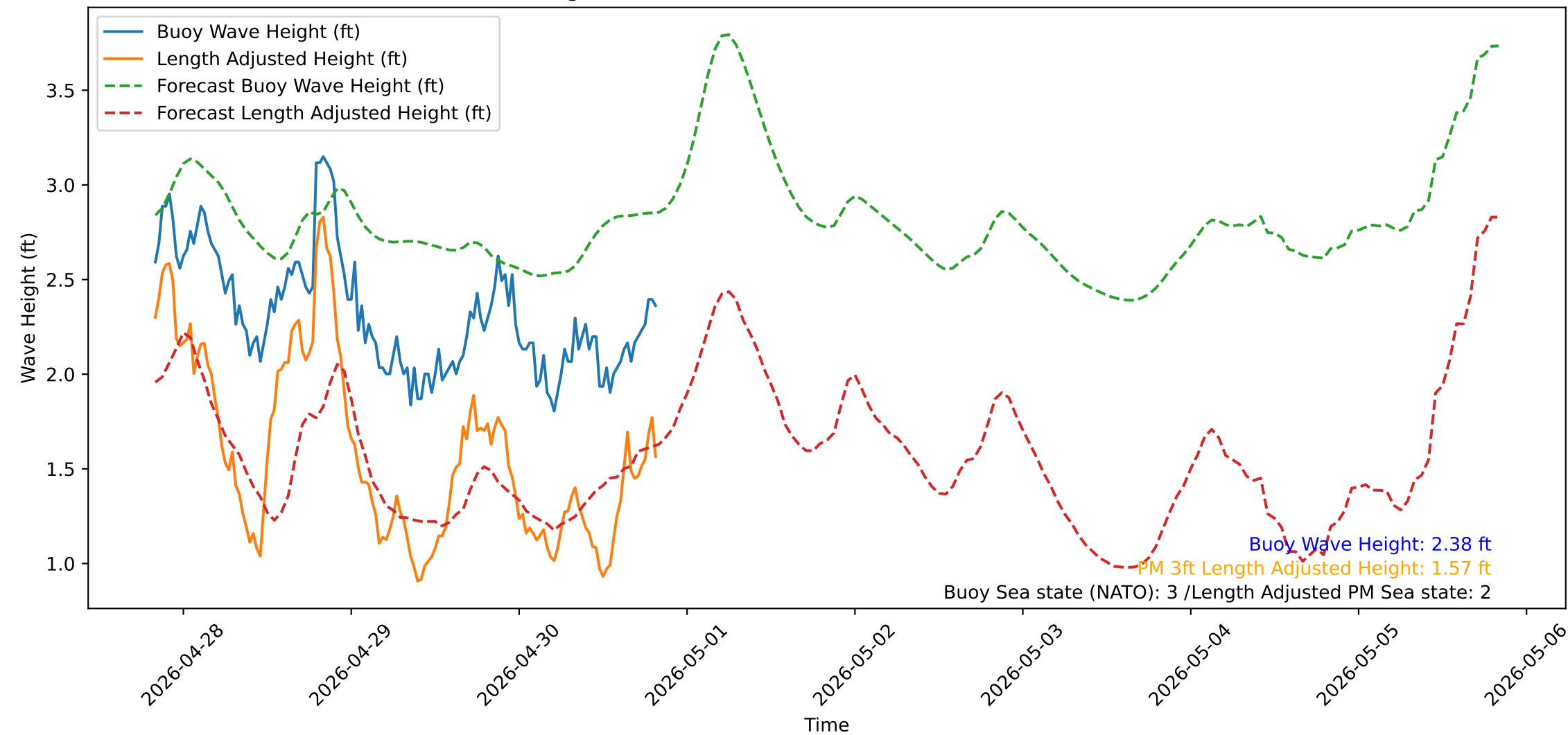
Wave Heights over Time for Green Beach at 2026-04-30 20:11:12
