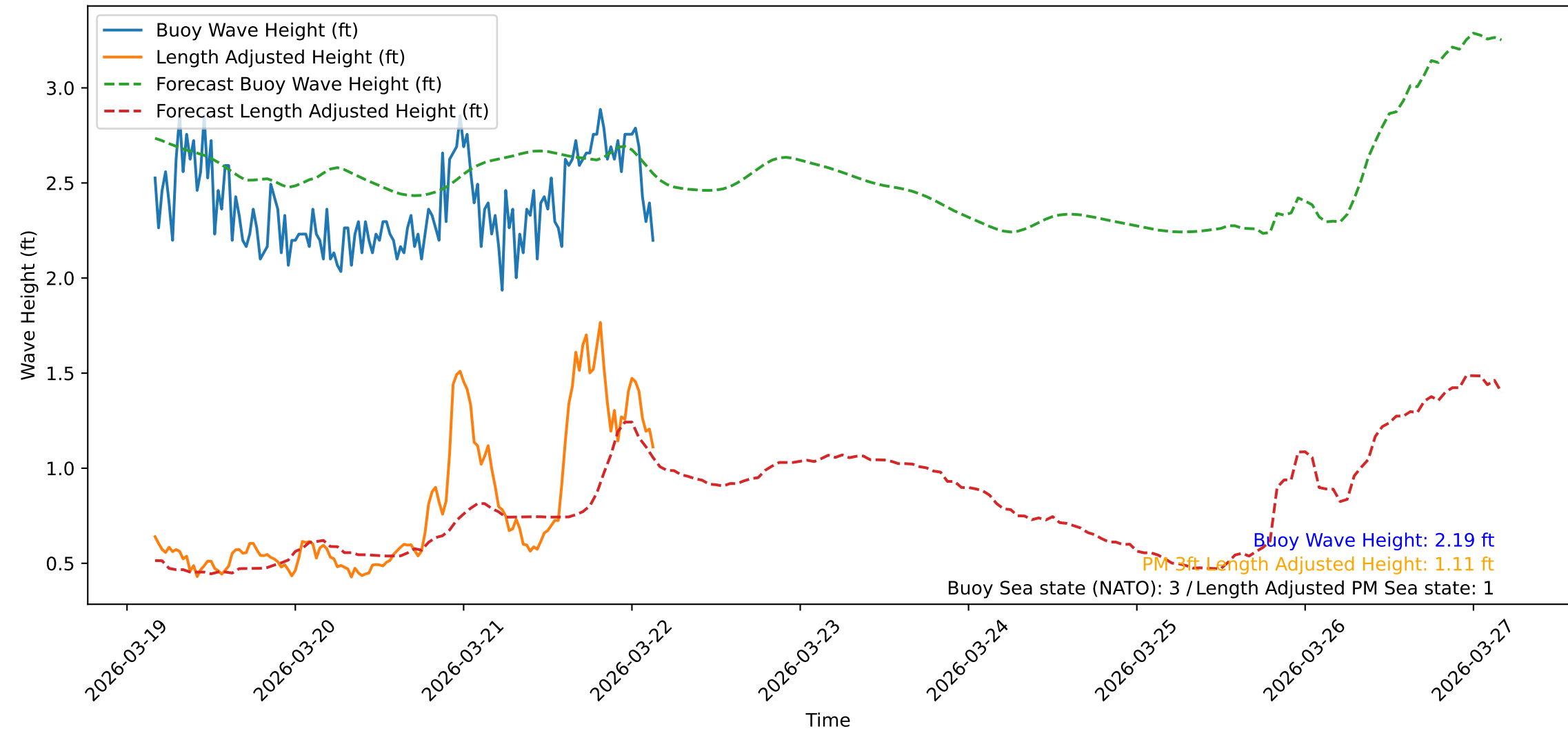
Wave Heights over Time for Green Beach at 2026-03-22 04:11:09
