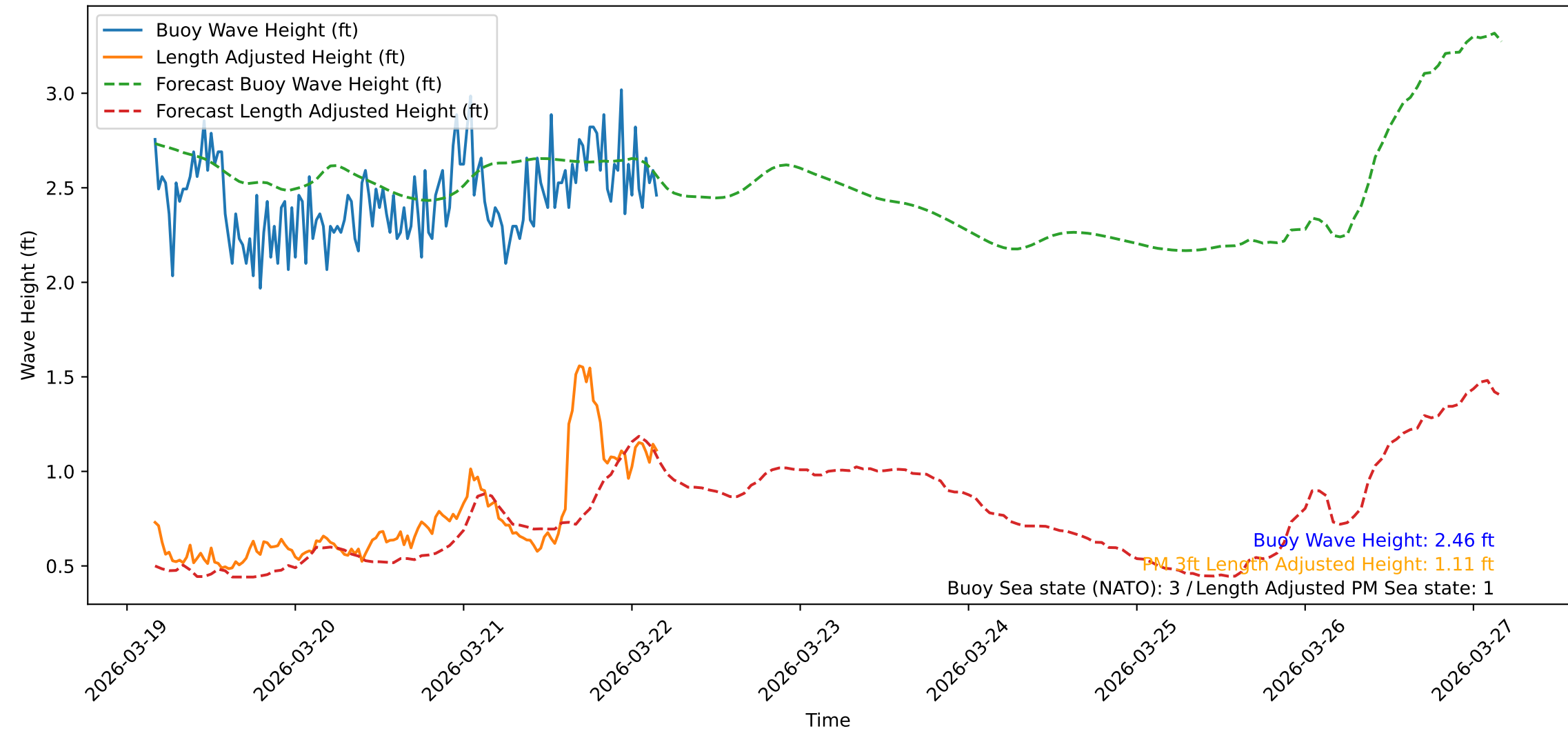
Wave Heights over Time for Oceanside Harbor at 2026-03-22 04:10:31
