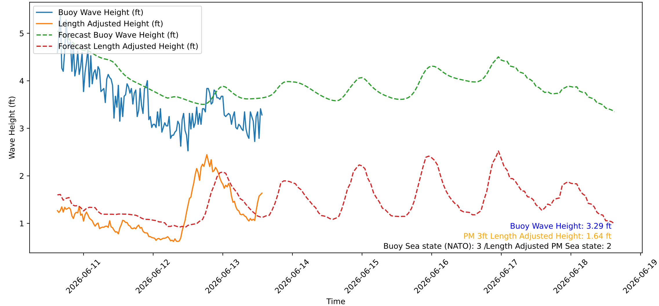
Wave Heights over Time for Red Beach at 2026-06-13 14:30:46
