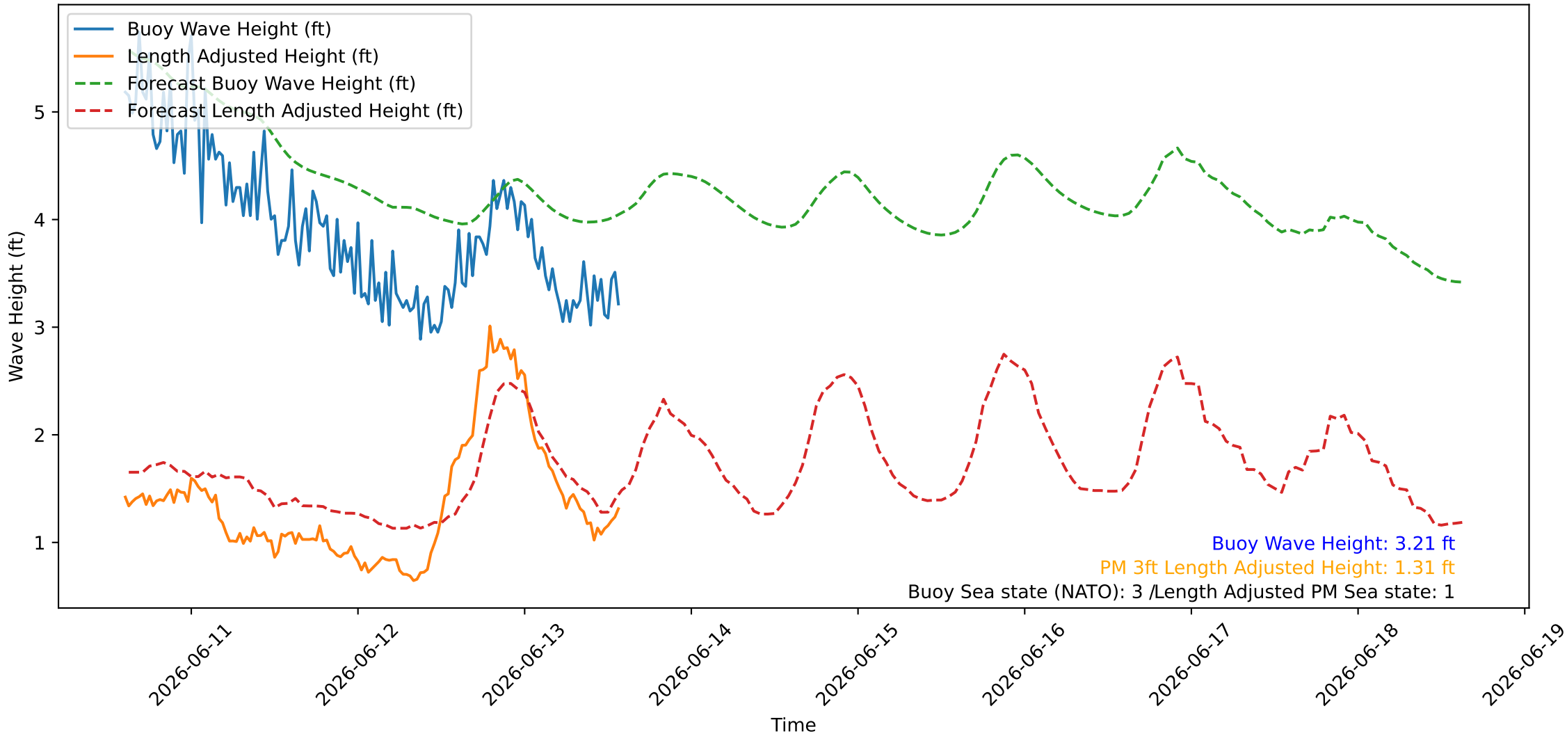
Wave Heights over Time for Green Beach at 2026-06-13 14:31:08
