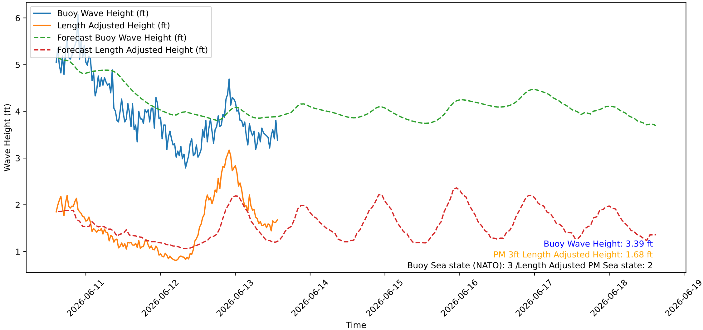
Wave Heights over Time for Oceanside Harbor at 2026-06-13 14:30:27
