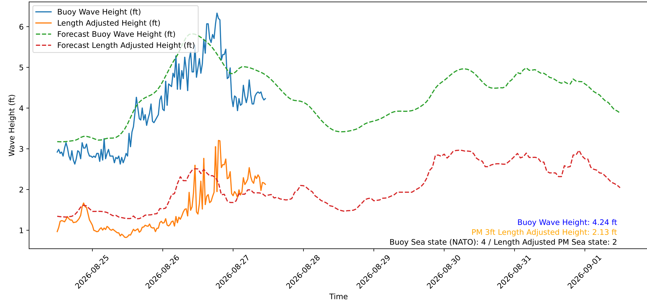
Wave Heights over Time for Green Beach at 2026-08-27 11:41:11
