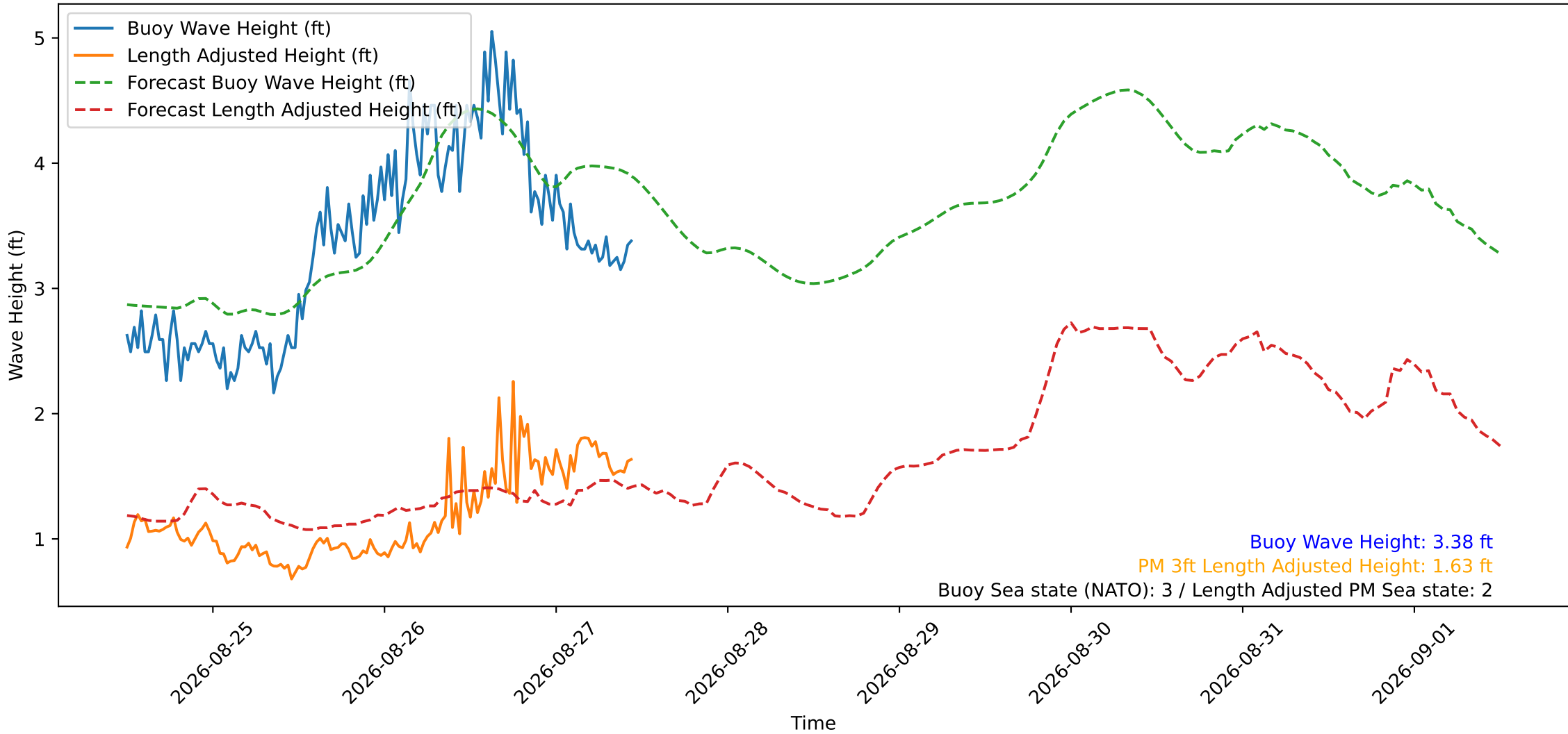
Wave Heights over Time for Red Beach at 2026-08-27 11:40:49
