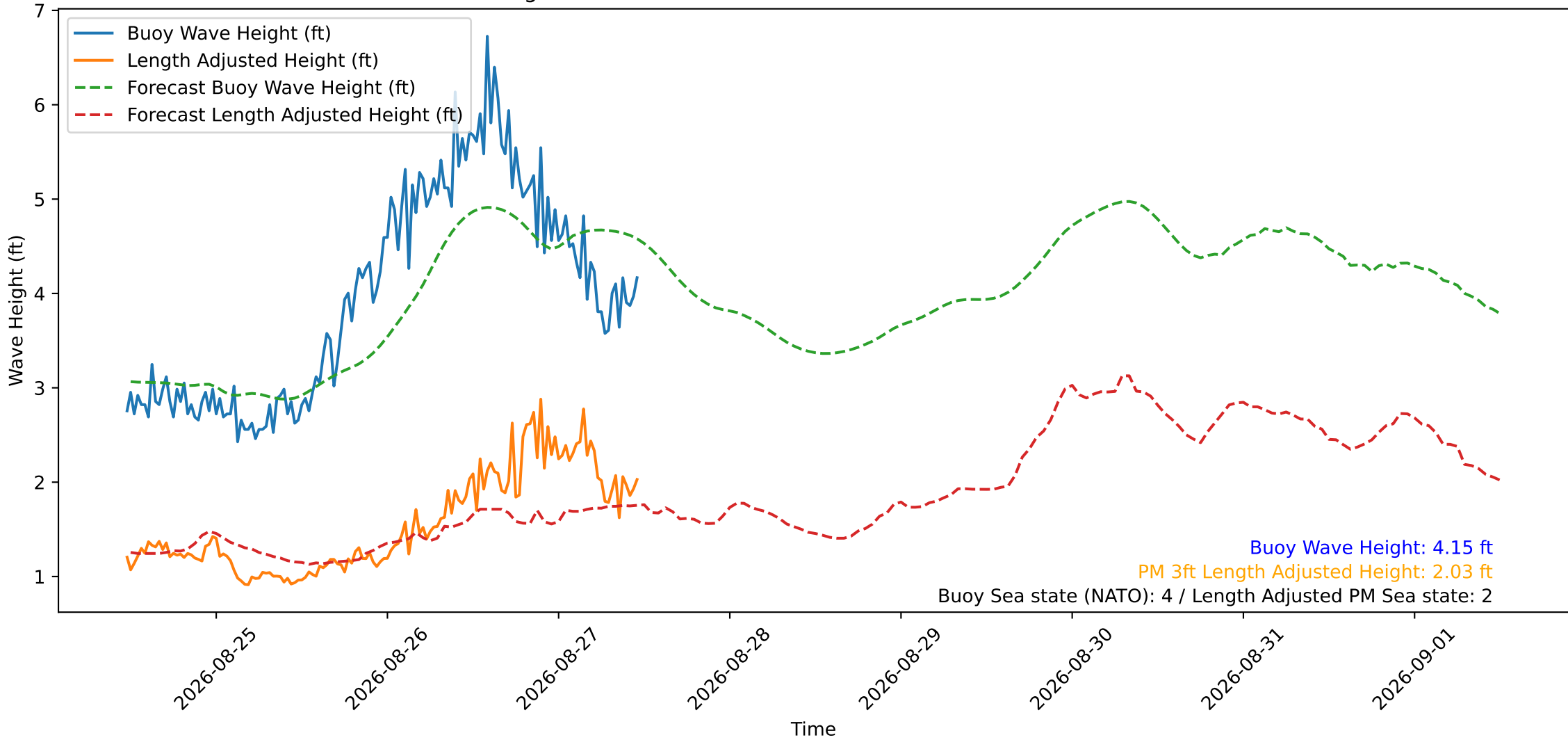
Wave Heights over Time for Oceanside Harbor at 2026-08-27 11:40:29
