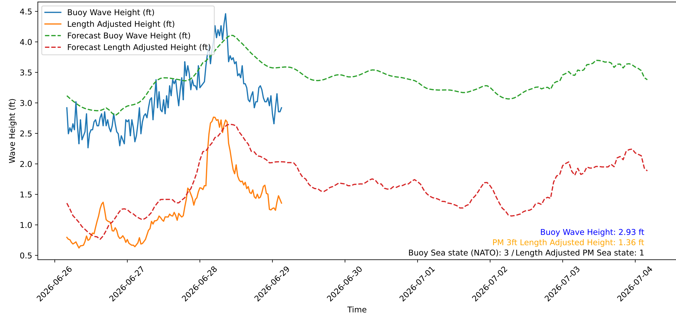
Wave Heights over Time for Red Beach at 2026-06-29 03:40:46
