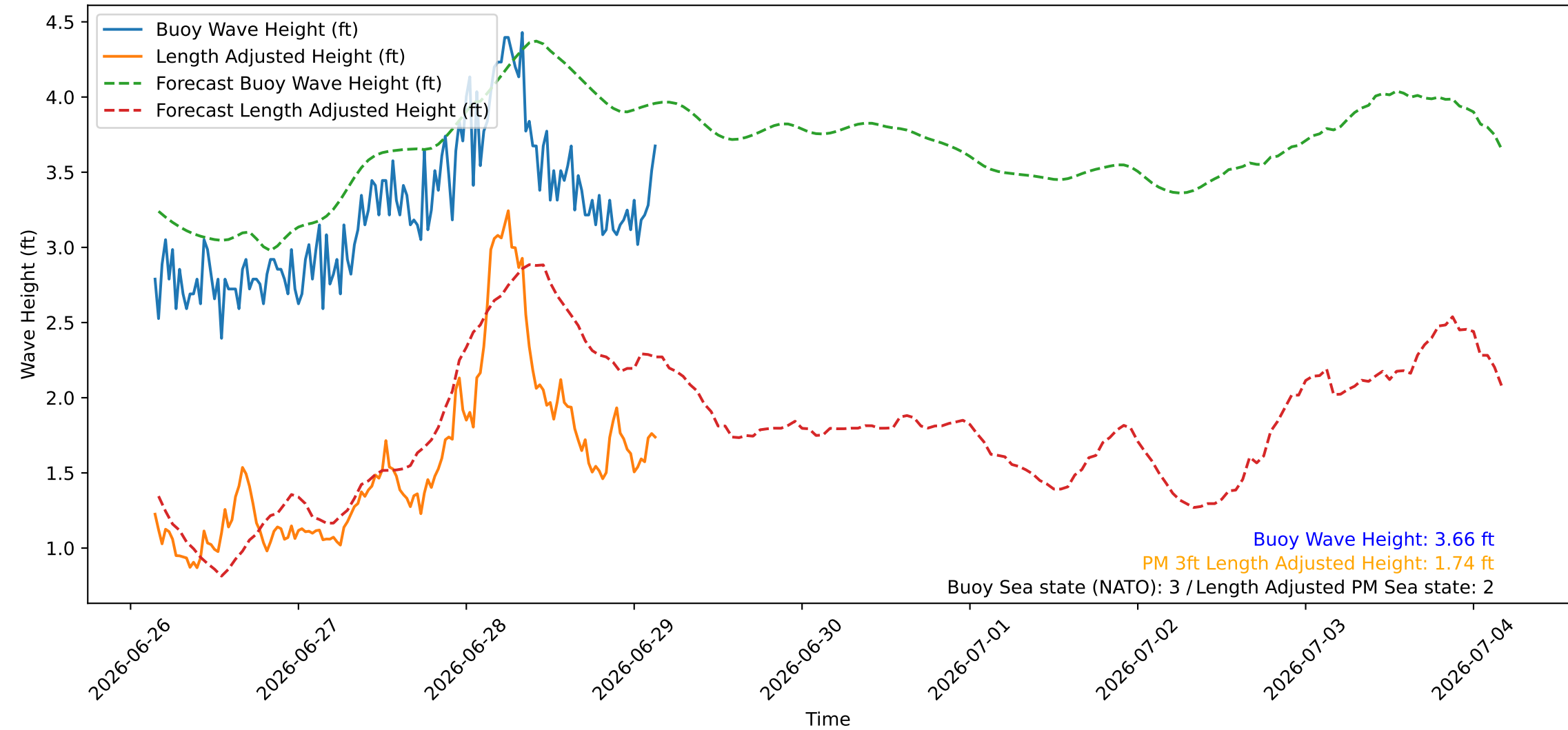
Wave Heights over Time for Oceanside Harbor at 2026-06-29 03:40:26
