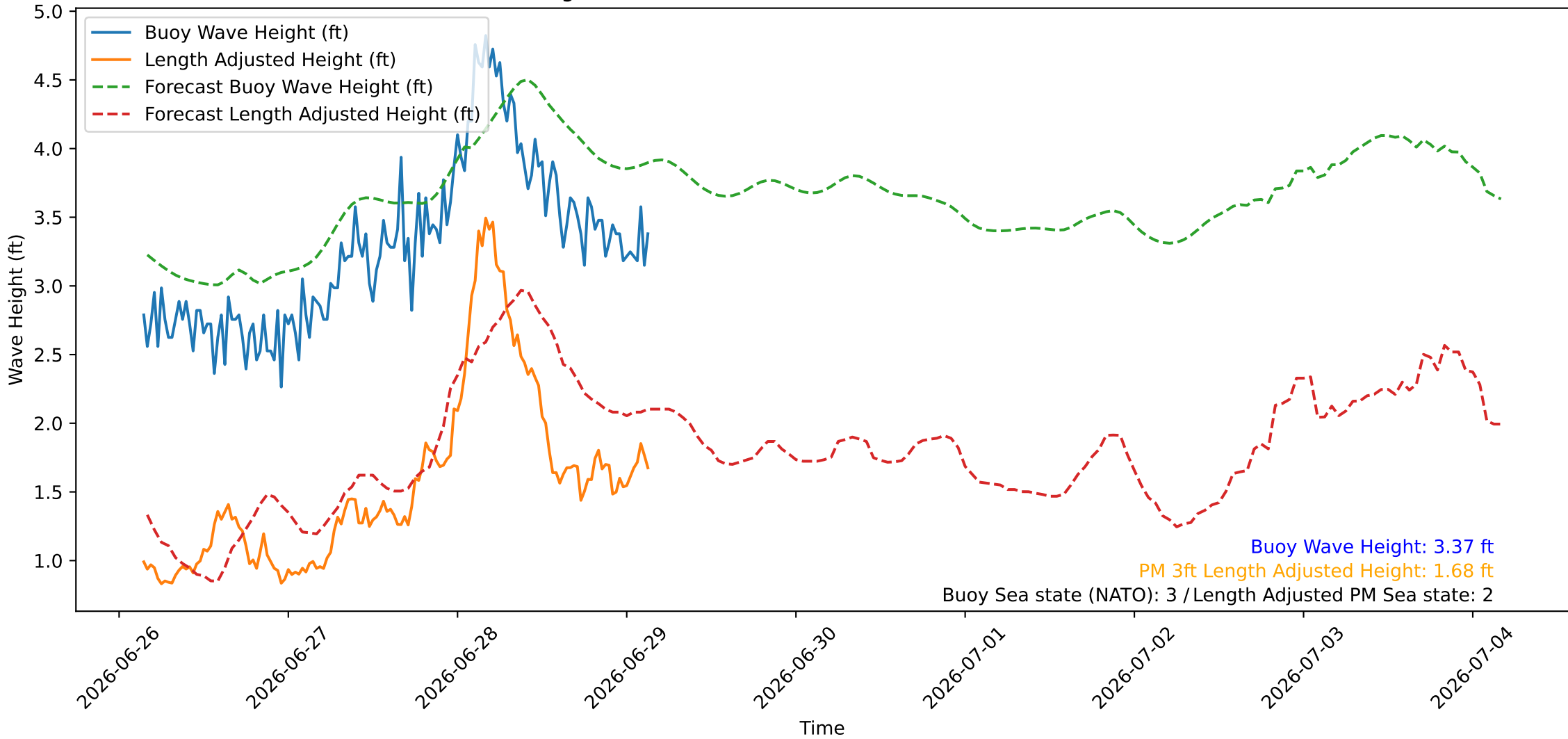
Wave Heights over Time for Green Beach at 2026-06-29 03:41:08
