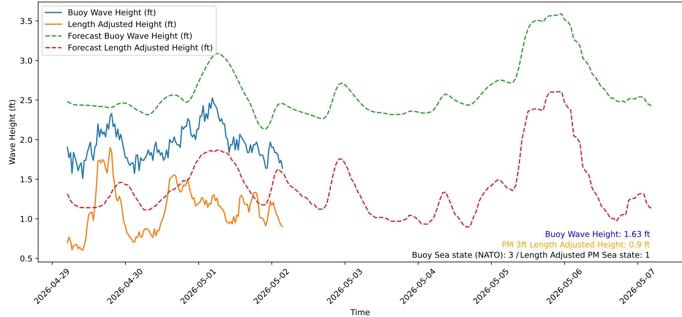
Wave Heights over Time for Red Beach at 2026-05-02 04:30:50
