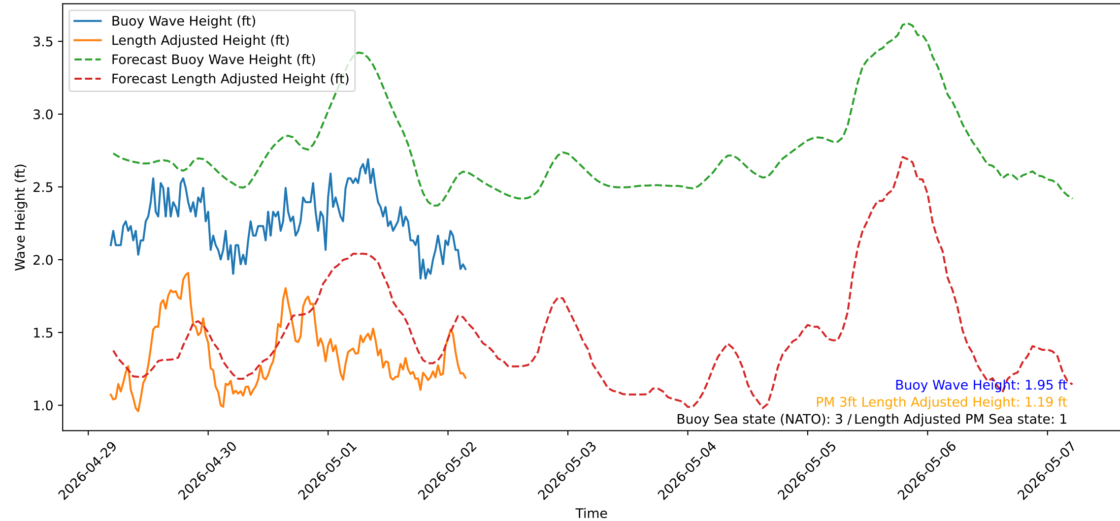
Wave Heights over Time for Oceanside Harbor at 2026-05-02 04:30:31
