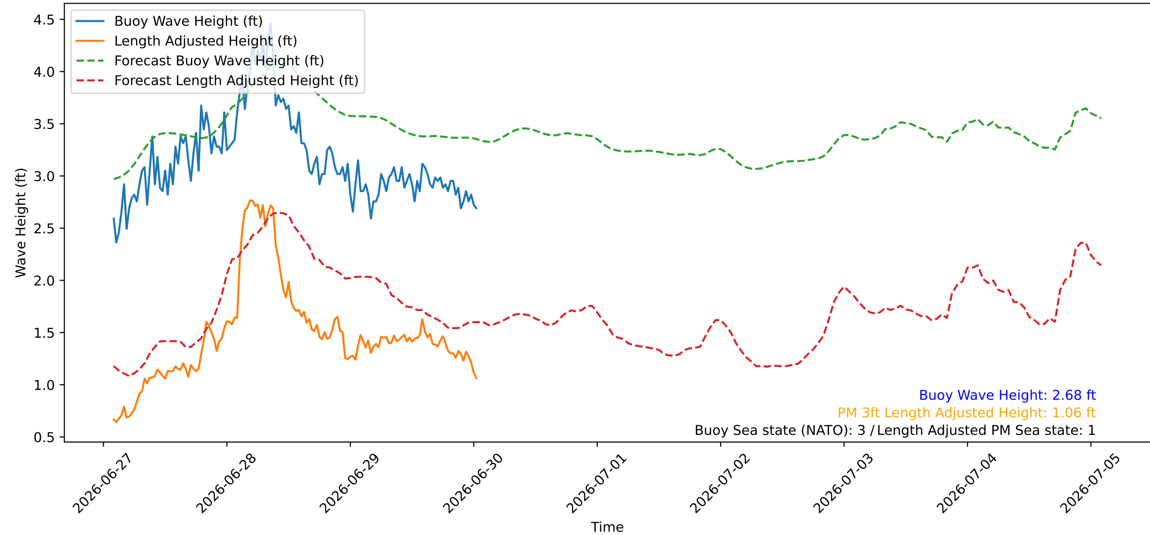
Wave Heights over Time for Red Beach at 2026-06-30 01:30:45
