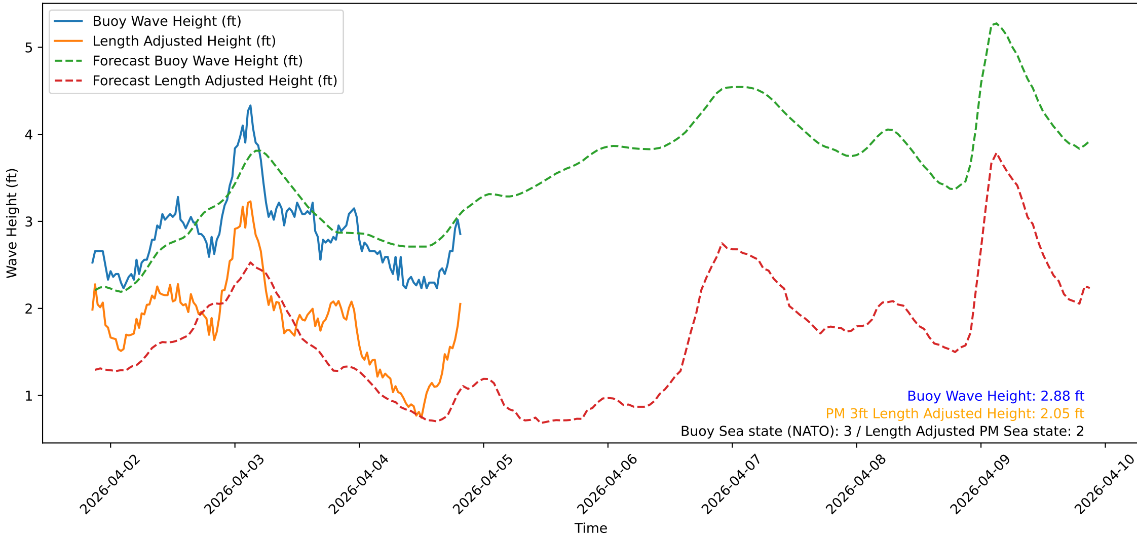
Wave Heights over Time for Green Beach at 2026-04-04 20:31:26
