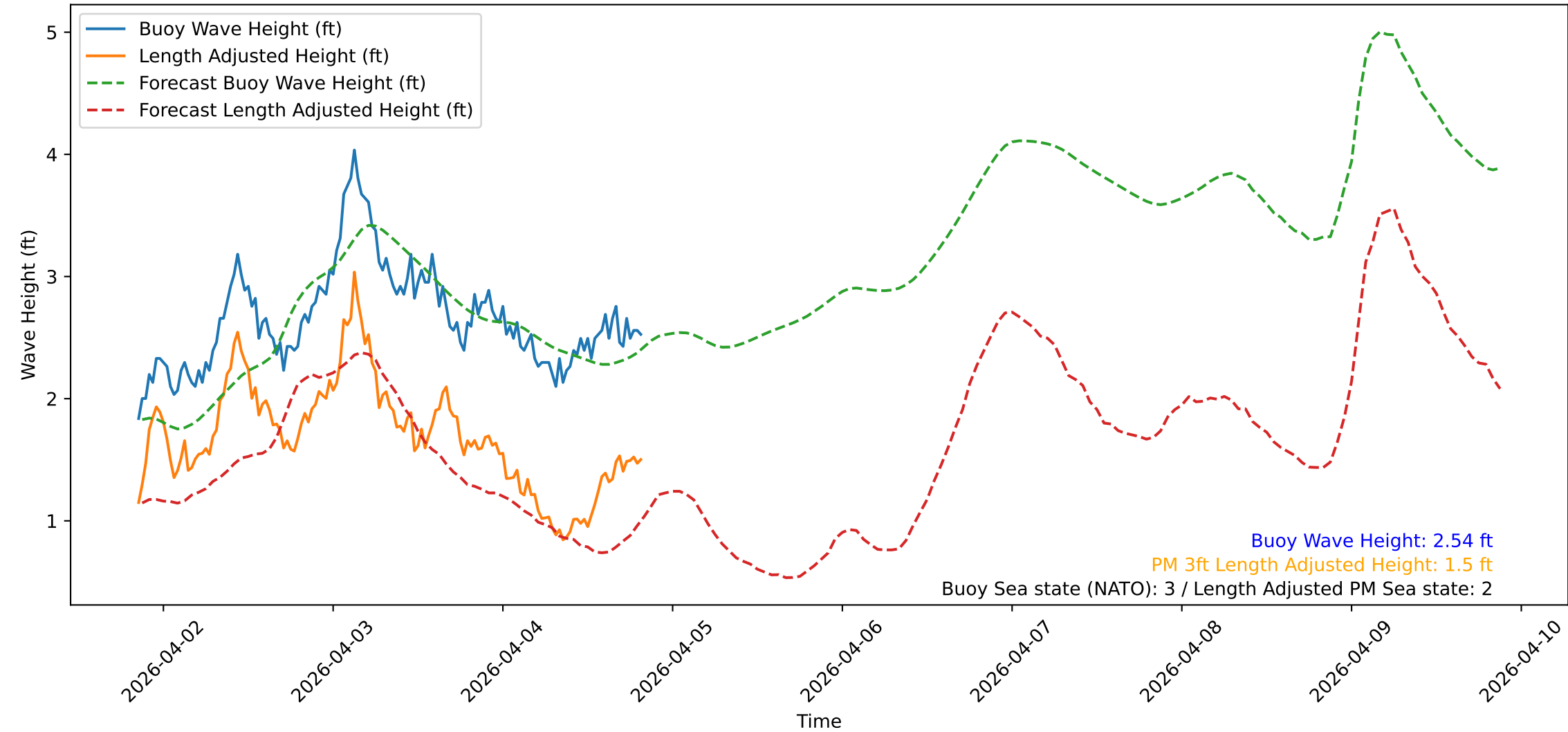
Wave Heights over Time for Oceanside Harbor at 2026-04-04 20:30:37
