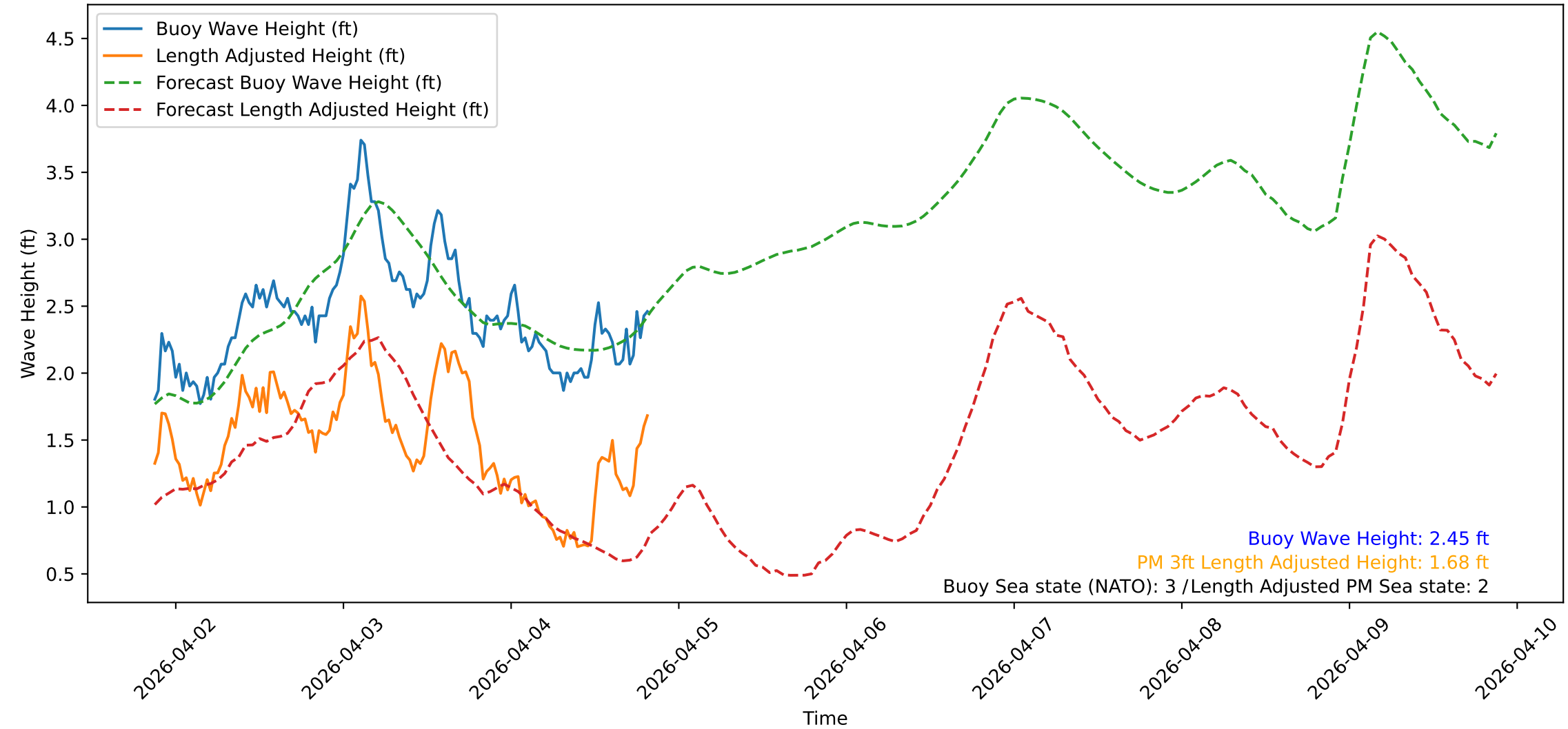
Wave Heights over Time for Red Beach at 2026-04-04 20:30:58
