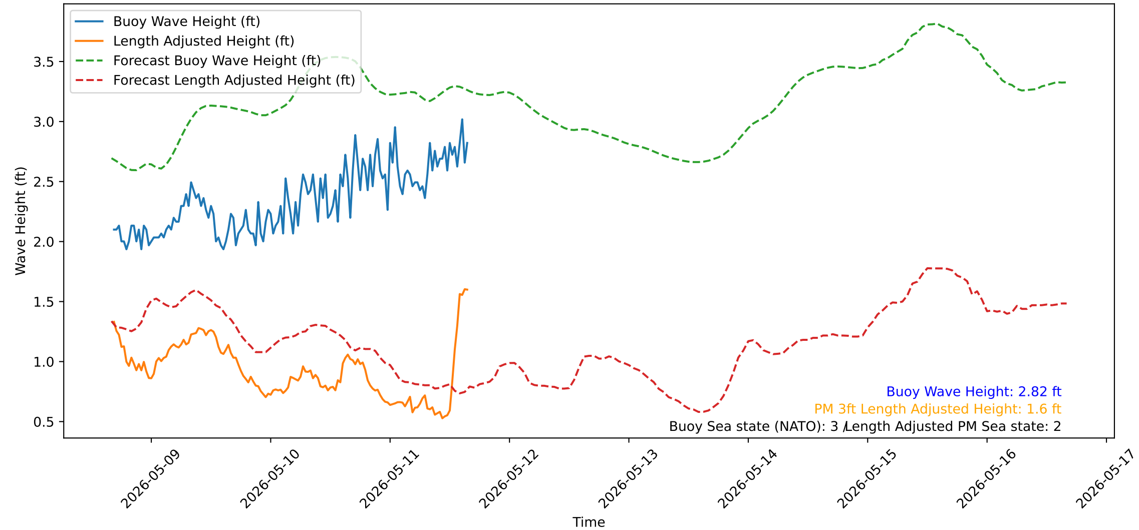
Wave Heights over Time for Red Beach at 2026-05-11 16:20:52
