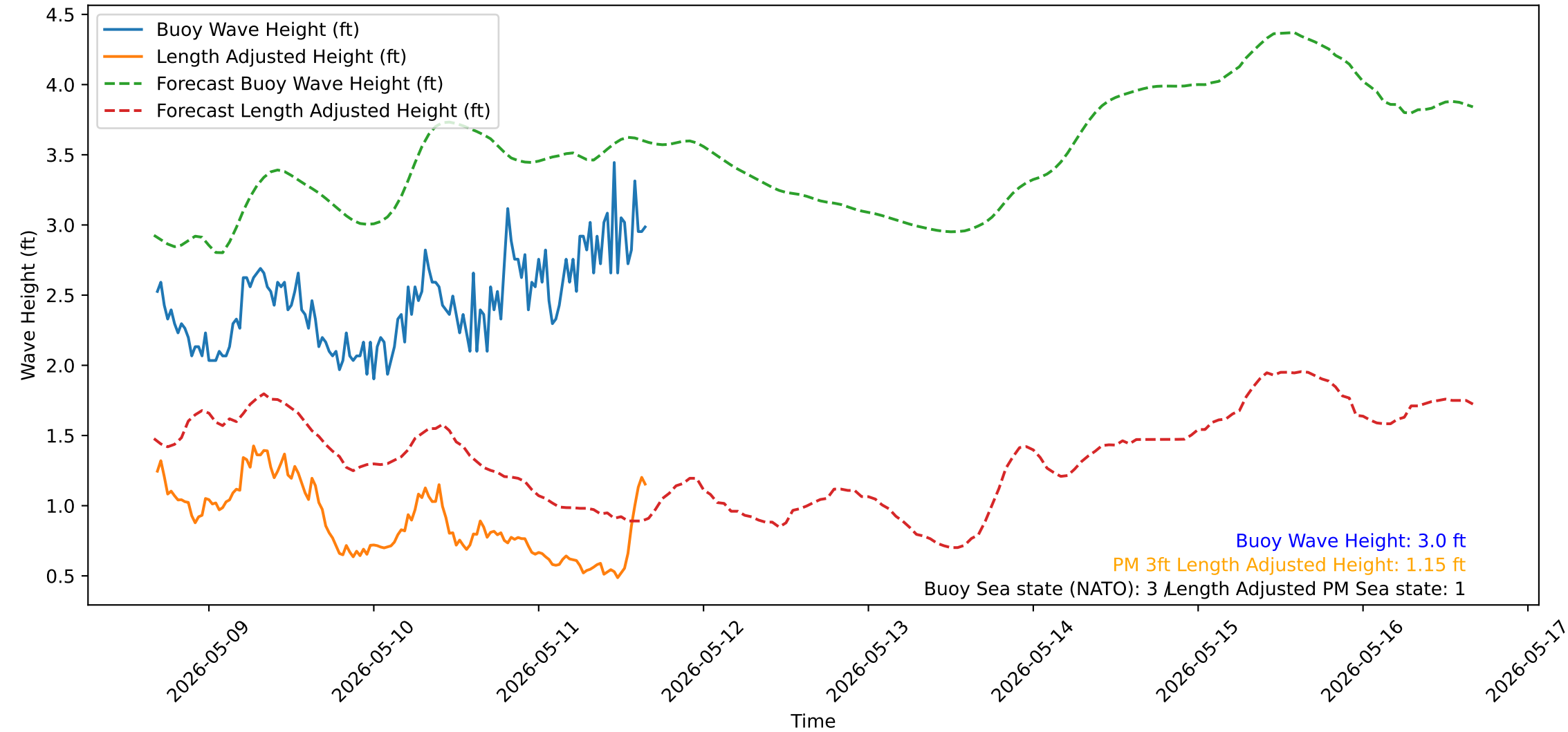
Wave Heights over Time for Green Beach at 2026-05-11 16:21:14
