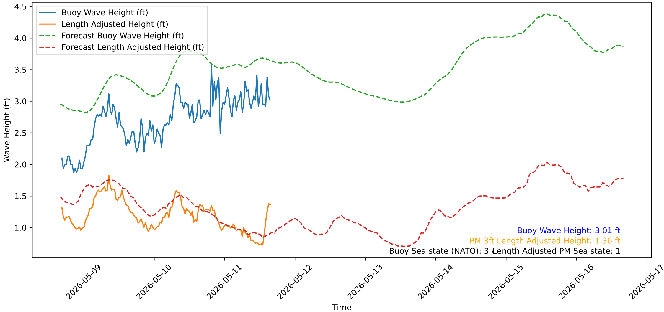
Wave Heights over Time for Oceanside Harbor at 2026-05-11 16:20:31
