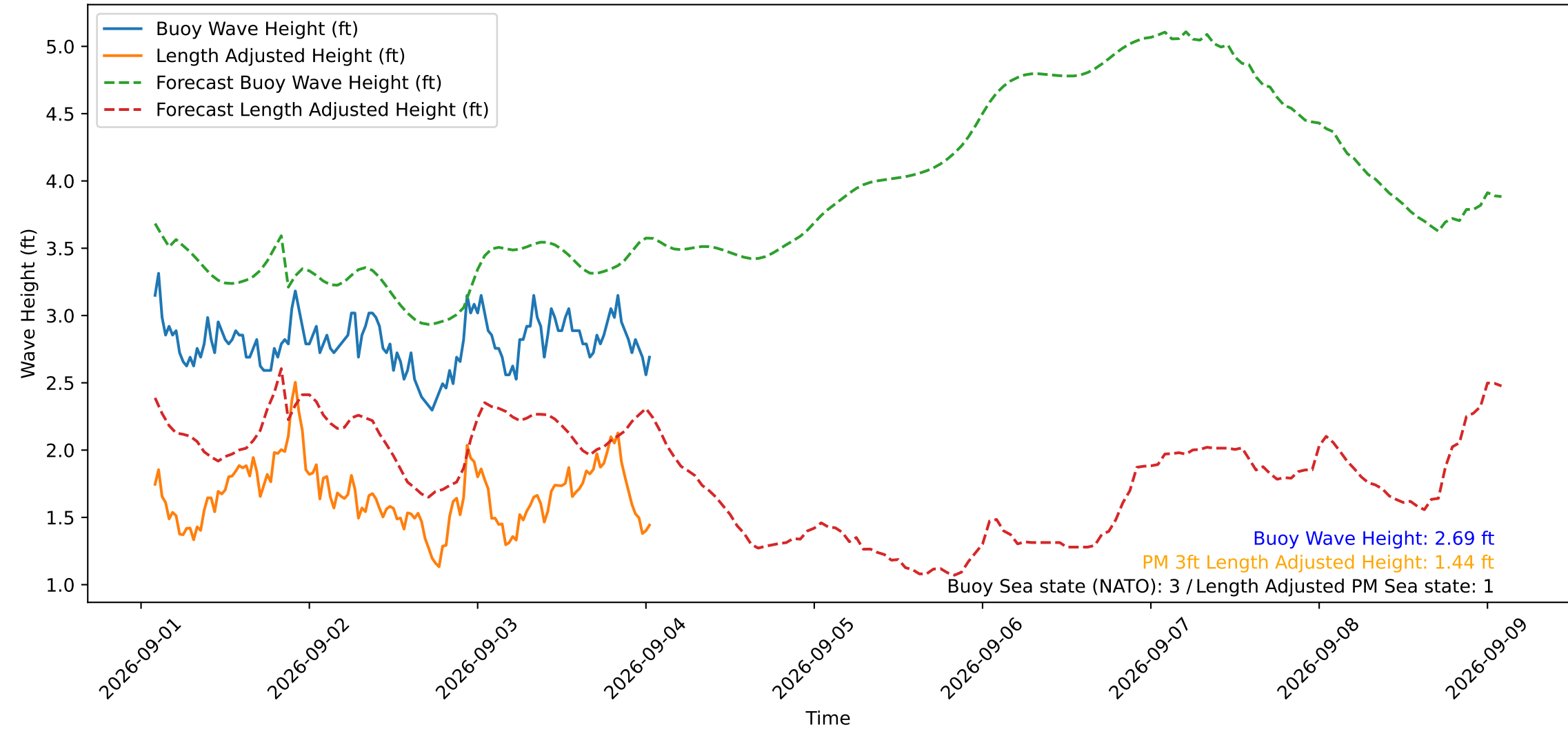
Wave Heights over Time for Red Beach at 2026-09-04 01:30:50
